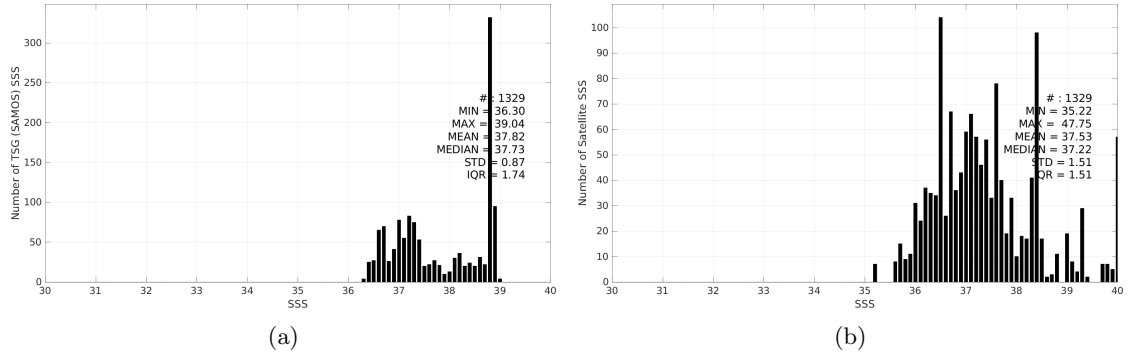
Figure 3: Histograms of SSS from TSG (SAMOS) (a) and SMOS SSS L3 v2 - 9-Days (BEC) (b) considering all match-up pairs per bins of 0.1 over the Mediterranean Sea Pi-MEP region and for the full satellite product period.
