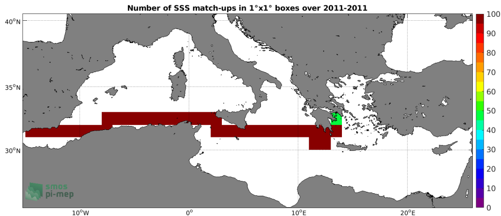
Figure 4: Number of SSS match-ups between TSG (SAMOS) SSS and the SMOS SSS L3 v2 - 9-Days (BEC) SSS product for the Mediterranean Sea Pi-MEP region over 1°x1° boxes and for the full satellite product period.
