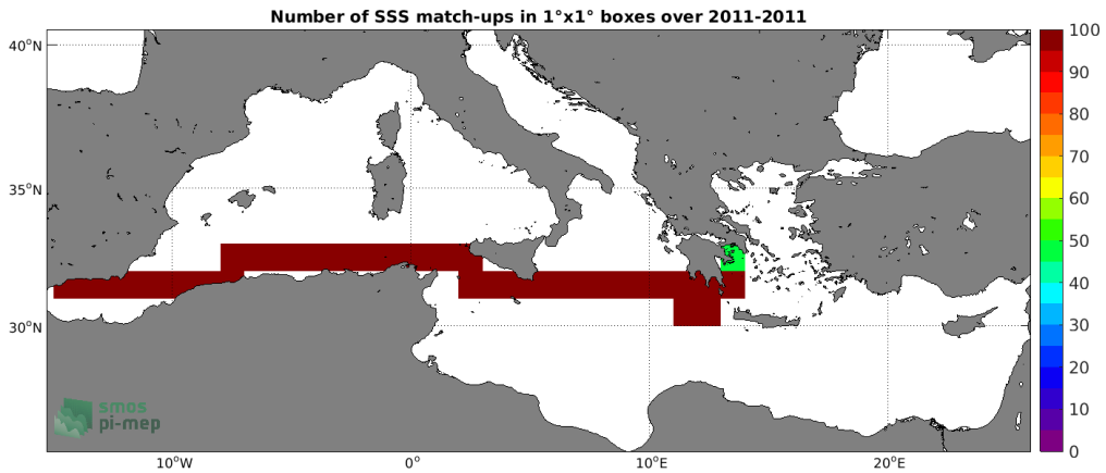
Figure 4: Number of SSS match-ups between TSG (SAMOS) SSS and the SMOS SSS L3 v2 - 9-Days (BEC) SSS product for the Mediterranean Sea Pi-MEP region over 1^\circ \times 1^\circ boxes and for the full satellite product period.
