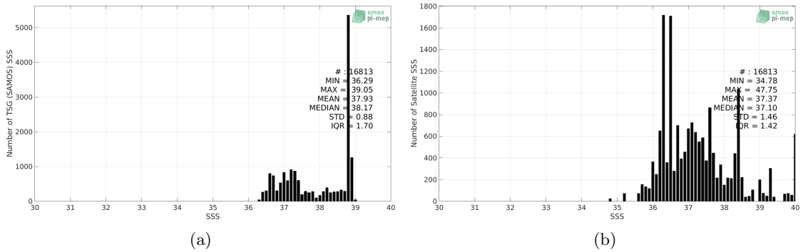
Figure 2: Histograms of SSS from TSG (SAMOS) (a) and SMOS SSS L3 v2 - 9-Days (BEC) (b) considering all match-up pairs per bins of 0.1 over the Mediterranean Sea Pi-MEP region and for the full satellite product period.
