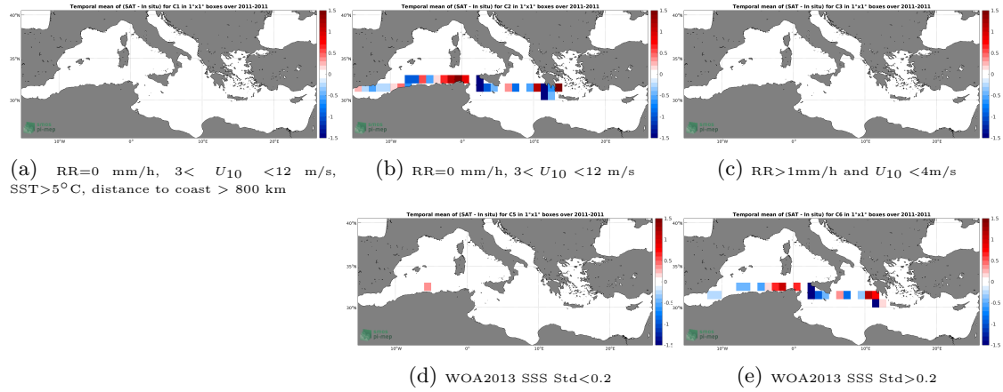
Figure 12: Temporal mean gridded over spatial boxes of size 1^{\circ}\times 1^{\circ} of \Delta\text{SSS} (SMOS SSS L3 v2 - 9-Days (BEC) - TSG (SAMOS)) for 5 different subdatasets corresponding to:RR=0 mm/h, 3 < U_{10} < 12 m/s, SST > 5^{\circ}\text{C} , distance to coast > 800 km (a), RR=0 mm/h, 3 < U_{10} < 12 m/s (b), RR > 1 mm/h and U_{10} < 4 m/s (c), WOA2013 SSS Std < 0.2 (d), WOA2013 SSS Std > 0.2 (e).
