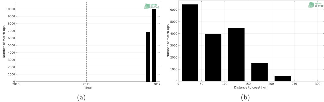
Figure 1: Number of match-ups between TSG (SAMOS) and SMOS SSS L3 v2 - 9-Days (BEC) SSS as a function of time (a) and as function of the distance to coast (b) over the Mediterranean Sea Pi-MEP region and for the full satellite product period.
