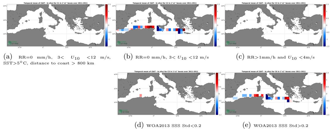
Figure 12: Temporal mean gridded over spatial boxes of size 1^{\circ}\times 1^{\circ} of \Delta\text{SSS} (SMOS L3 v2 - 9-Days (BEC) - TSG (SAMOS)) for 5 different subdatasets corresponding to:RR=0 mm/h, 3 < U_{10} < 12 m/s, SST >5^{\circ}\text{C} , distance to coast > 800 km (a), RR=0 mm/h, 3 < U_{10} < 12 m/s (b), RR >1 mm/h and U_{10} < 4 m/s (c), WOA2013 SSS Std <0.2 (d), WOA2013 SSS Std >0.2 (e).
