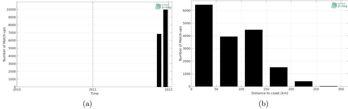
Figure 1: Number of match-ups between TSG (SAMOS) and SMOS L3 v2 - 9-Days (BEC) SSS as a function of time (a) and as function of the distance to coast (b) over the Mediterranean Sea Pi-MEP region and for the full satellite product period.
