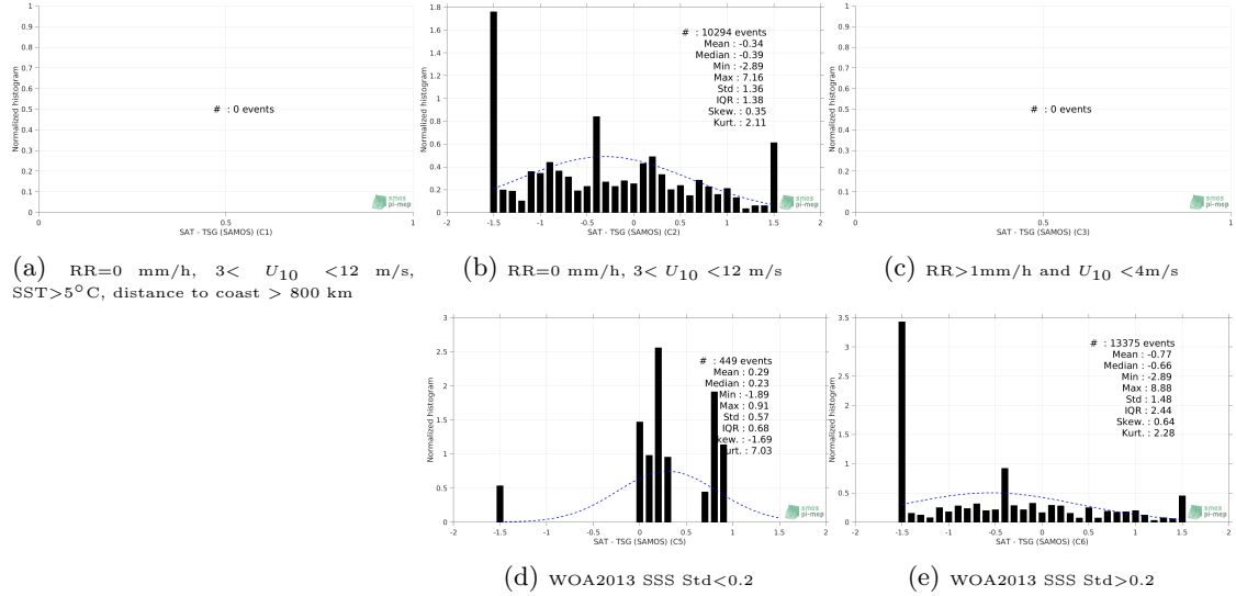
Figure 13: Normalized histogram of \Delta SSS (SMOS L3 v2 - 9-Days (BEC) - TSG (SAMOS)) for 5 different subdatasets corresponding to: RR=0 mm/h, 3 < U_{10} < 12 m/s, SST > 5°C, distance to coast > 800 km (a), RR=0 mm/h, 3 < U_{10} < 12 m/s (b), RR > 1mm/h and U_{10} < 4 m/s (c), WOA2013 SSS Std < 0.2 (d), WOA2013 SSS Std > 0.2 (e).
