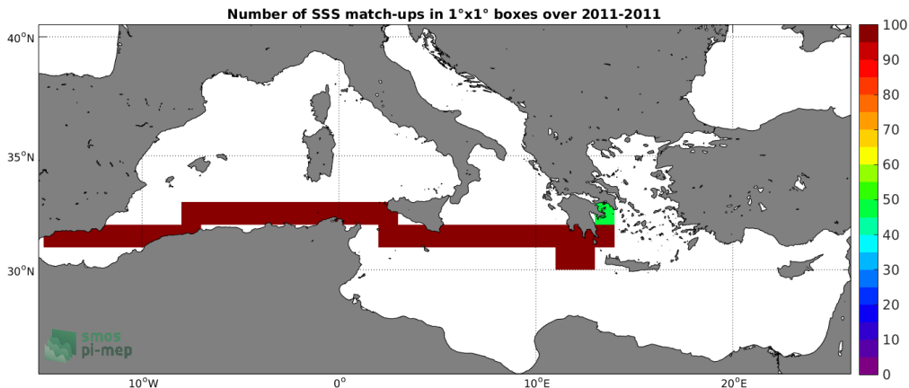
Figure 4: Number of SSS match-ups between TSG (SAMOS) SSS and the SMOS L3 v2 - 9-Days (BEC) SSS product for the Mediterranean Sea Pi-MEP region over 1^\circ \times 1^\circ boxes and for the full satellite product period.
