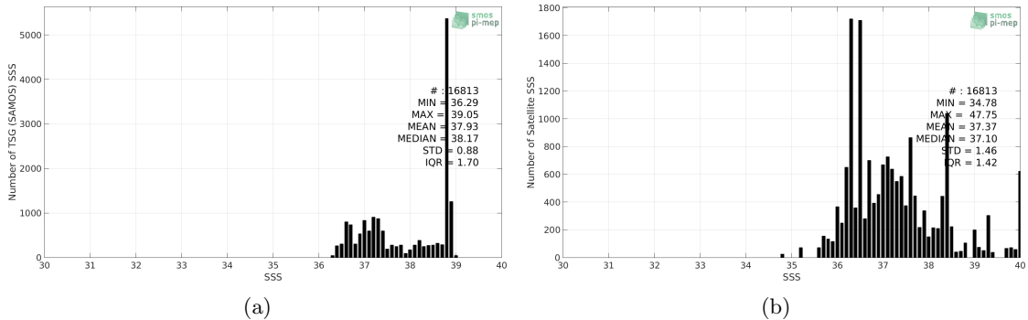
Figure 2: Histograms of SSS from TSG (SAMOS) (a) and SMOS L3 v2 - 9-Days (BEC) (b) considering all match-up pairs per bins of 0.1 over the Mediterranean Sea Pi-MEP region and for the full satellite product period.
