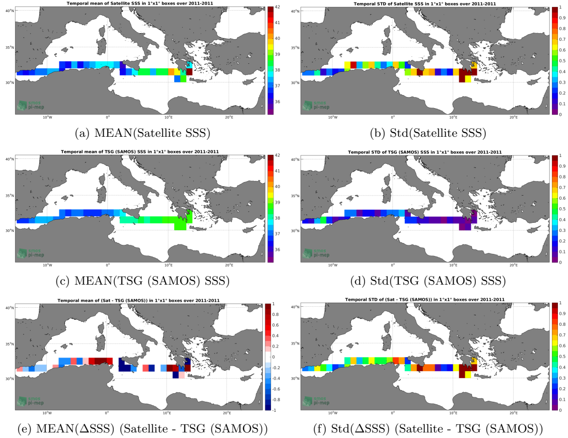
Figure 6: Temporal mean (left) and Std (right) of SSS from SMOS L3 v2 - 9-Days (BEC) (top), TSG (SAMOS) (middle), and of \Delta SSS (Satellite - TSG (SAMOS)). Only match-up pairs are used to generate these maps.
