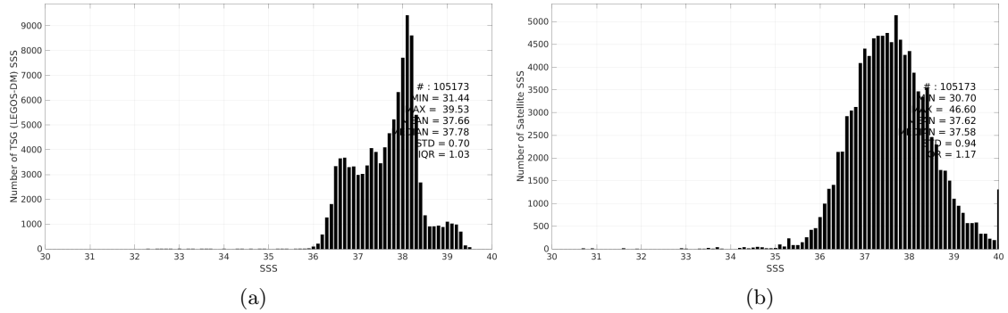
Figure 3: Histograms of SSS from TSG (LEGOS-DM) (a) and SMOS SSS L3 v2 - 9-Days (BEC) (b) considering all match-up pairs per bins of 0.1 over the Mediterranean Sea Pi-MEP region and for the full satellite product period.
