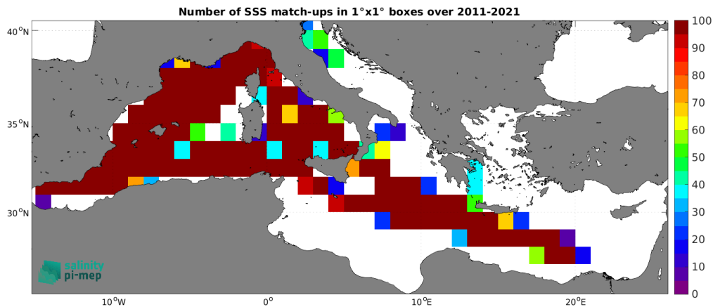
Figure 5: Number of SSS match-ups between TSG (LEGOS-DM) SSS and the SMOS SSS L3 v2 - 9-Days (BEC) SSS product for the Mediterranean Sea Pi-MEP region over 1^\circ \times 1^\circ boxes and for the full satellite product period.
