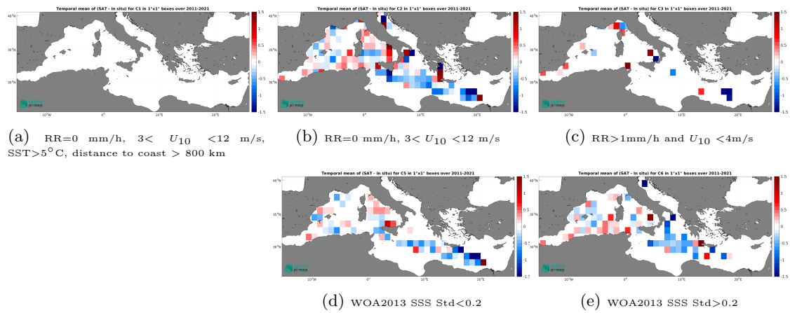
Figure 14: Temporal mean gridded over spatial boxes of size 1^\circ \times 1^\circ of \Delta SSS (SMOS SSS L3 v2 - 9-Days (BEC) - TSG (LEGOS-DM)) for 5 different subdatasets corresponding to:RR=0 mm/h, 3 < U_{10} < 12 m/s, SST>5°C, distance to coast > 800 km (a), RR=0 mm/h, 3 < U_{10} < 12 m/s (b), RR>1mm/h and U_{10} < 4 m/s (c), WOA2013 SSS Std<0.2 (d), WOA2013 SSS Std>0.2 (e).
