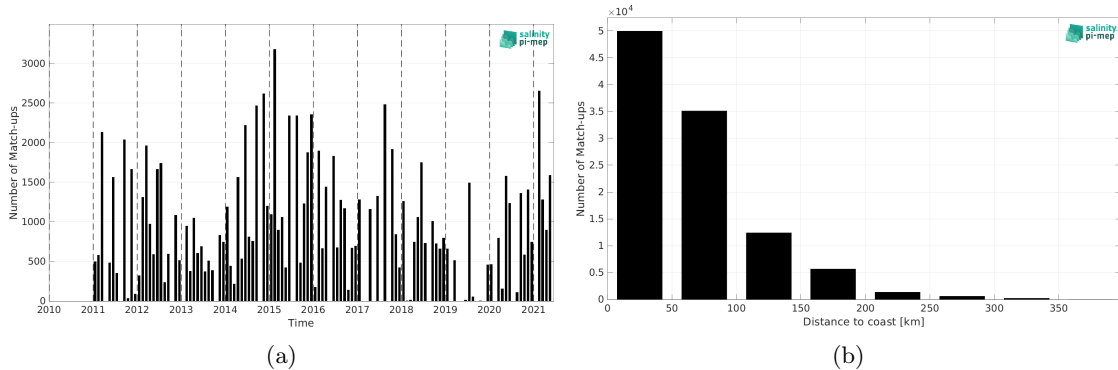
Figure 2: Number of match-ups between TSG (LEGOS-DM) and SMOS SSS L3 v2 - 9-Days (BEC) SSS as a function of time (a) and as function of the distance to coast (b) over the Mediterranean Sea Pi-MEP region and for the full satellite product period.
