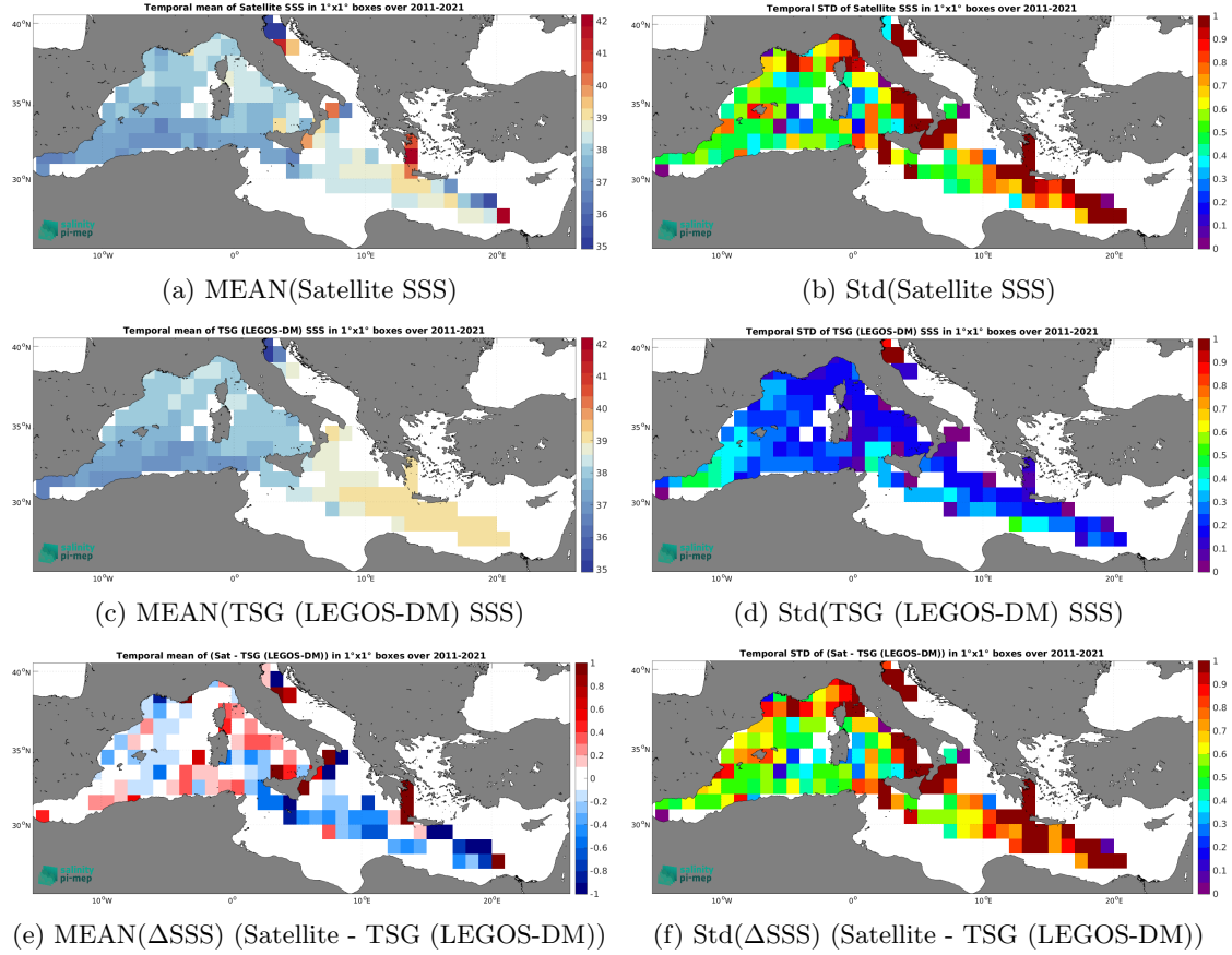
Figure 7: Temporal mean (left) and Std (right) of SSS from SMOS SSS L3 v2 - 9-Days (BEC) (top), TSG (LEGOS-DM) (middle), and of \Delta\text{SSS} (Satellite - TSG (LEGOS-DM)). Only match-up pairs are used to generate these maps.
