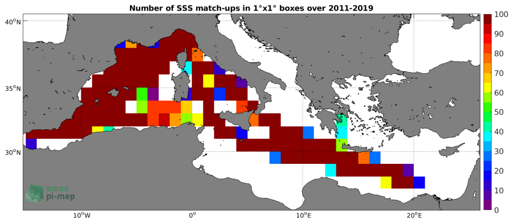
Figure 4: Number of SSS match-ups between TSG (LEGOS-DM) SSS and the SMOS SSS L3 v2 - 9-Days (BEC) SSS product for the Mediterranean Sea Pi-MEP region over 1°x1° boxes and for the full satellite product period.
