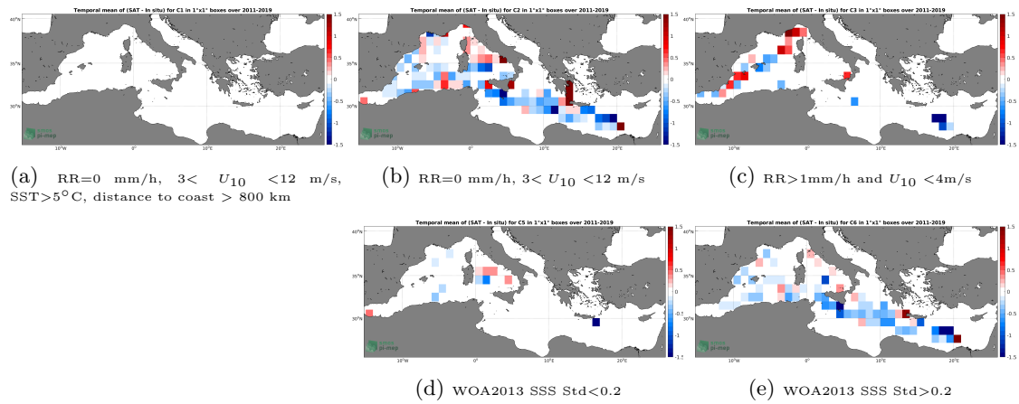
Figure 12: Temporal mean gridded over spatial boxes of size 1^\circ \times 1^\circ of \Delta SSS (SMOS SSS L3 v2 - 9-Days (BEC) - TSG (LEGOS-DM)) for 5 different subdatasets corresponding to:RR=0 mm/h, 3 < U_{10} < 12 m/s, SST >5^\circ C, distance to coast > 800 km (a), RR=0 mm/h, 3 < U_{10} < 12 m/s (b), RR >1 mm/h and U_{10} < 4 m/s (c), WOA2013 SSS Std <0.2 (d), WOA2013 SSS Std >0.2 (e).
