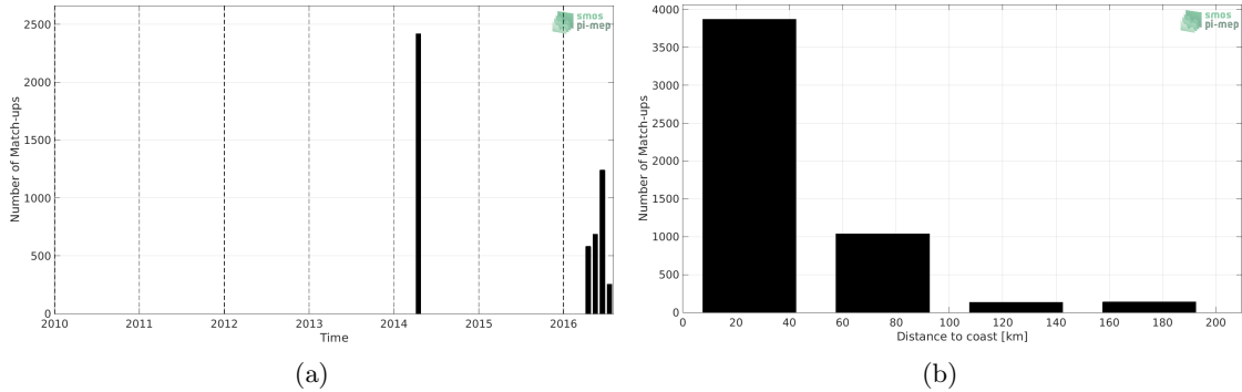
Figure 1: Number of match-ups between TSG (GOSUD-Sailing-ship) and SMOS SSS L3 v2 - 9-Days (BEC) SSS as a function of time (a) and as function of the distance to coast (b) over the Mediterranean Sea Pi-MEP region and for the full satellite product period.
