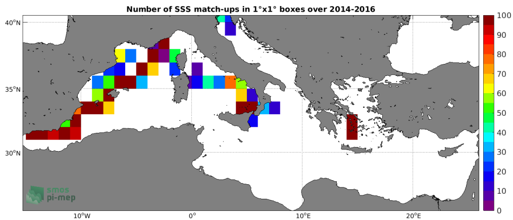
Figure 4: Number of SSS match-ups between TSG (GOSUD-Sailing-ship) SSS and the SMOS SSS L3 v2 - 9-Days (BEC) SSS product for the Mediterranean Sea Pi-MEP region over 1°x1° boxes and for the full satellite product period.
