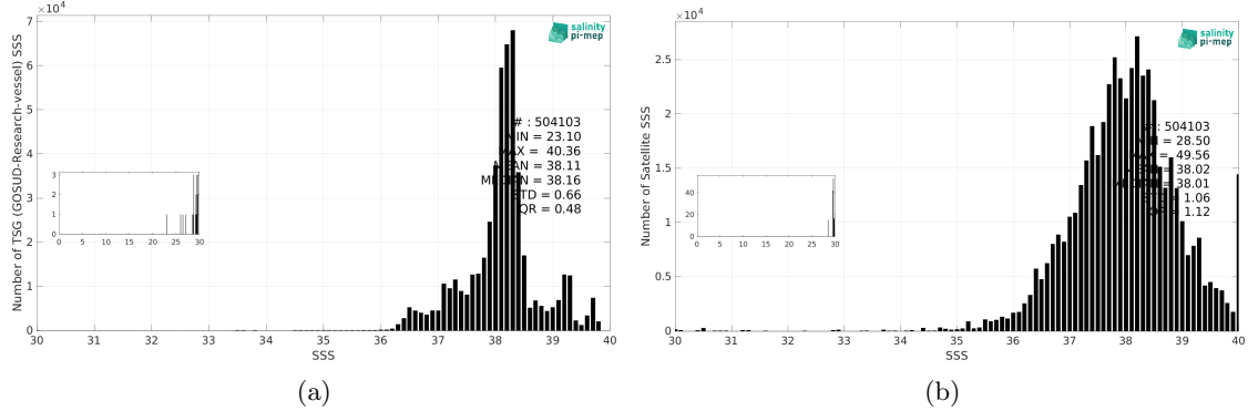
Figure 3: Histograms of SSS from TSG (GOSUD-Research-vessel) (a) and SMOS SSS L3 v2 - 9-Days (BEC) (b) considering all match-up pairs per bins of 0.1 over the Mediterranean Sea Pi-MEP region and for the full satellite product period.
