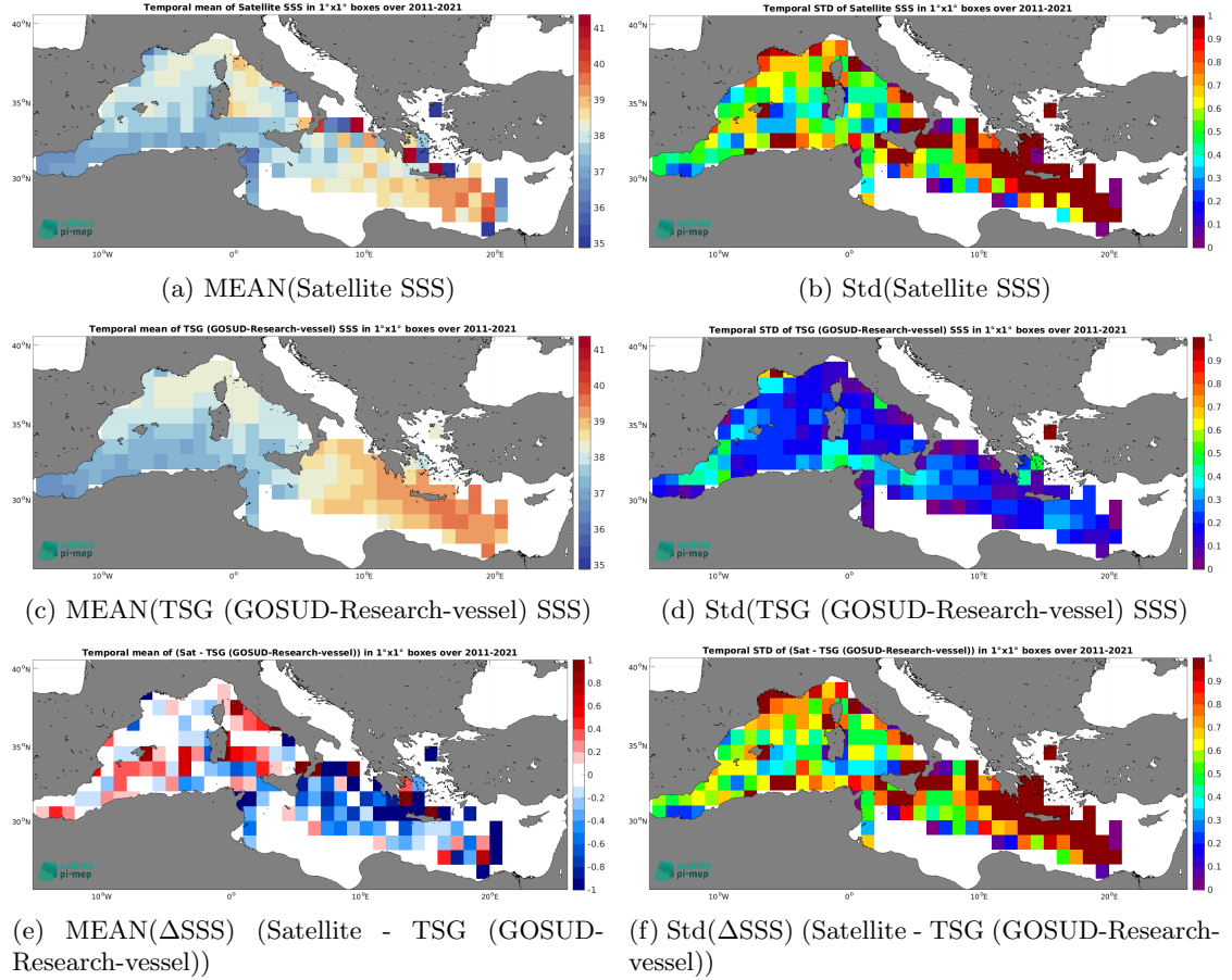
Figure 7: Temporal mean (left) and Std (right) of SSS from SMOS SSS L3 v2 - 9-Days (BEC) (top), TSG (GOSUD-Research-vessel) (middle), and of \Delta\text{SSS} (Satellite - TSG (GOSUD-Research-vessel)). Only match-up pairs are used to generate these maps.
