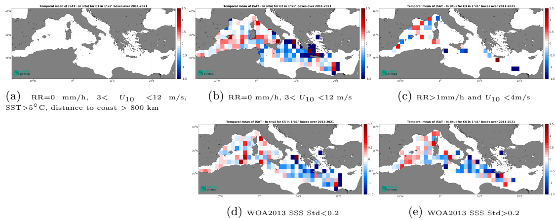
Figure 14: Temporal mean gridded over spatial boxes of size 1^\circ \times 1^\circ of \Delta\text{SSS} (SMOS SSS L3 v2 - 9-Days (BEC) - TSG (GOSUD-Research-vessel)) for 5 different subdatasets corresponding to:RR=0 mm/h, 3 < U_{10} < 12 m/s, SST>5°C, distance to coast > 800 km (a), RR=0 mm/h, 3 < U_{10} < 12 m/s (b), RR>1mm/h and U_{10} < 4 m/s (c), WOA2013 SSS Std<0.2 (d), WOA2013 SSS Std>0.2 (e).
