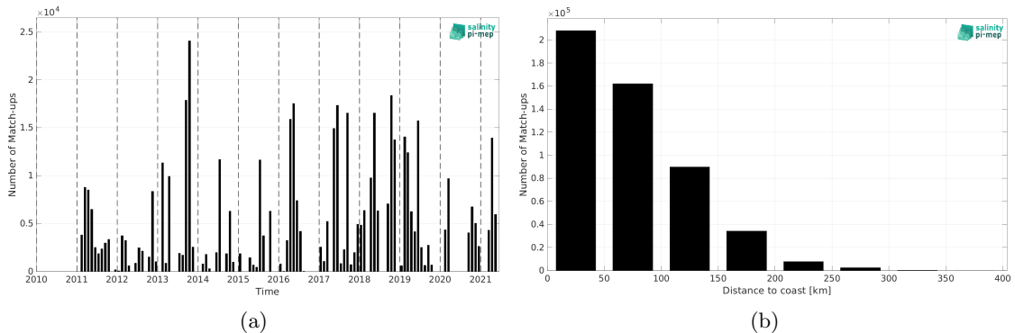
Figure 2: Number of match-ups between TSG (GOSUD-Research-vessel) and SMOS SSS L3 v2 - 9-Days (BEC) SSS as a function of time (a) and as function of the distance to coast (b) over the Mediterranean Sea Pi-MEP region and for the full satellite product period.
