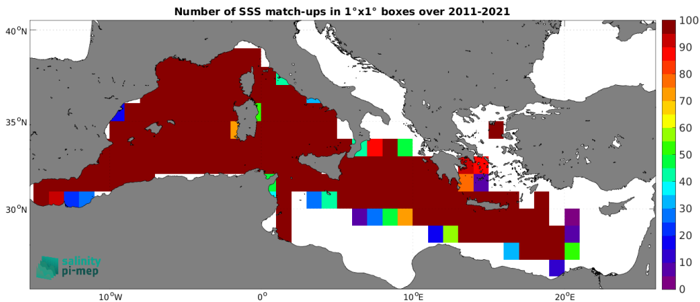
Figure 5: Number of SSS match-ups between TSG (GOSUD-Research-vessel) SSS and the SMOS SSS L3 v2 - 9-Days (BEC) SSS product for the Mediterranean Sea Pi-MEP region over 1^\circ \times 1^\circ boxes and for the full satellite product period.
