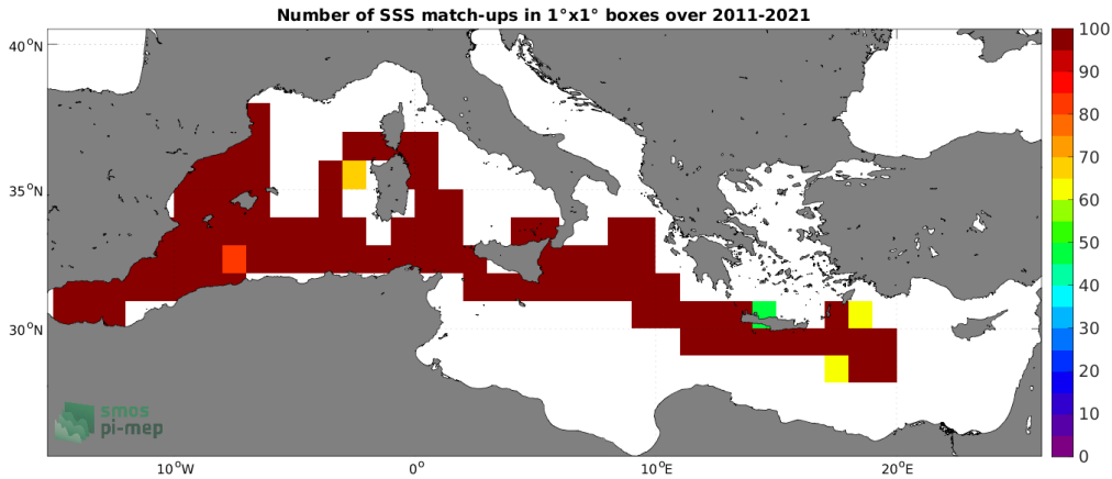
Figure 4: Number of SSS match-ups between TSG (CSIC-UTM) SSS and the SMOS SSS L3 v2 - 9-Days (BEC) SSS product for the Mediterranean Sea Pi-MEP region over 1^\circ \times 1^\circ boxes and for the full satellite product period.
