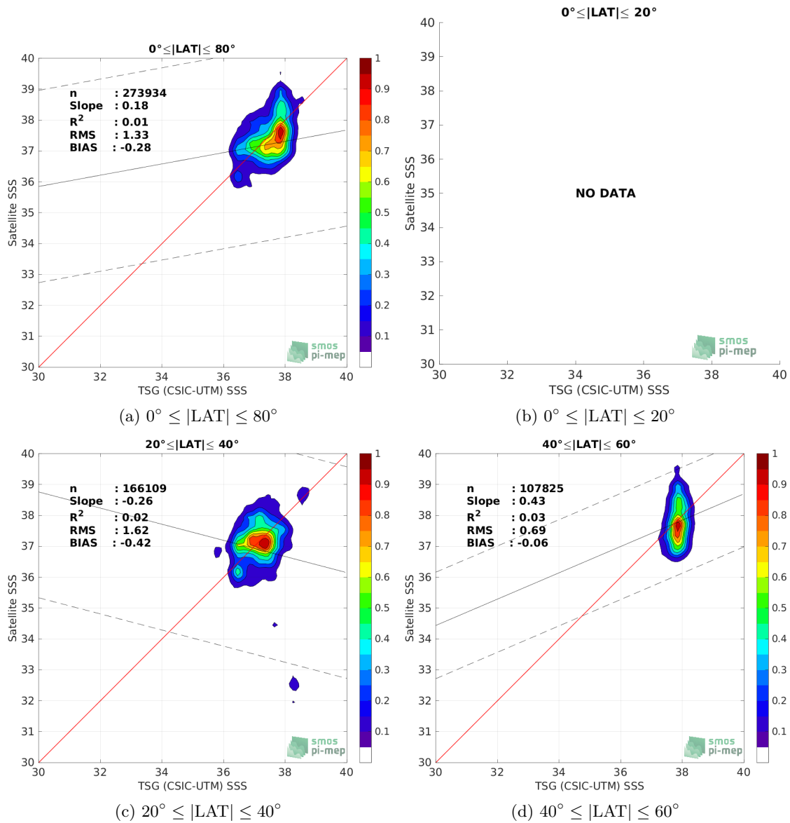
Figure 9: Contour maps of the concentration of SMOS SSS L3 v2 - 9-Days (BEC) SSS (y-axis) versus TSG (CSIC-UTM) SSS (x-axis) at match-up pairs for different latitude bands. For each plot, the red line shows x=y . The black thin and dashed lines indicate a linear fit through the data cloud and the \pm 95\% confidence levels, respectively. The number match-up pairs n , the slope and R^2 coefficient of the linear fit, the root mean square (RMS) and the mean bias between satellite and in situ data are indicated for each latitude band in each plots.
