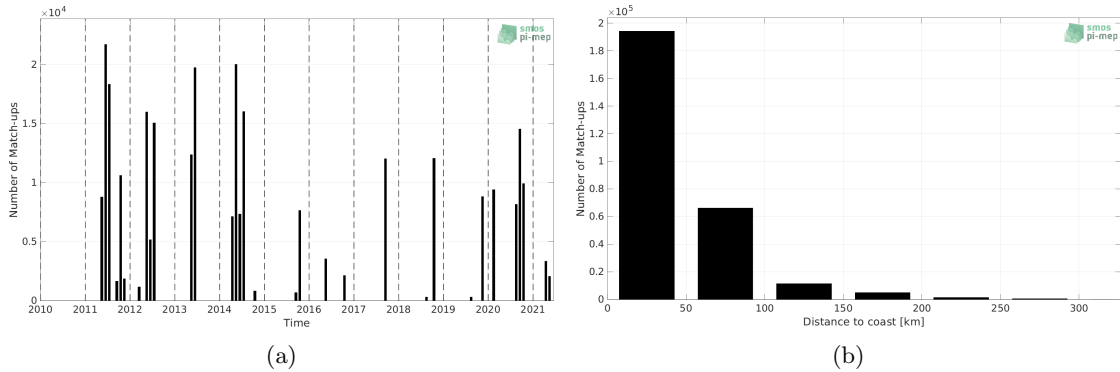
Figure 1: Number of match-ups between TSG (CSIC-UTM) and SMOS SSS L3 v2 - 9-Days (BEC) SSS as a function of time (a) and as function of the distance to coast (b) over the Mediterranean Sea Pi-MEP region and for the full satellite product period.
