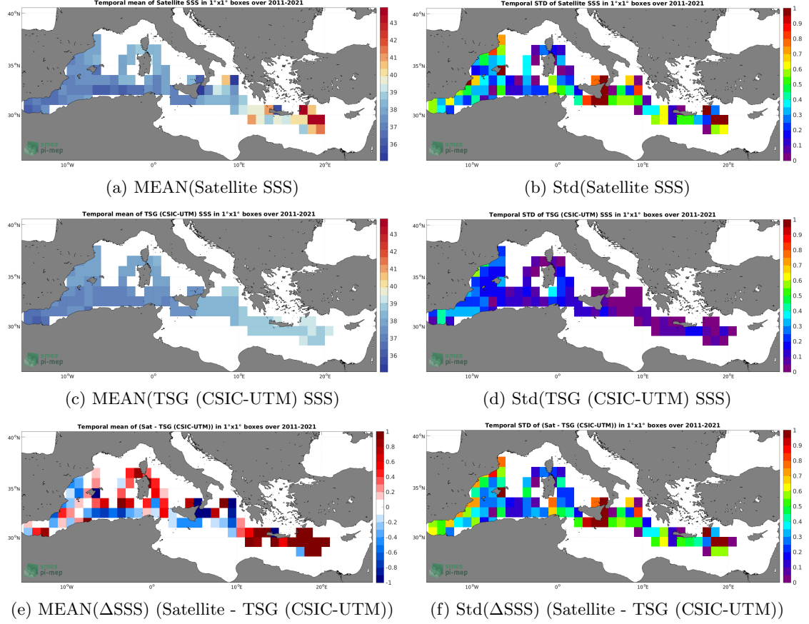
Figure 6: Temporal mean (left) and Std (right) of SSS from SMOS SSS L3 v2 - 9-Days (BEC) (top), TSG (CSIC-UTM) (middle), and of \Delta\text{SSS} (Satellite - TSG (CSIC-UTM)). Only match-up pairs are used to generate these maps.
