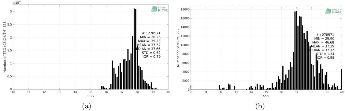
Figure 2: Histograms of SSS from TSG (CSIC-UTM) (a) and SMOS SSS L3 v2 - 9-Days (BEC) (b) considering all match-up pairs per bins of 0.1 over the Mediterranean Sea Pi-MEP region and for the full satellite product period.
