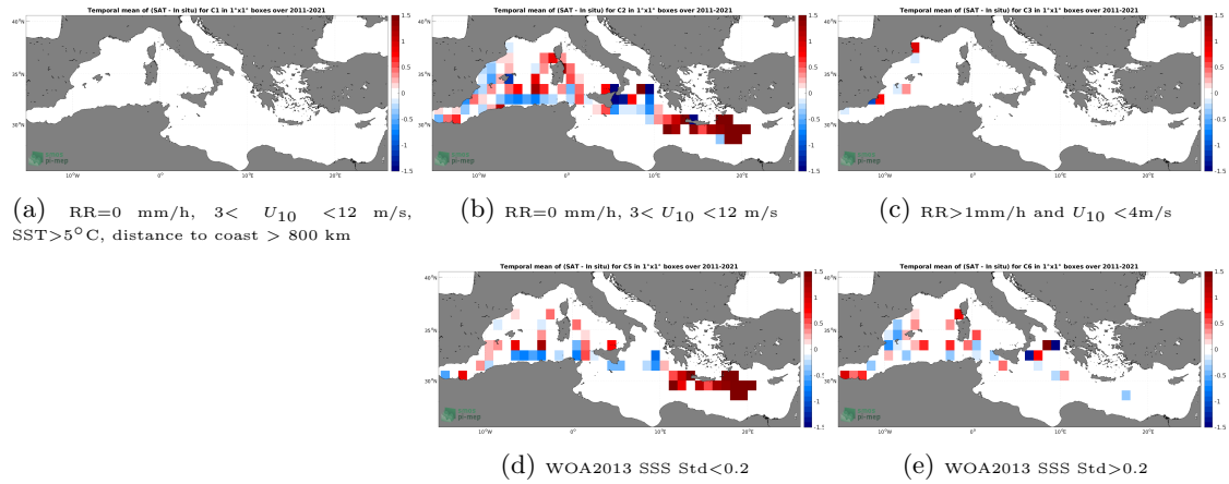
Figure 12: Temporal mean gridded over spatial boxes of size 1^\circ \times 1^\circ of \Delta SSS (SMOS SSS L3 v2 - 9-Days (BEC) - TSG (CSIC-UTM)) for 5 different subdatasets corresponding to:RR=0 mm/h, 3 < U_{10} < 12 m/s, SST >5^\circ\text{C} , distance to coast > 800 km (a), RR=0 mm/h, 3 < U_{10} < 12 m/s (b), RR >1 mm/h and U_{10} < 4 m/s (c), WOA2013 SSS Std <0.2 (d), WOA2013 SSS Std >0.2 (e).
