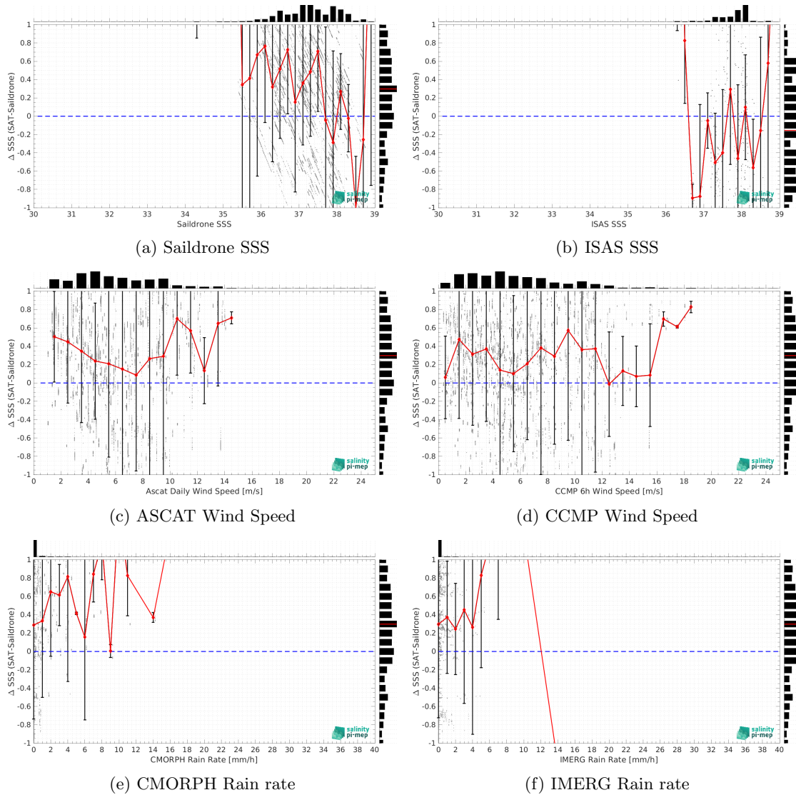
Figure 12: \Delta SSS (Satellite - Sailldrone) sorted as function of Sailldrone SSS values (a), ISAS SSS (b), ASCAT Wind speed (c), CCMP Wind speed (d), CMORPH rain rate (e) and IMERG rain rate (f). In all plots the median and Std of \Delta SSS for each bin is indicated by the red curves and black vertical thick bars ( \pm 1 Std).
