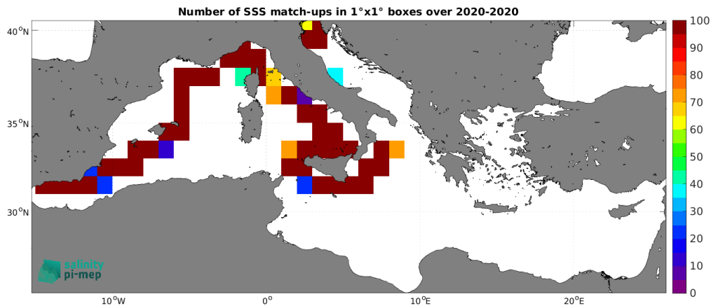
Figure 5: Number of SSS match-ups between Saildrone SSS and the SMOS SSS L3 v2 - 9-Days (BEC) SSS product for the Mediterranean Sea Pi-MEP region over 1^\circ \times 1^\circ boxes and for the full satellite product period.
