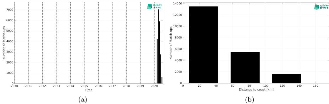
Figure 2: Number of match-ups between Saildrone and SMOS SSS L3 v2 - 9-Days (BEC) SSS as a function of time (a) and as function of the distance to coast (b) over the Mediterranean Sea Pi-MEP region and for the full satellite product period.
