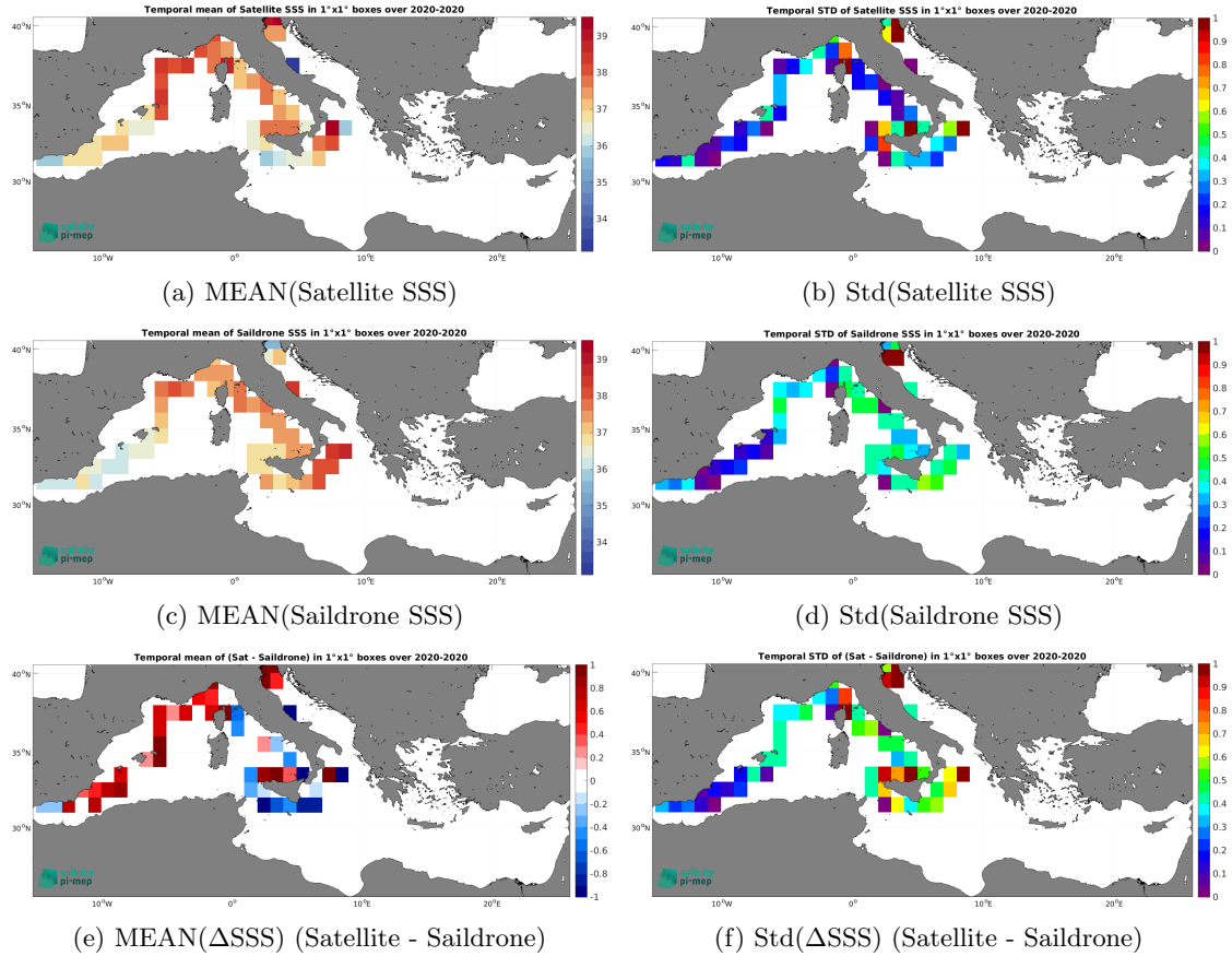
Figure 7: Temporal mean (left) and Std (right) of SSS from SMOS SSS L3 v2 - 9-Days (BEC) (top), Saildrone (middle), and of \Delta SSS (Satellite - Saildrone). Only match-up pairs are used to generate these maps.
