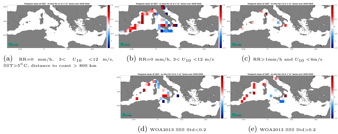
Figure 14: Temporal mean gridded over spatial boxes of size 1^\circ \times 1^\circ of \Delta SSS (SMOS SSS L3 v2 - 9-Days (BEC) - Saildrone) for 5 different subdatasets corresponding to:RR=0 mm/h, 3 < U_{10} < 12 m/s, SST >5^\circ\text{C} , distance to coast > 800 km (a), RR=0 mm/h, 3 < U_{10} < 12 m/s (b), RR >1 mm/h and U_{10} < 4 m/s (c), WOA2013 SSS Std <0.2 (d), WOA2013 SSS Std >0.2 (e).
