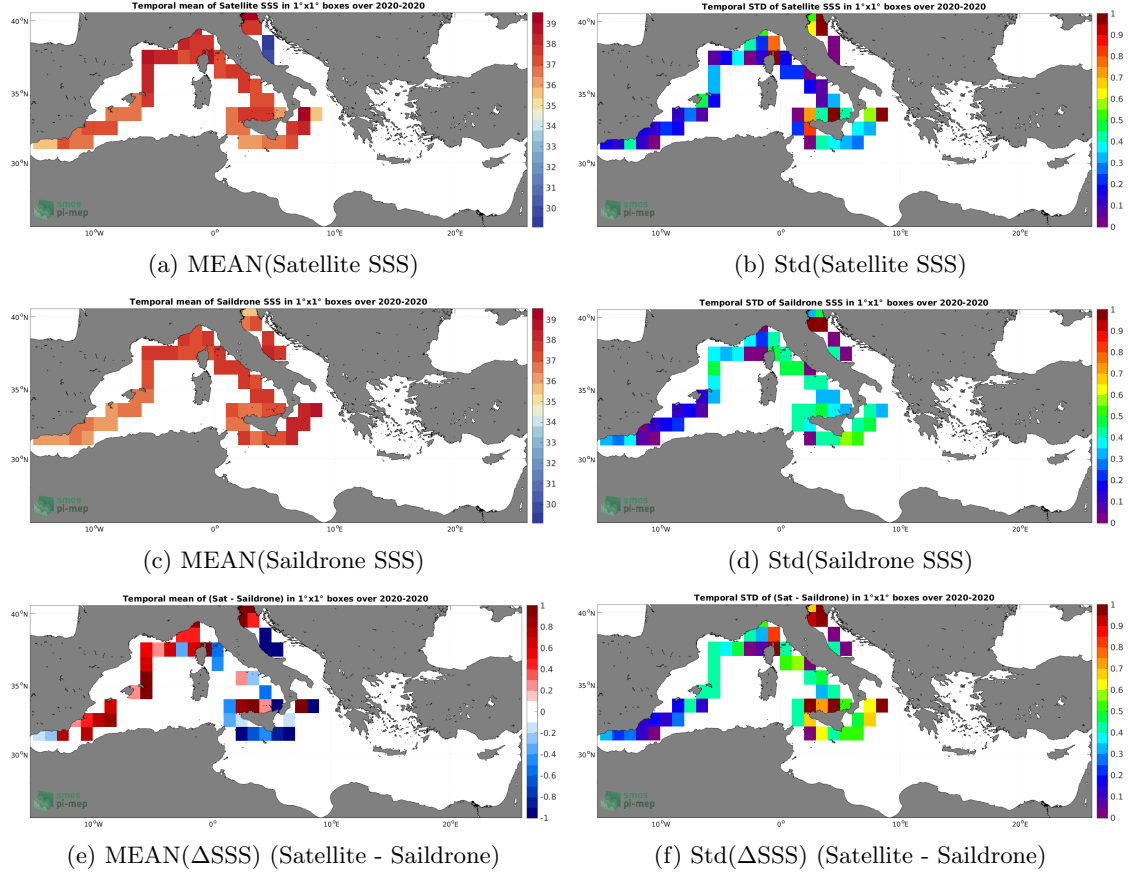
Figure 6: Temporal mean (left) and Std (right) of SSS from SMOS SSS L3 v2 - 9-Days (BEC) (top), Sairdrone (middle), and of \Delta SSS (Satellite - Sairdrone). Only match-up pairs are used to generate these maps.
