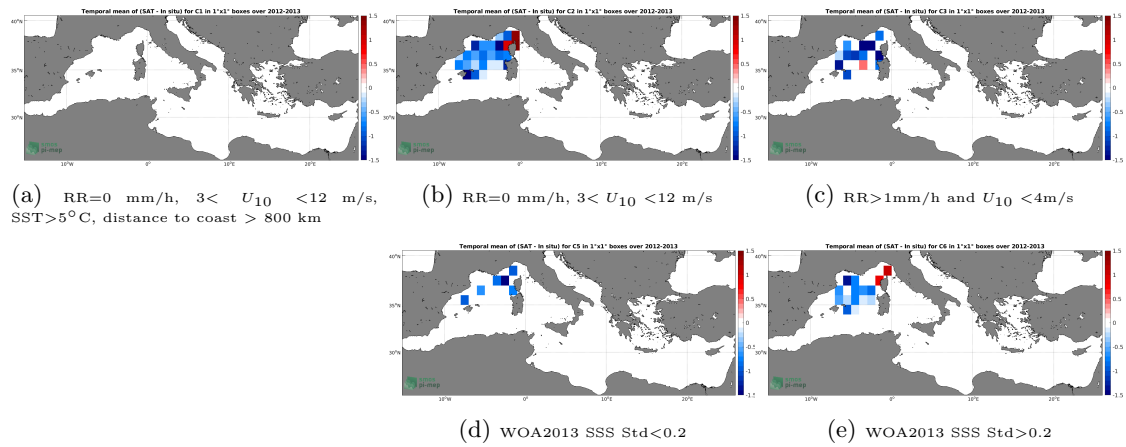
Figure 11: Temporal mean gridded over spatial boxes of size 1^\circ \times 1^\circ of \Delta SSS (SMOS SSS L3 v2 - 9-Days (BEC) - Surface drifters) for 5 different subdatasets corresponding to:RR=0 mm/h, 3 < U_{10} < 12 m/s, SST >5^\circ\text{C} , distance to coast > 800 km (a), RR=0 mm/h, 3 < U_{10} < 12 m/s (b), RR >1 mm/h and U_{10} < 4 m/s (c), WOA2013 SSS Std <0.2 (d), WOA2013 SSS Std >0.2 (e).
