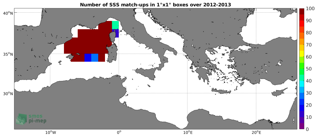
Figure 3: Number of SSS match-ups between Surface drifters SSS and the SMOS SSS L3 v2 - 9-Days (BEC) SSS product for the Mediterranean Sea Pi-MEP region over 1^\circ \times 1^\circ boxes and for the full satellite product period.
