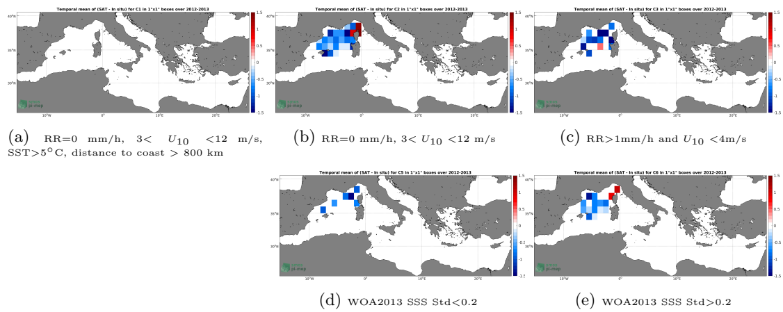
Figure 11: Temporal mean gridded over spatial boxes of size 1^\circ \times 1^\circ of \Delta SSS (SMOS SSS L3 v2 - 9-Days (BEC) - Surface drifters) for 5 different subdatasets corresponding to: RR=0 mm/h, 3 < U_{10} < 12 m/s, SST > 5°C, distance to coast > 800 km (a), RR=0 mm/h, 3 < U_{10} < 12 m/s (b), RR > 1mm/h and U_{10} < 4 m/s (c), WOA2013 SSS Std < 0.2 (d), WOA2013 SSS Std > 0.2 (e).
