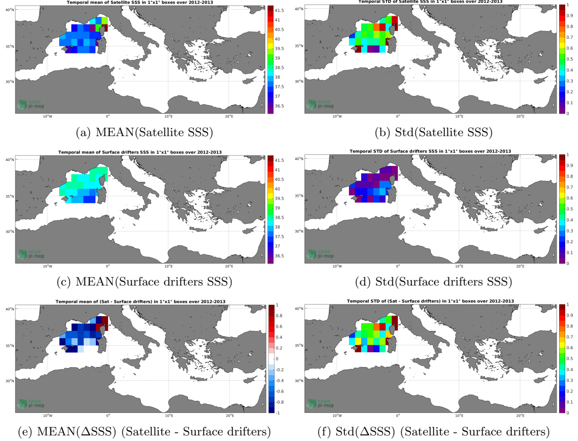
Figure 5: Temporal mean (left) and Std (right) of SSS from SMOS L3 v2 - 9-Days (BEC) (top), Surface drifters (middle), and of \Delta SSS (Satellite - Surface drifters). Only match-up pairs are used to generate these maps.
