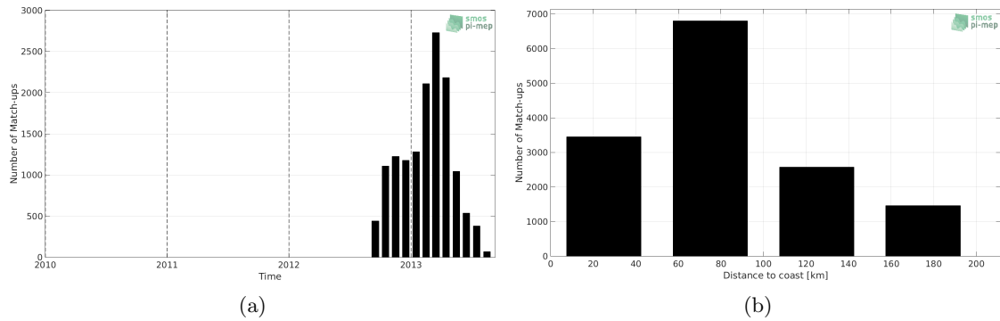
Figure 1: Number of match-ups between Surface drifters and SMOS L3 v2 - 9-Days (BEC) SSS as a function of time (a) and as function of the distance to coast (b) over the Mediterranean Sea Pi-MEP region and for the full satellite product period.
