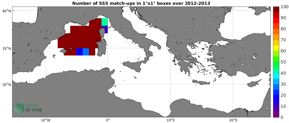
Figure 3: Number of SSS match-ups between Surface drifters SSS and the SMOS L3 v2 - 9-Days (BEC) SSS product for the Mediterranean Sea Pi-MEP region over 1^\circ \times 1^\circ boxes and for the full satellite product period.
