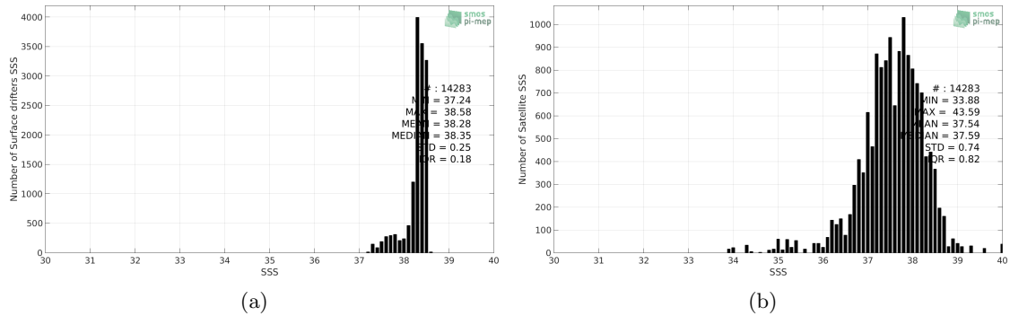
Figure 2: Histograms of SSS from Surface drifters (a) and SMOS L3 v2 - 9-Days (BEC) (b) considering all match-up pairs per bins of 0.1 over the Mediterranean Sea Pi-MEP region and for the full satellite product period.
