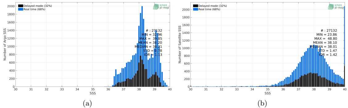
Figure 2: Histograms of SSS from Argo (a) and SMOS L3 v2 - 9-Days (BEC) (b) considering all match-up pairs per bins of 0.1 over the Mediterranean Sea Pi-MEP region and for the full satellite product period.
