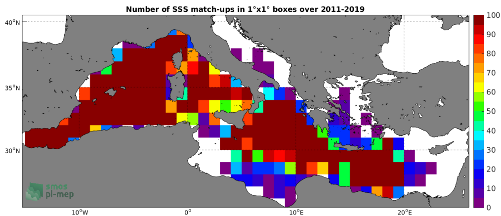
Figure 4: Number of SSS match-ups between Argon SSS and the SMOS L3 v2 - 9-Days (BEC) SSS product for the Mediterranean Sea Pi-MEP region over 1°x1° boxes and for the full satellite product period.
