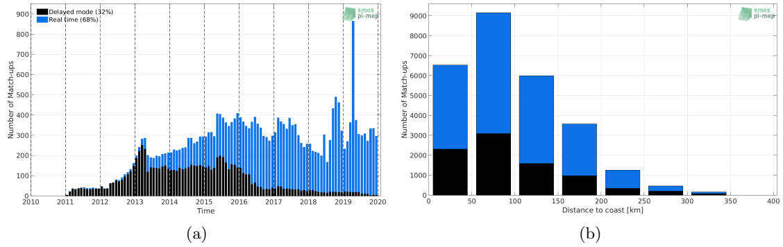
Figure 1: Number of match-ups between Argo and SMOS L3 v2 - 9-Days (BEC) SSS as a function of time (a) and as function of the distance to coast (b) over the Mediterranean Sea Pi-MEP region and for the full satellite product period.
