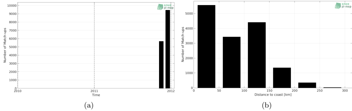
Figure 1: Number of match-ups between TSG-SAMOS and SMOS-L3-BEC-OA-V1-9DAYS-0.25DEG SSS as a function of time (a) and as function of the distance to coast (b) over the Mediterranean Sea Pi-MEP region and for the full satellite product period.
