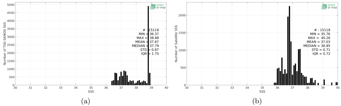
Figure 2: Histograms of SSS from TSG-SAMOS (a) and SMOS-L3-BEC-OA-V1-9DAYS-0.25DEG (b) considering all match-up pairs per bins of 0.1 over the Mediterranean Sea Pi-MEP region and for the full satellite product period.
