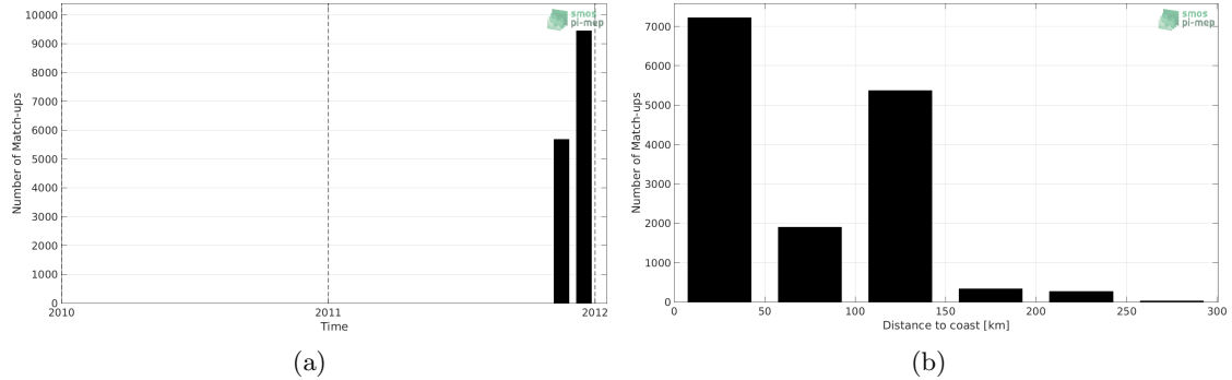
Figure 1: Number of match-ups between TSG-SAMOS and SMOS-L3-BEC-OA-V1-9DAYS-0.25DEG SSS as a function of time (a) and as function of the distance to coast (b) over the Mediterranean Sea Pi-MEP region and for the full satellite product period.
