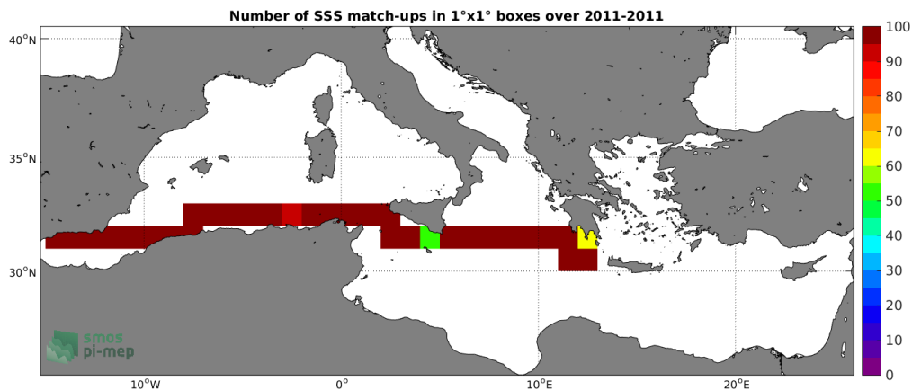
Figure 4: Number of SSS match-ups between TSG-SAMOS SSS and the SMOS-L3-BEC-OA-V1-9DAYS-0.25DEG SSS product for the Mediterranean Sea Pi-MEP region over 1^\circ \times 1^\circ boxes and for the full satellite product period.
