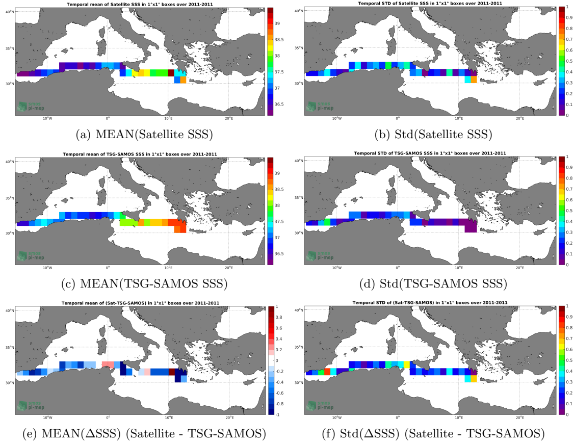
Figure 6: Temporal mean (left) and Std (right) of SSS from SMOS-L3-BEC-OA-V1-9DAYS-0.25DEG (top), TSG-SAMOS (middle), and of \Delta SSS (Satellite - TSG-SAMOS). Only match-up pairs are used to generate these maps.
