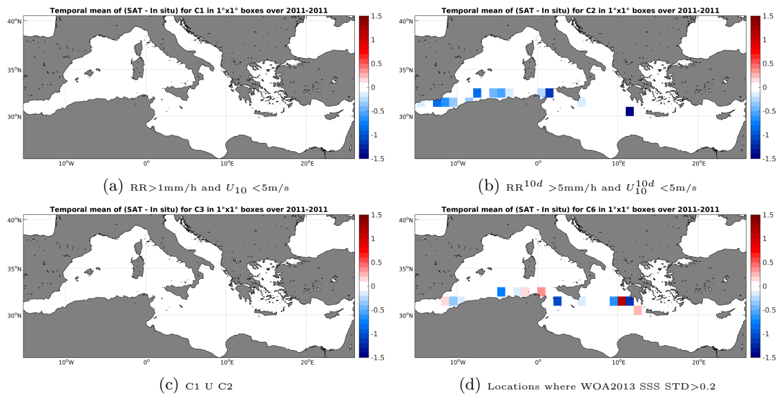
Figure 12: Temporal mean gridded over spatial boxes of size 1^\circ \times 1^\circ of \Delta SSS (SMOS-L3-BEC-OA-V1-9DAYS-0.25DEG - TSG-SAMOS) for 4 different subdatasets corresponding to:RR >1 mm/h and U_{10} < 5 m/s (a), RR^{10d} > 5 mm/h and U_{10}^{10d} < 5 m/s (b), C1 U C2 (c),Locations where WOA2013 SSS STD >0.2 (d).
