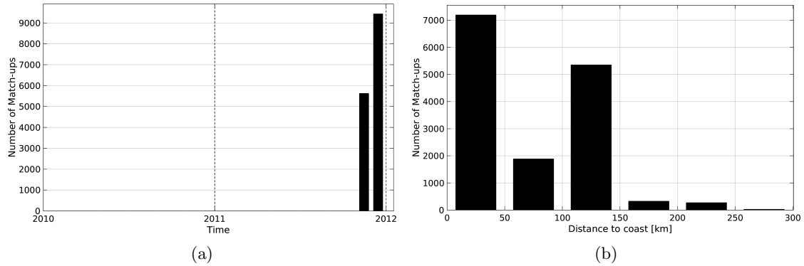
Figure 1: Number of match-ups between TSG-SAMOS and SMOS-L3-BEC-OA-V1-9DAYS-0.25DEG SSS as a function of time (a) and as function of the distance to coast (b) over the Mediterranean Sea Pi-MEP region and for the full satellite product period.
