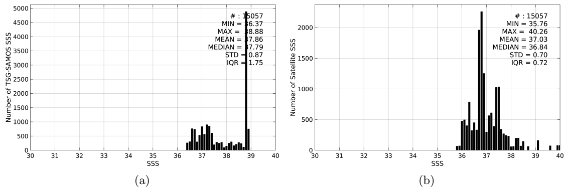
Figure 2: Histograms of SSS from TSG-SAMOS (a) and SMOS-L3-BEC-OA-V1-9DAYS-0.25DEG (b) considering all match-up pairs per bins of 0.1 over the Mediterranean Sea Pi-MEP region and for the full satellite product period.
