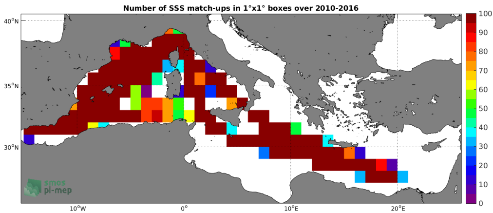
Figure 4: Number of SSS match-ups between TSG-LEGOS-DM SSS and the SMOS-L3-BEC-OA-V1-9DAYS-0.25DEG SSS product for the Mediterranean Sea Pi-MEP region over 1^\circ \times 1^\circ boxes and for the full satellite product period.
