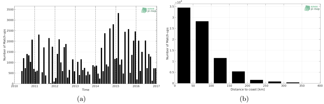
Figure 1: Number of match-ups between TSG-LEGOS-DM and SMOS-L3-BEC-OA-V1-9DAYS-0.25DEG SSS as a function of time (a) and as function of the distance to coast (b) over the Mediterranean Sea Pi-MEP region and for the full satellite product period.
