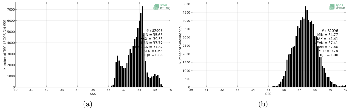
Figure 2: Histograms of SSS from TSG-LEGOS-DM (a) and SMOS-L3-BEC-OA-V1-9DAYS-0.25DEG (b) considering all match-up pairs per bins of 0.1 over the Mediterranean Sea Pi-MEP region and for the full satellite product period.
