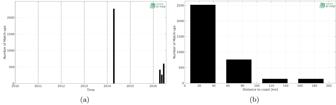
Figure 1: Number of match-ups between TSG-GOSUD-Sailing-ship and SMOS-L3-BEC-OA-V1-9DAYS-0.25DEG SSS as a function of time (a) and as function of the distance to coast (b) over the Mediterranean Sea Pi-MEP region and for the full satellite product period.
