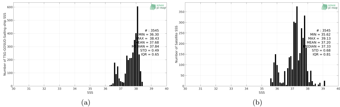
Figure 2: Histograms of SSS from TSG-GOSUD-Sailing-ship (a) and SMOS-L3-BEC-OA-V1-9DAYS-0.25DEG (b) considering all match-up pairs per bins of 0.1 over the Mediterranean Sea Pi-MEP region and for the full satellite product period.
