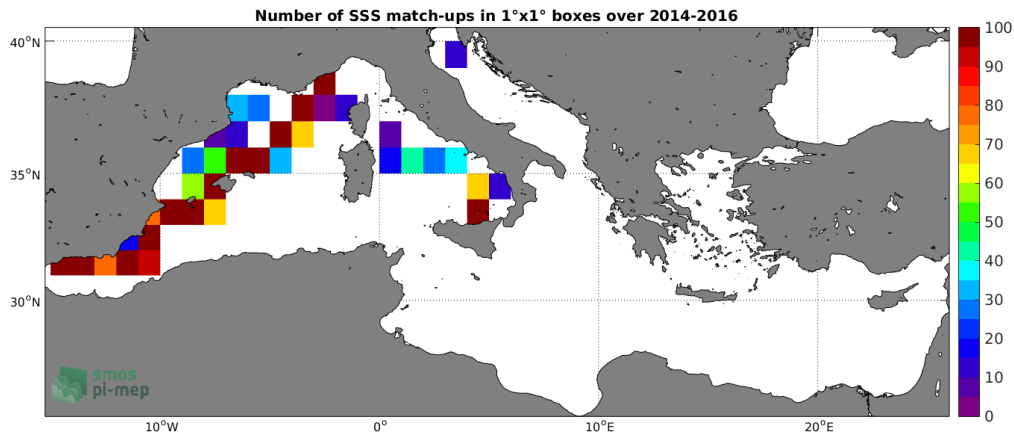
Figure 4: Number of SSS match-ups between TSG-GOSUD-Sailing-ship SSS and the SMOS-L3-BEC-OA-V1-9DAYS-0.25DEG SSS product for the Mediterranean Sea Pi-MEP region over 1°x1° boxes and for the full satellite product period.
