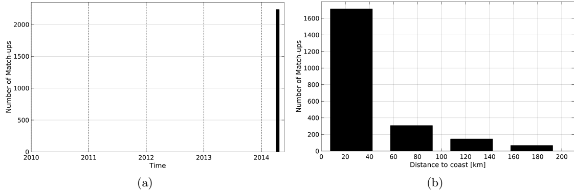
Figure 1: Number of match-ups between TSG-GOSUD-Sailing-ship and SMOS-L3-BEC-OA-V1-9DAYS-0.25DEG SSS as a function of time (a) and as function of the distance to coast (b) over the Mediterranean Sea Pi-MEP region and for the full satellite product period.
