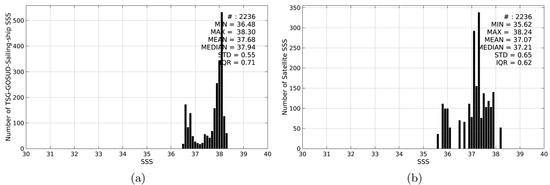
Figure 2: Histograms of SSS from TSG-GOSUD-Sailing-ship (a) and SMOS-L3-BEC-OA-V1-9DAYS-0.25DEG (b) considering all match-up pairs per bins of 0.1 over the Mediterranean Sea Pi-MEP region and for the full satellite product period.
