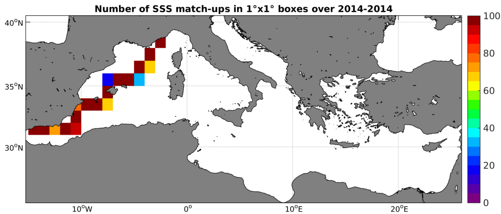
Figure 4: Number of SSS match-ups between TSG-GOSUD-Sailing-ship SSS and the SMOS-L3-BEC-OA-V1-9DAYS-0.25DEG SSS product for the Mediterranean Sea Pi-MEP region over 1^\circ \times 1^\circ boxes and for the full satellite product period.
