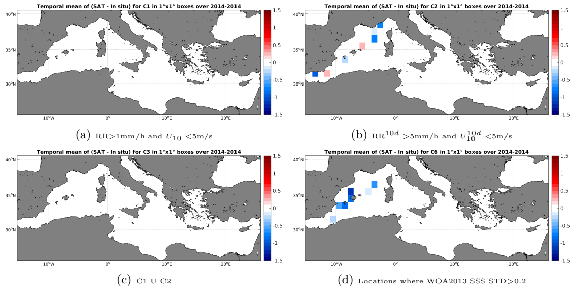
Figure 12: Temporal mean gridded over spatial boxes of size 1°x1° of \Delta SSS (SMOS-L3-BEC-OA-V1-9DAYS-0.25DEG - TSG-GOSUD-Sailing-ship) for 4 different subdatasets corresponding to: RR > 1mm/h and U_{10} < 5m/s (a), RR 10d > 5mm/h and U_{10}^{10d} < 5m/s (b), C1 U C2 (c), Locations where WOA2013 SSS STD > 0.2 (d).
