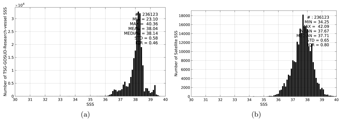
Figure 2: Histograms of SSS from TSG-GOSUD-Research-vessel (a) and SMOS-L3-BEC-OA-V1-9DAYS-0.25DEG (b) considering all match-up pairs per bins of 0.1 over the Mediterranean Sea Pi-MEP region and for the full satellite product period.
