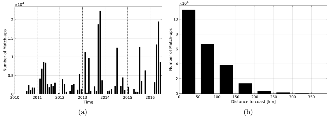
Figure 1: Number of match-ups between TSG-GOSUD-Research-vessel and SMOS-L3-BEC-OA-V1-9DAYS-0.25DEG SSS as a function of time (a) and as function of the distance to coast (b) over the Mediterranean Sea Pi-MEP region and for the full satellite product period.
