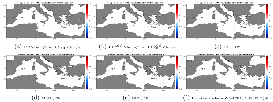
Figure 12: Temporal mean gridded over spatial boxes of size 1^\circ \times 1^\circ of \Delta SSS (SMOS-L3-BEC-OA-V1-9DAYS-0.25DEG - Sea mammals) for 6 different subdatasets corresponding to: RR > 1\text{mm/h} and U_{10} < 5\text{m/s} (a), RR^{10d} > 5\text{mm/h} and U_{10}^{10d} < 5\text{m/s} (b), C1 U C2 (c), MLD < 20\text{m} (d), BLT > 10\text{m} (e), Locations where WOA2013 SSS STD > 0.2 (f).
