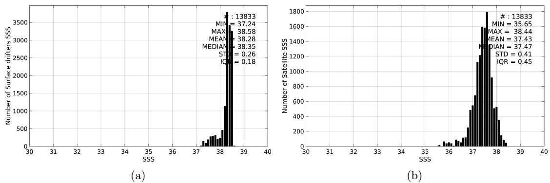
Figure 2: Histograms of SSS from Surface drifters (a) and SMOS-L3-BEC-OA-V1-9DAYS-0.25DEG (b) considering all match-up pairs per bins of 0.1 over the Mediterranean Sea Pi-MEP region and for the full satellite product period.
