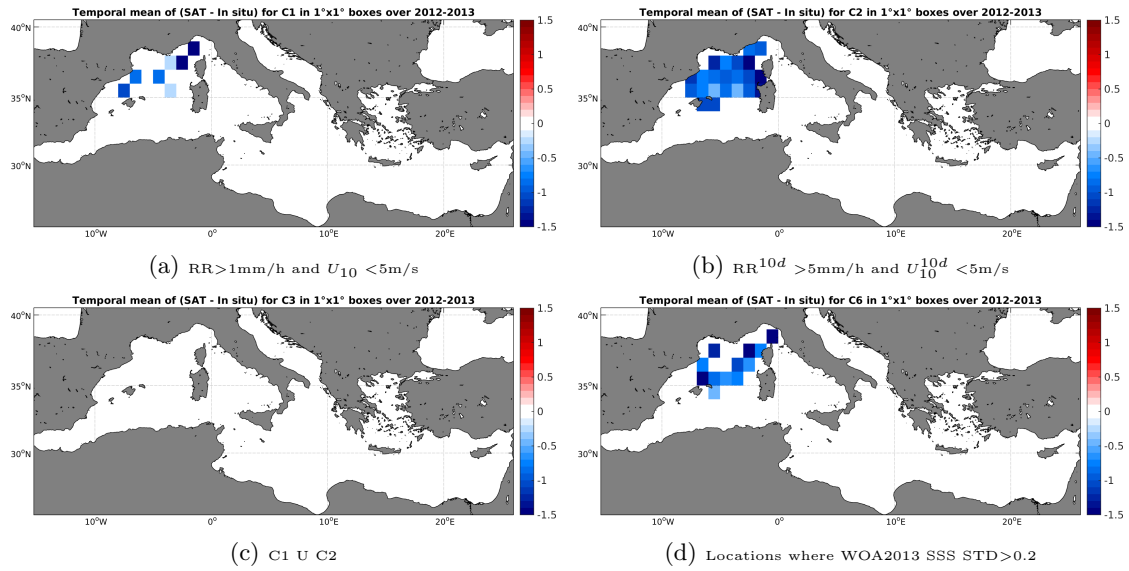
Figure 11: Temporal mean gridded over spatial boxes of size 1^\circ \times 1^\circ of \Delta SSS (SMOS-L3-BEC-OA-V1-9DAYS-0.25DEG - Surface drifters) for 4 different subdatasets corresponding to:RR > 1 mm/h and U_{10} < 5 m/s (a), RR 10d > 5 mm/h and U_{10}^{10d} < 5 m/s (b), C1 U C2 (c),Locations where WOA2013 SSS STD > 0.2 (d).
