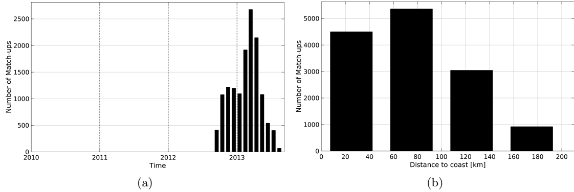
Figure 1: Number of match-ups between Surface drifters and SMOS-L3-BEC-OA-V1-9DAYS-0.25DEG SSS as a function of time (a) and as function of the distance to coast (b) over the Mediterranean Sea Pi-MEP region and for the full satellite product period.
