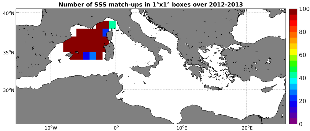
Figure 3: Number of SSS match-ups between Surface drifters SSS and the SMOS-L3-BEC-OA-V1-9DAYS-0.25DEG SSS product for the Mediterranean Sea Pi-MEP region over 1^\circ \times 1^\circ boxes and for the full satellite product period.
