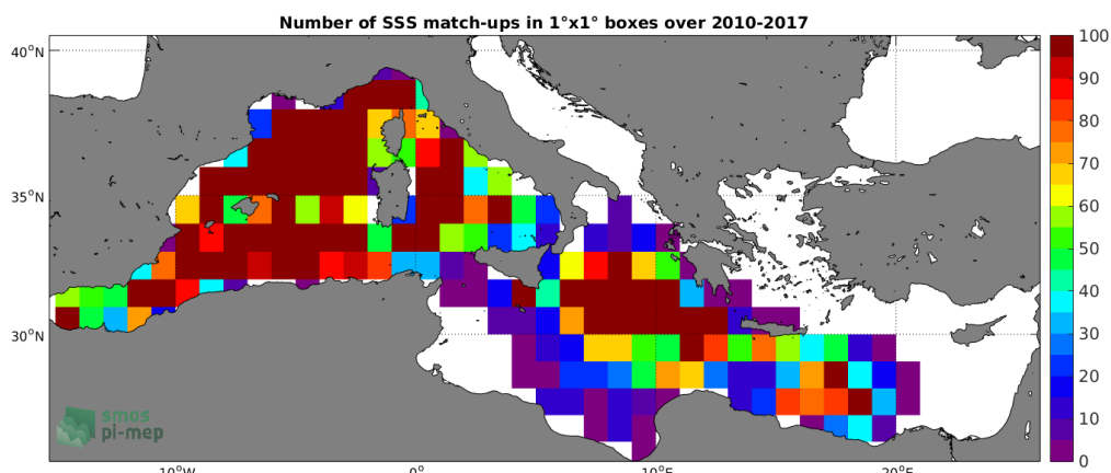
Figure 4: Number of SSS match-ups between Argo SSS and the SMOS-L3-BEC-OA-V1-9DAYS-0.25DEG SSS product for the Mediterranean Sea Pi-MEP region over 1°x1° boxes and for the full satellite product period.
