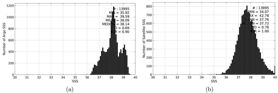
Figure 2: Histograms of SSS from Argo (a) and SMOS-L3-BEC-OA-V1-9DAYS-0.25DEG (b) considering all match-up pairs per bins of 0.1 over the Mediterranean Sea Pi-MEP region and for the full satellite product period.
