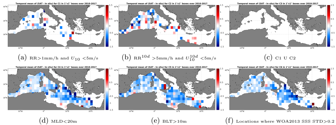
Figure 12: Temporal mean gridded over spatial boxes of size 1^\circ \times 1^\circ of \Delta SSS (SMOS-L3-BEC-OA-V1-9DAYS-0.25DEG - Argo) for 6 different subdatasets corresponding to: RR > 1mm/h and U_{10} < 5\text{m/s} (a), RR^{10d} > 5\text{mm/h} and U_{10}^{10d} < 5\text{m/s} (b), C1 U C2 (c), MLD < 20m (d), BLT > 10m (e), Locations where WOA2013 SSS STD > 0.2 (f).
