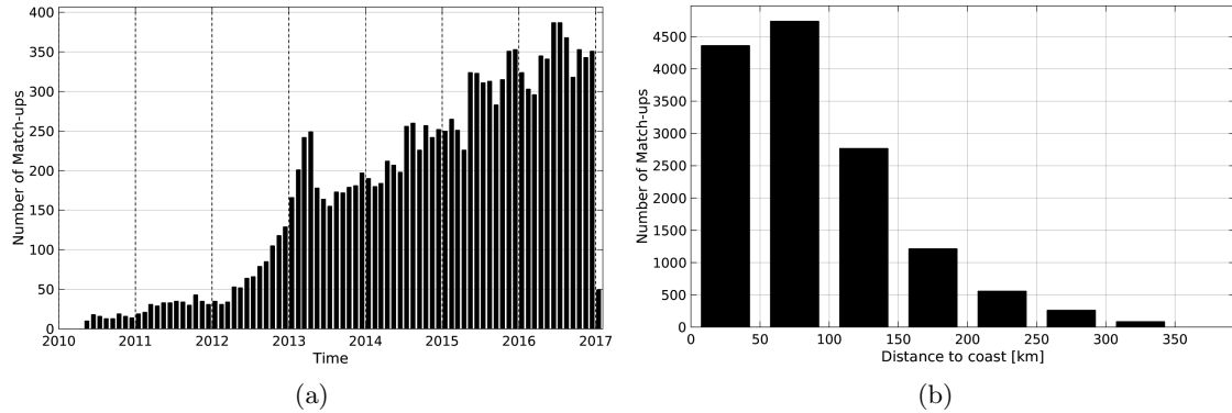
Figure 1: Number of match-ups between Argo and SMOS-L3-BEC-OA-V1-9DAYS-0.25DEG SSS as a function of time (a) and as function of the distance to coast (b) over the Mediterranean Sea Pi-MEP region and for the full satellite product period.
