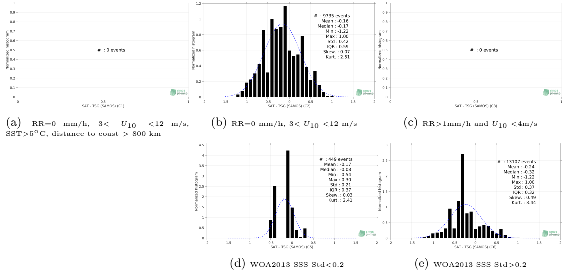
Figure 13: Normalized histogram of \Delta SSS (SMOS SSS L3 MED-ATL-OA v2 - 9 Days (BEC) - TSG (SAMOS)) for 5 different subdatasets corresponding to: RR=0 mm/h, 3 < U_{10} < 12 m/s, SST>5°C, distance to coast > 800 km (a), RR=0 mm/h, 3 < U_{10} < 12 m/s (b), RR>1mm/h and U_{10} < 4 m/s (c), WOA2013 SSS Std<0.2 (d), WOA2013 SSS Std>0.2 (e).
