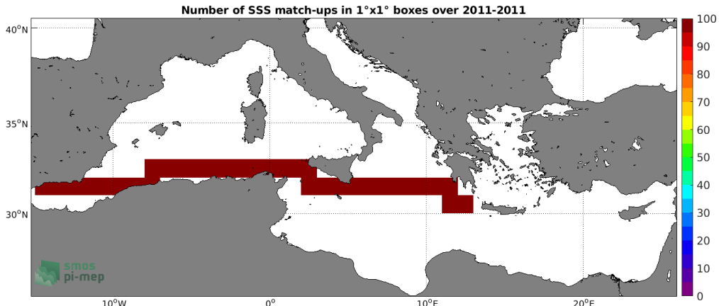
Figure 4: Number of SSS match-ups between TSG (SAMOS) SSS and the SMOS SSS L3 MED-ATL-OA v2 - 9 Days (BEC) SSS product for the Mediterranean Sea Pi-MEP region over 1^\circ \times 1^\circ boxes and for the full satellite product period.
