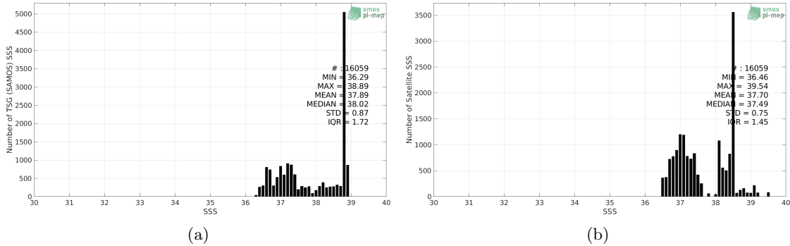
Figure 2: Histograms of SSS from TSG (SAMOS) (a) and SMOS SSS L3 MED-ATL-OA v2 - 9 Days (BEC) (b) considering all match-up pairs per bins of 0.1 over the Mediterranean Sea Pi-MEP region and for the full satellite product period.
