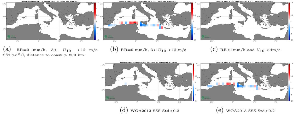
Figure 12: Temporal mean gridded over spatial boxes of size 1^{\circ}\times 1^{\circ} of \Delta\text{SSS} (SMOS SSS L3 MED-ATL-OA v2 - 9 Days (BEC) - TSG (SAMOS)) for 5 different subdatasets corresponding to:RR=0 mm/h, 3 < U_{10} < 12 m/s, SST > 5^{\circ}\text{C} , distance to coast > 800 km (a), RR=0 mm/h, 3 < U_{10} < 12 m/s (b), RR > 1 mm/h and U_{10} < 4 m/s (c), WOA2013 SSS Std < 0.2 (d), WOA2013 SSS Std > 0.2 (e).
