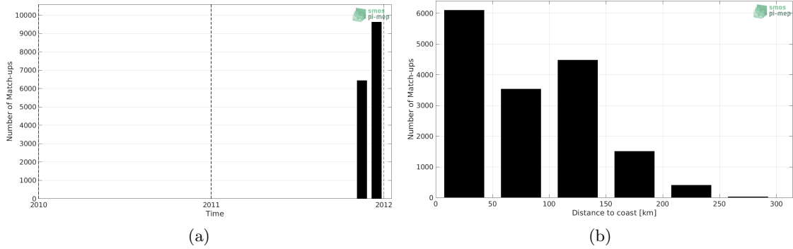
Figure 1: Number of match-ups between TSG (SAMOS) and SMOS SSS L3 MED-ATL-OA v2 - 9 Days (BEC) SSS as a function of time (a) and as function of the distance to coast (b) over the Mediterranean Sea Pi-MEP region and for the full satellite product period.
