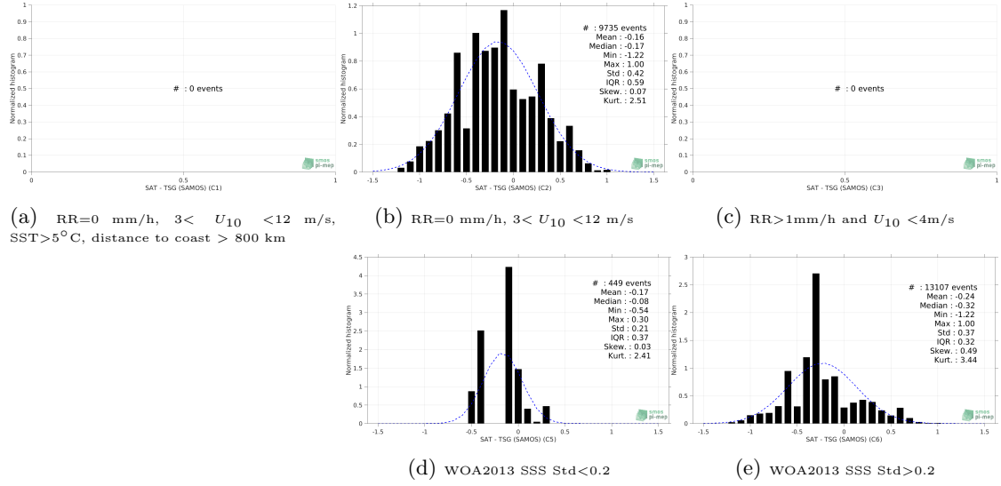
Figure 13: Normalized histogram of \Delta\text{SSS} (SMOS SSS L3 MED-ATL-OA v2 - 9 Days (BEC) - TSG (SAMOS)) for 5 different subdatasets corresponding to: RR=0 mm/h, 3 < U_{10} < 12 m/s, SST > 5^\circ\text{C} , distance to coast > 800 km (a), RR=0 mm/h, 3 < U_{10} < 12 m/s (b), RR > 1 mm/h and U_{10} < 4 m/s (c), WOA2013 SSS Std < 0.2 (d), WOA2013 SSS Std > 0.2 (e).
