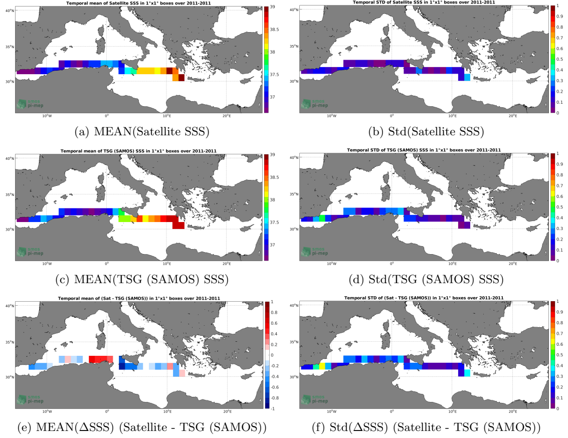
Figure 6: Temporal mean (left) and Std (right) of SSS from SMOS SSS L3 MED-ATL-OA v2 - 9 Days (BEC) (top), TSG (SAMOS) (middle), and of \Delta SSS (Satellite - TSG (SAMOS)). Only match-up pairs are used to generate these maps.
