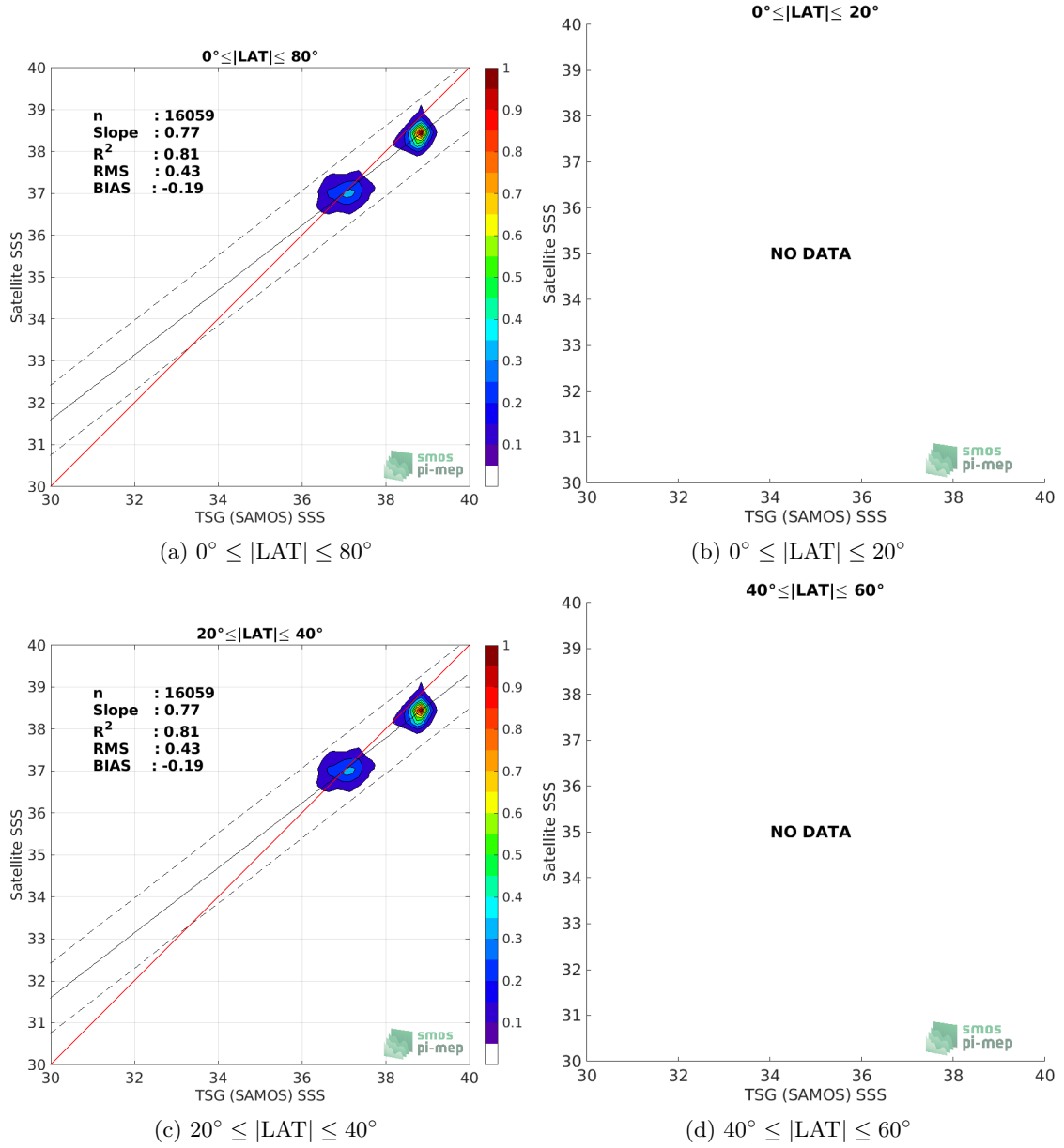
Figure 9: Contour maps of the concentration of SMOS SSS L3 MED-ATL-OA v2 - 9 Days (BEC) SSS (y-axis) versus TSG (SAMOS) SSS (x-axis) at match-up pairs for different latitude bands. For each plot, the red line shows x=y . The black thin and dashed lines indicate a linear fit through the data cloud and the \pm 95\% confidence levels, respectively. The number match-up pairs n , the slope and R^2 coefficient of the linear fit, the root mean square (RMS) and the mean bias between satellite and in situ data are indicated for each latitude band in each plots.
