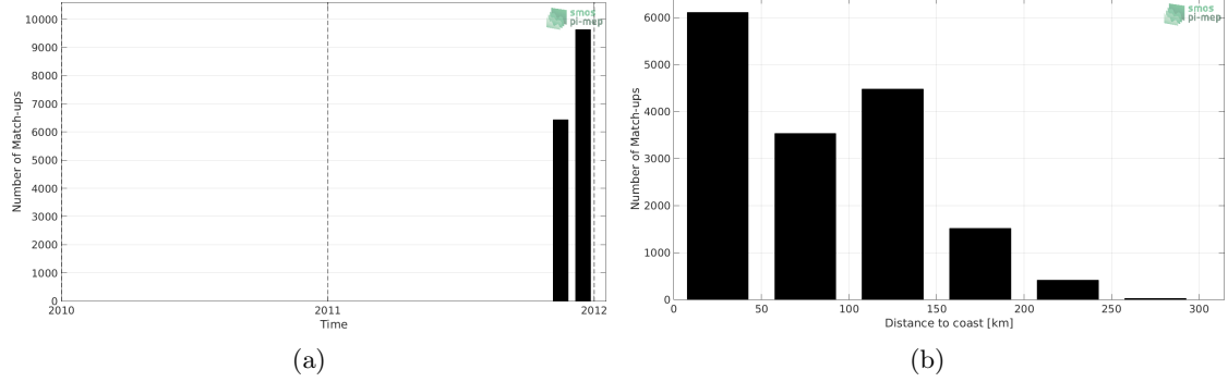
Figure 1: Number of match-ups between TSG-SAMOS and SMOS L3 MED-ATL-OA v2 - 9 Days (BEC) SSS as a function of time (a) and as function of the distance to coast (b) over the Mediterranean Sea Pi-MEP region and for the full satellite product period.
