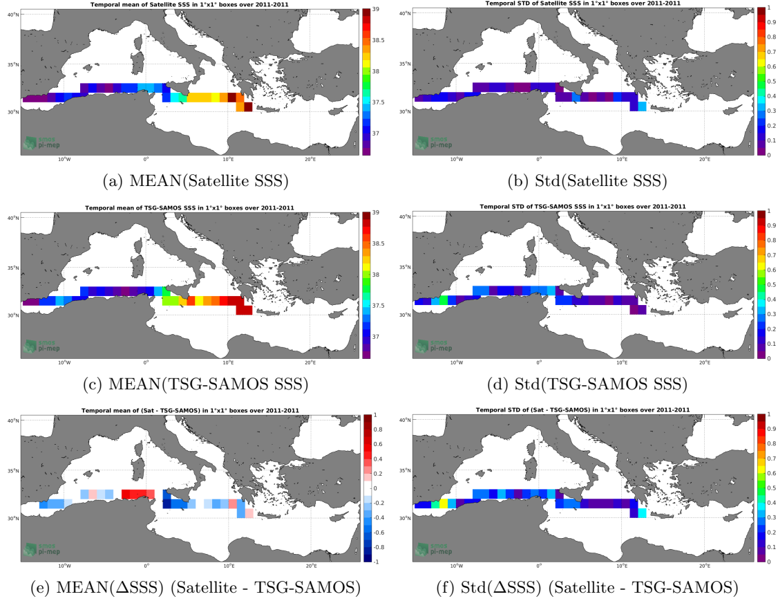
Figure 6: Temporal mean (left) and Std (right) of SSS from SMOS L3 MED-ATL-OA v2 - 9 Days (BEC) (top), TSG-SAMOS (middle), and of \Delta SSS (Satellite - TSG-SAMOS). Only match-up pairs are used to generate these maps.
