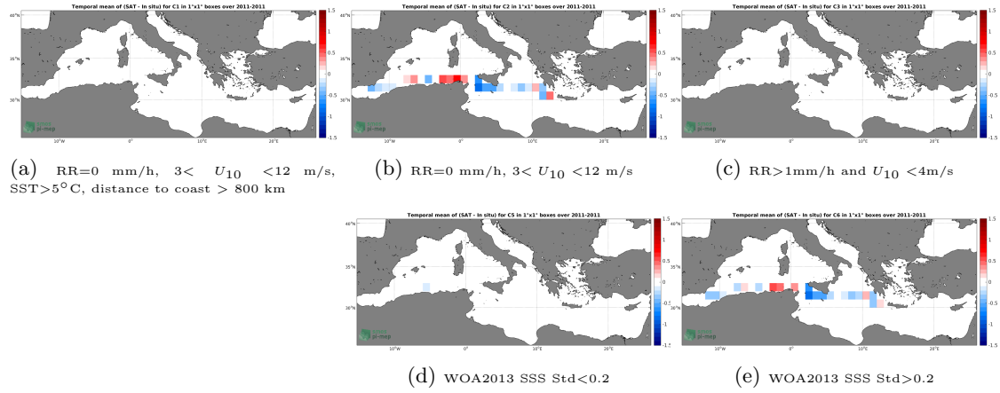
Figure 12: Temporal mean gridded over spatial boxes of size 1^{\circ}\times 1^{\circ} of \Delta\text{SSS} (SMOS L3 MED-ATL-OA v2 - 9 Days (BEC) - TSG-SAMOS) for 5 different subdatasets corresponding to:RR=0 mm/h, 3 < U_{10} < 12 m/s, SST >5^{\circ}\text{C} , distance to coast > 800 km (a), RR=0 mm/h, 3 < U_{10} < 12 m/s (b), RR >1 mm/h and U_{10} < 4 m/s (c), WOA2013 SSS Std <0.2 (d), WOA2013 SSS Std >0.2 (e).
