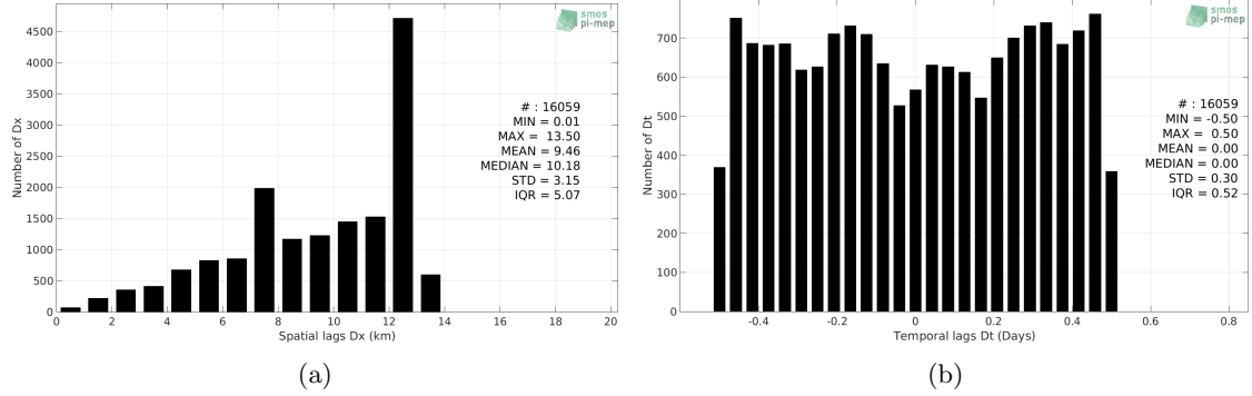
Figure 5: Histograms of the spatial (a) and temporal (b) lags between the time of the TSG-SAMOS measurements and the date of the corresponding SMOS L3 MED-ATL-OA v2 - 9 Days (BEC) SSS product.
