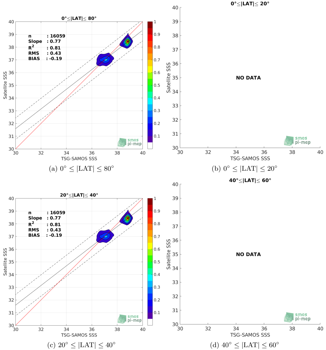
Figure 9: Contour maps of the concentration of SMOS L3 MED-ATL-OA v2 - 9 Days (BEC) SSS (y-axis) versus TSG-SAMOS SSS (x-axis) at match-up pairs for different latitude bands. For each plot, the red line shows x=y . The black thin and dashed lines indicate a linear fit through the cloud and the \pm 95\% confidence levels, respectively. The number match-up pairs n , the slope and R^2 coefficient of the linear fit, the root mean square (RMS) and the mean bias between satellite and in situ data are indicated for each latitude band in each plots.
