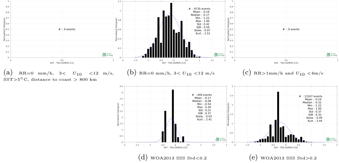
Figure 13: Normalized histogram of \Delta SSS (SMOS L3 MED-ATL-OA v2 - 9 Days (BEC) - TSG-SAMOS) for 5 different subdatasets corresponding to: RR=0 mm/h, 3 < U_{10} < 12 m/s, SST>5°C, distance to coast > 800 km (a), RR=0 mm/h, 3 < U_{10} < 12 m/s (b), RR>1mm/h and U_{10} < 4 m/s (c), WOA2013 SSS Std<0.2 (d), WOA2013 SSS Std>0.2 (e).
