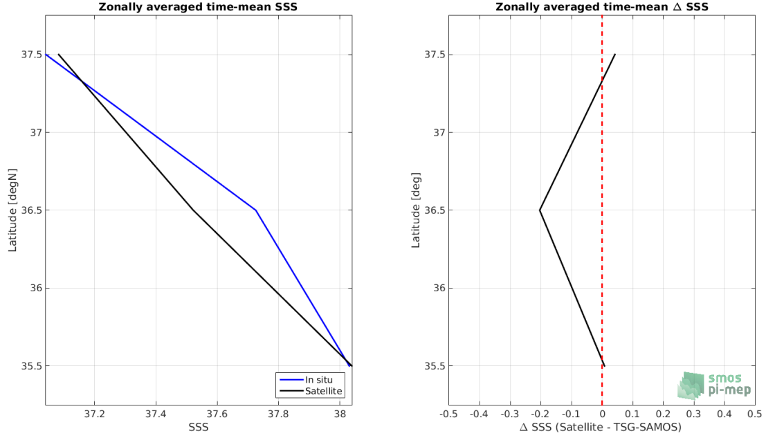
Figure 8: Left panel: Zonal mean SSS from SMOS L3 MED-ATL-OA v2 - 9 Days (BEC) satellite product (black) and from TSG-SAMOS (blue). Right panel: Zonal mean of \Delta SSS (Satellite - TSG-SAMOS) for all the collected Pi-MEP match-up pairs estimated over the full satellite product period.
