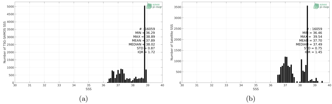
Figure 2: Histograms of SSS from TSG-SAMOS (a) and SMOS L3 MED-ATL-OA v2 - 9 Days (BEC) (b) considering all match-up pairs per bins of 0.1 over the Mediterranean Sea Pi-MEP region and for the full satellite product period.
