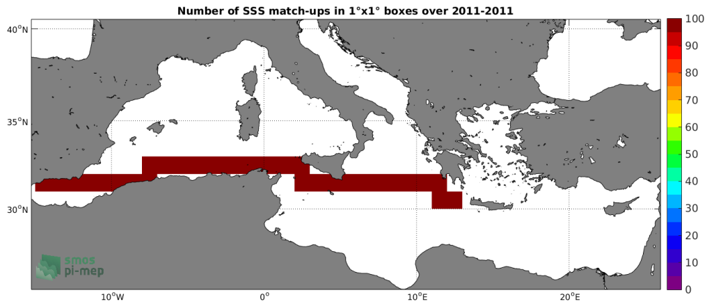
Figure 4: Number of SSS match-ups between TSG-SAMOS SSS and the SMOS L3 MED-ATL-OA v2 - 9 Days (BEC) SSS product for the Mediterranean Sea Pi-MEP region over 1^\circ \times 1^\circ boxes and for the full satellite product period.
