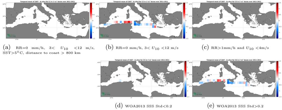
Figure 12: Temporal mean gridded over spatial boxes of size 1^\circ \times 1^\circ of \Delta SSS (SMOS-L3-BEC-MED-ATL-OA-V2-9DAYS-0.25DEG - TSG-SAMOS) for 5 different subdatasets corresponding to: RR=0 mm/h, 3 < U_{10} < 12 m/s, SST > 5^\circ C , distance to coast > 800 km (a), RR=0 mm/h, 3 < U_{10} < 12 m/s (b), RR > 1 mm/h and U_{10} < 4 m/s (c), WOA2013 SSS Std < 0.2 (d), WOA2013 SSS Std > 0.2 (e).
