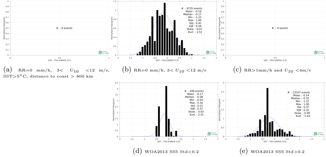
Figure 13: Normalized histogram of \Delta SSS (SMOS-L3-BEC-MED-ATL-OA-V2-9DAYS-0.25DEG - TSG-SAMOS) for 5 different subdatasets corresponding to: RR=0 mm/h, 3 < U_{10} < 12 m/s, SST > 5°C, distance to coast > 800 km (a), RR=0 mm/h, 3 < U_{10} < 12 m/s (b), RR > 1mm/h and U_{10} < 4 m/s (c), WOA2013 SSS Std < 0.2 (d), WOA2013 SSS Std > 0.2 (e).
