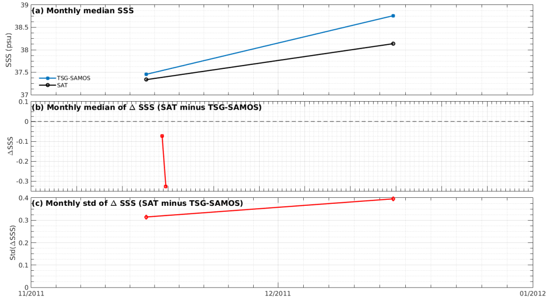
Figure 7: Time series of the monthly median SSS (top), median of \Delta SSS (Satellite - TSG-SAMOS) and Std of \Delta SSS (Satellite - TSG-SAMOS) over the Mediterranean Sea Pi-MEP region considering all match-ups collected by the Pi-MEP.
