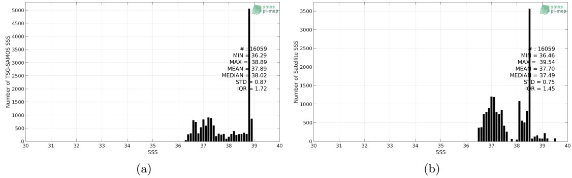
Figure 2: Histograms of SSS from TSG-SAMOS (a) and SMOS-L3-BEC-MED-ATL-OA-V2-9DAYS-0.25DEG (b) considering all match-up pairs per bins of 0.1 over the Mediterranean Sea Pi-MEP region and for the full satellite product period.
