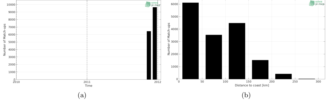
Figure 1: Number of match-ups between TSG-SAMOS and SMOS-L3-BEC-MED-ATL-OA-V2-9DAYS-0.25DEG SSS as a function of time (a) and as function of the distance to coast (b) over the Mediterranean Sea Pi-MEP region and for the full satellite product period.
