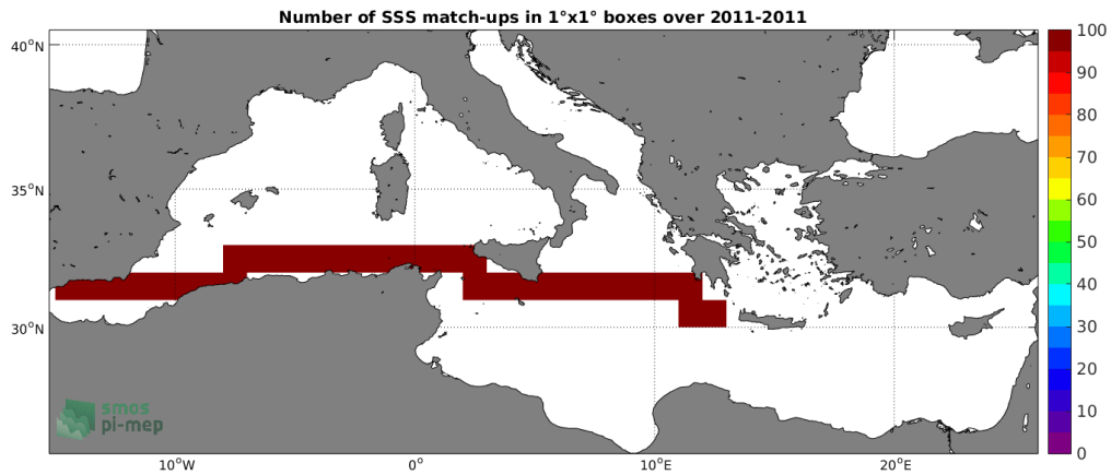
Figure 4: Number of SSS match-ups between TSG-SAMOS SSS and the SMOS-L3-BEC-MED-ATL-OA-V2-9DAYS-0.25DEG SSS product for the Mediterranean Sea Pi-MEP region over 1^\circ \times 1^\circ boxes and for the full satellite product period.
