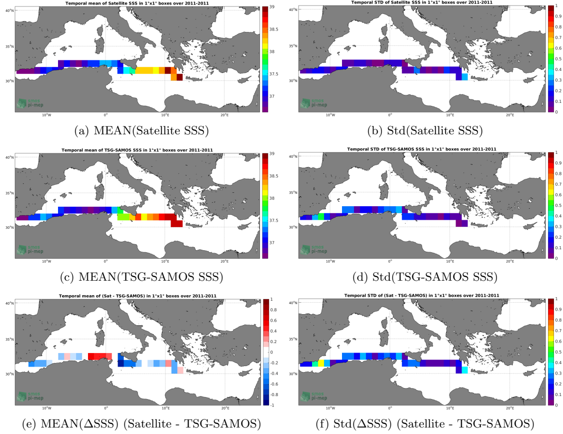
Figure 6: Temporal mean (left) and Std (right) of SSS from SMOS-L3-BEC-MED-ATL-OA-V2-9DAYS-0.25DEG (top), TSG-SAMOS (middle), and of \Delta SSS (Satellite - TSG-SAMOS). Only match-up pairs are used to generate these maps.
