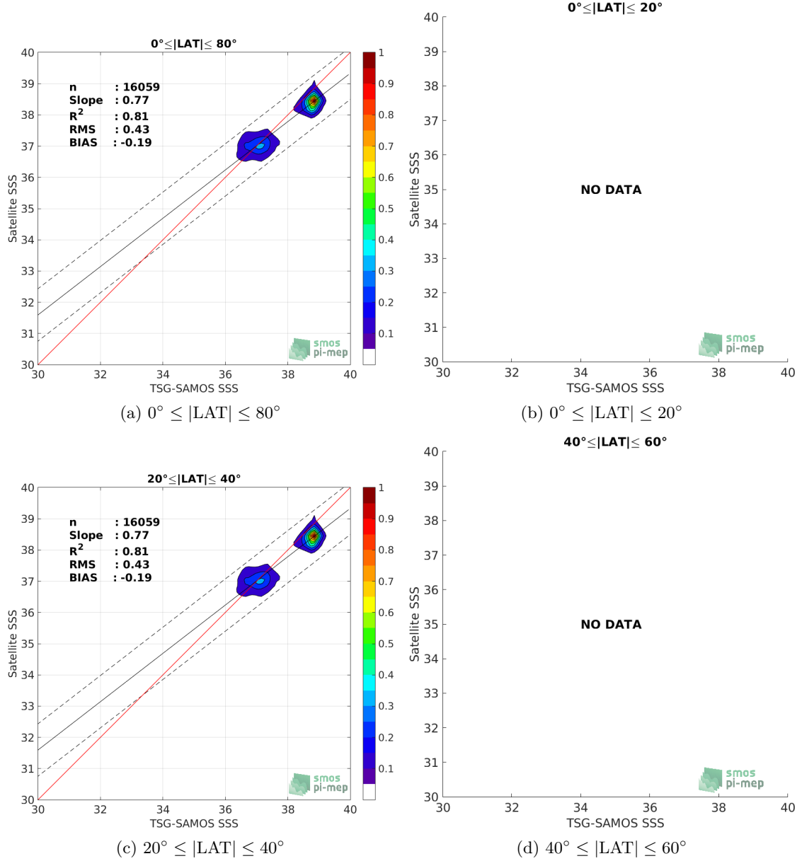
Figure 9: Contour maps of the concentration of SMOS-L3-BEC-MED-ATL-OA-V2-9DAYS-0.25DEG SSS (y-axis) versus TSG-SAMOS SSS (x-axis) at match-up pairs for different latitude bands. For each plot, the red line shows x=y . The black thin and dashed lines indicate a linear fit through the data cloud and the \pm 95\% confidence levels, respectively. The number match-up pairs n , the slope and R^2 coefficient of the linear fit, the root mean square (RMS) and the mean bias between satellite and in situ data are indicated for each latitude band in each plots.
