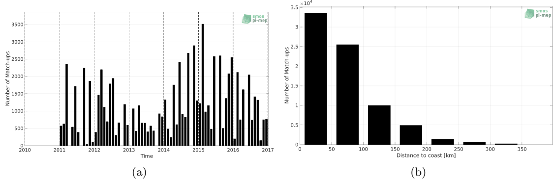
Figure 1: Number of match-ups between TSG (LEGOS-DM) and SMOS SSS L3 MED-ATL-OA v2 - 9 Days (BEC) SSS as a function of time (a) and as function of the distance to coast (b) over the Mediterranean Sea Pi-MEP region and for the full satellite product period.
