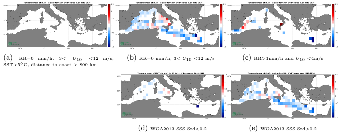
Figure 12: Temporal mean gridded over spatial boxes of size 1^\circ \times 1^\circ of \Delta SSS (SMOS SSS L3 MED-ATL-OA v2 - 9 Days (BEC) - TSG (LEGOS-DM)) for 5 different subdatasets corresponding to:RR=0 mm/h, 3 < U_{10} < 12 m/s, SST >5^\circ\text{C} , distance to coast > 800 km (a), RR=0 mm/h, 3 < U_{10} < 12 m/s (b), RR >1 mm/h and U_{10} < 4 m/s (c), WOA2013 SSS Std <0.2 (d), WOA2013 SSS Std >0.2 (e).
