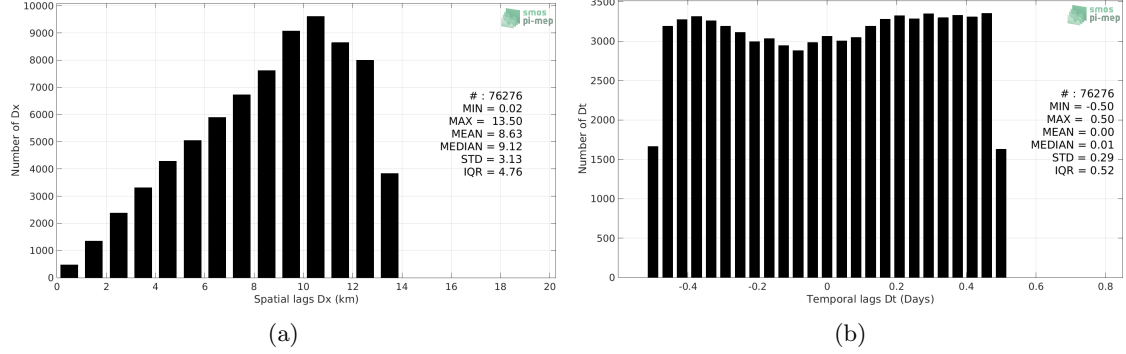
Figure 5: Histograms of the spatial (a) and temporal (b) lags between the time of the TSG (LEGOS-DM) measurements and the date of the corresponding SMOS SSS L3 MED-ATL-OA v2 - 9 Days (BEC) SSS product.
