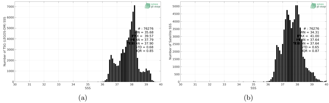
Figure 2: Histograms of SSS from TSG (LEGOS-DM) (a) and SMOS SSS L3 MED-ATL-OA v2 - 9 Days (BEC) (b) considering all match-up pairs per bins of 0.1 over the Mediterranean Sea Pi-MEP region and for the full satellite product period.
