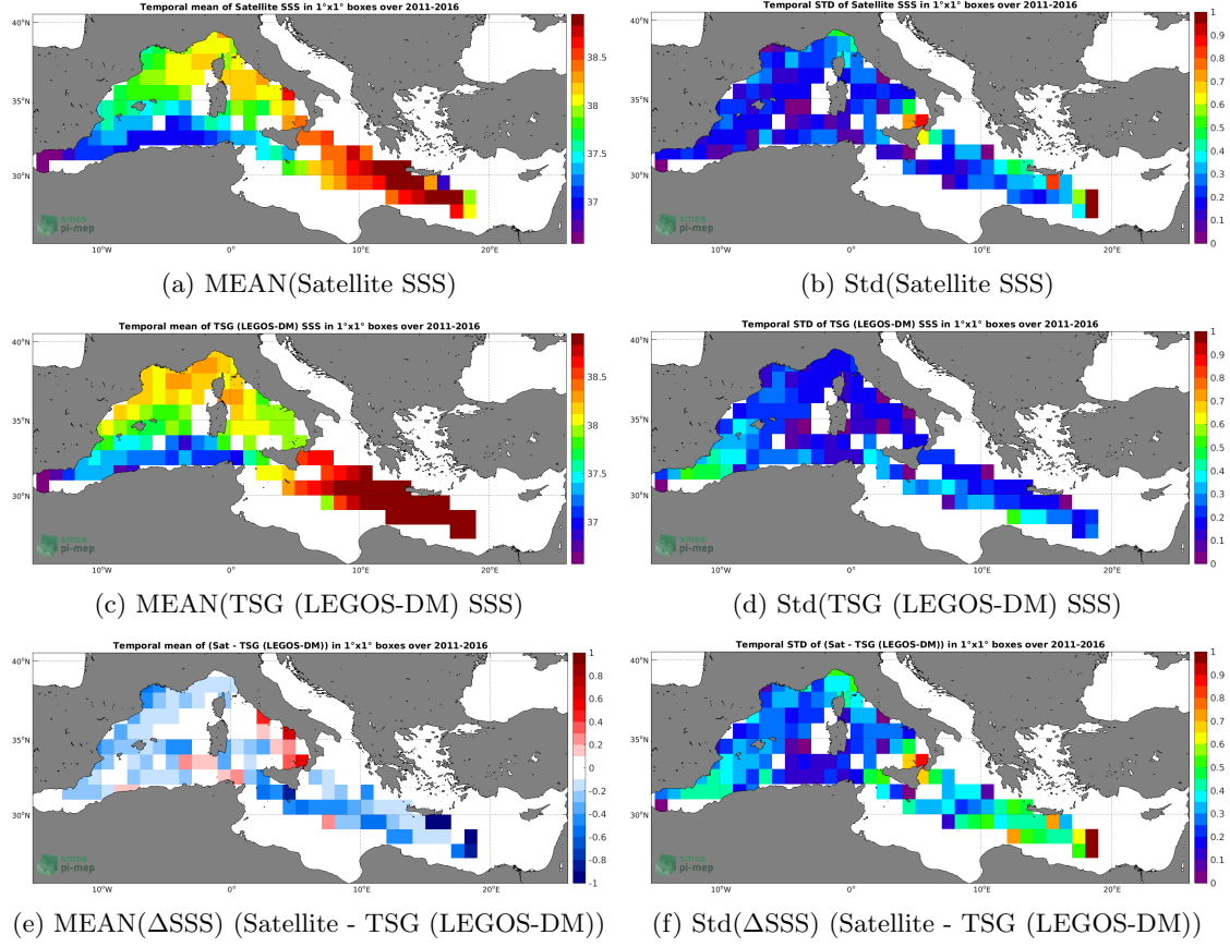
Figure 6: Temporal mean (left) and Std (right) of SSS from SMOS SSS L3 MED-ATL-OA v2 - 9 Days (BEC) (top), TSG (LEGOS-DM) (middle), and of \Delta SSS (Satellite - TSG (LEGOS-DM)). Only match-up pairs are used to generate these maps.
