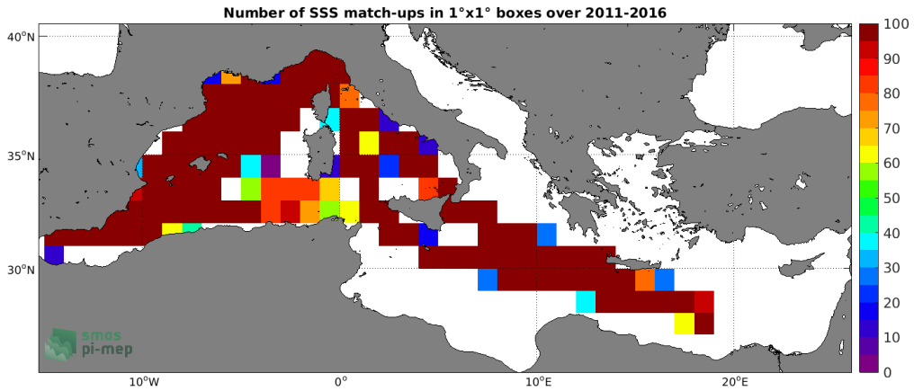
Figure 4: Number of SSS match-ups between TSG (LEGOS-DM) SSS and the SMOS SSS L3 MED-ATL-OA v2 - 9 Days (BEC) SSS product for the Mediterranean Sea Pi-MEP region over 1°x1° boxes and for the full satellite product period.
