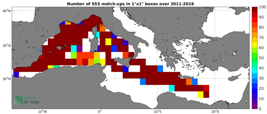
Figure 4: Number of SSS match-ups between TSG-LEGOS-DM SSS and the SMOS L3 MED-ATL-OA v2 - 9 Days (BEC) SSS product for the Mediterranean Sea Pi-MEP region over 1°x1° boxes and for the full satellite product period.
