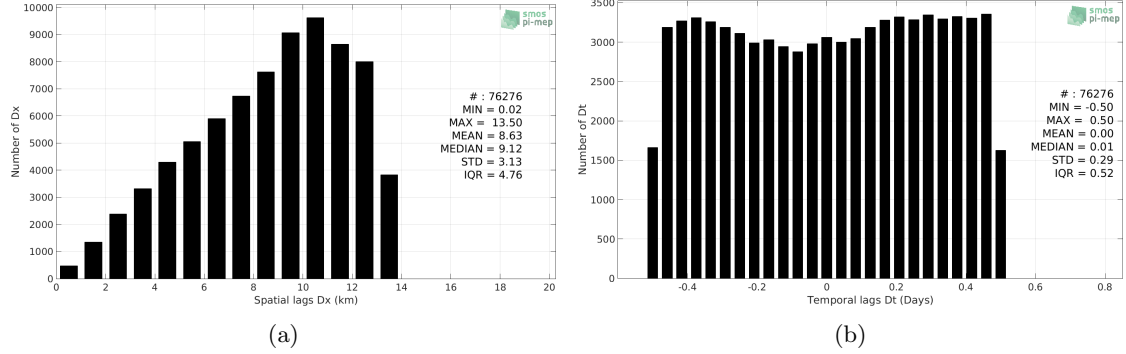
Figure 5: Histograms of the spatial (a) and temporal (b) lags between the time of the TSG-LEGOS-DM measurements and the date of the corresponding SMOS L3 MED-ATL-OA v2 - 9 Days (BEC) SSS product.
