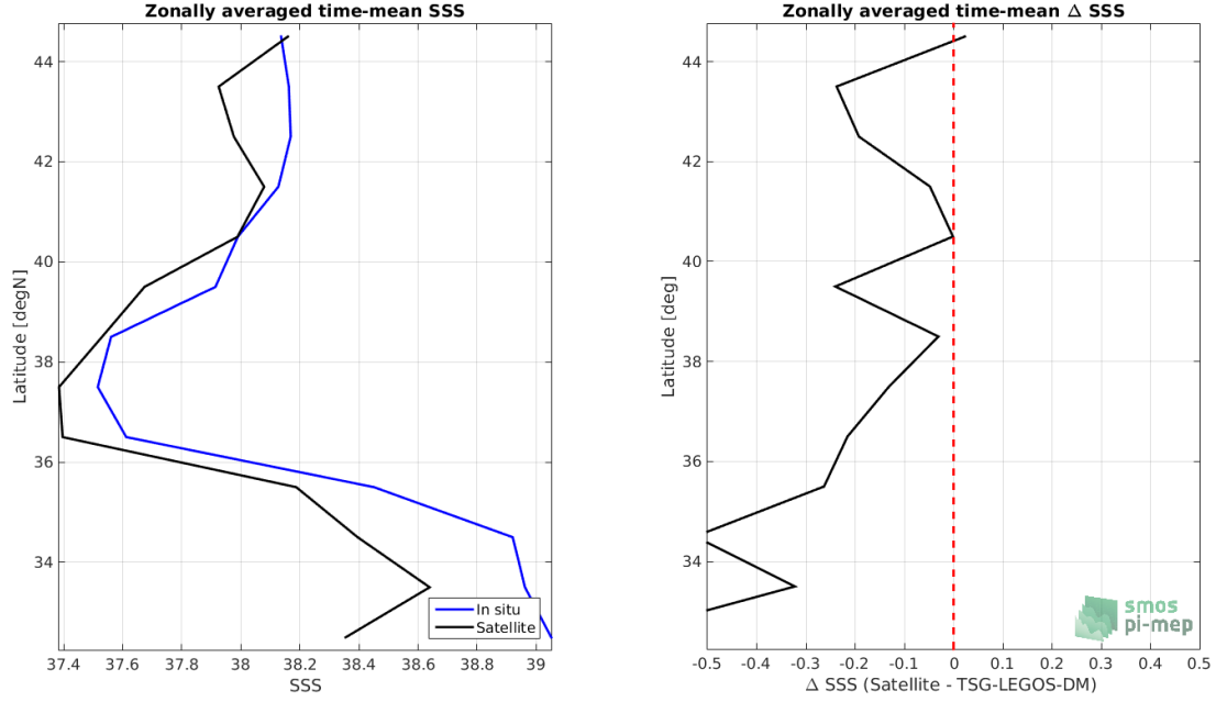
Figure 8: Left panel: Zonal mean SSS from SMOS L3 MED-ATL-OA v2 - 9 Days (BEC) satellite product (black) and from TSG-LEGOS-DM (blue). Right panel: Zonal mean of \Delta SSS (Satellite - TSG-LEGOS-DM) for all the collected Pi-MEP match-up pairs estimated over the full satellite product period.
