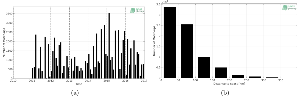
Figure 1: Number of match-ups between TSG-LEGOS-DM and SMOS L3 MED-ATL-OA v2 - 9 Days (BEC) SSS as a function of time (a) and as function of the distance to coast (b) over the Mediterranean Sea Pi-MEP region and for the full satellite product period.
