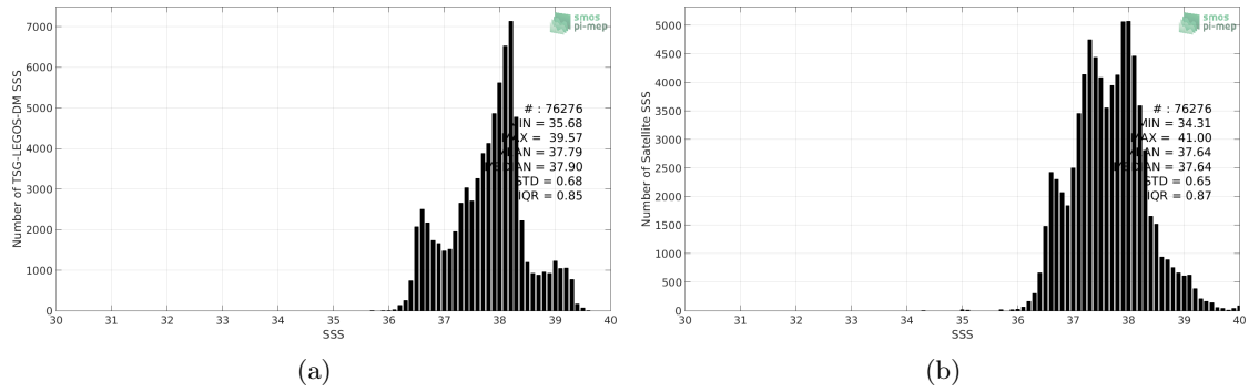
Figure 2: Histograms of SSS from TSG-LEGOS-DM (a) and SMOS L3 MED-ATL-OA v2 - 9 Days (BEC) (b) considering all match-up pairs per bins of 0.1 over the Mediterranean Sea Pi-MEP region and for the full satellite product period.
