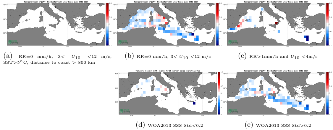
Figure 12: Temporal mean gridded over spatial boxes of size 1^\circ \times 1^\circ of \Delta SSS (SMOS L3 MED-ATL-OA v2 - 9 Days (BEC) - TSG-LEGOS-DM) for 5 different subdatasets corresponding to: RR=0 mm/h, 3 < U_{10} < 12 m/s, SST > 5^\circ C , distance to coast > 800 km (a), RR=0 mm/h, 3 < U_{10} < 12 m/s (b), RR > 1 mm/h and U_{10} < 4 m/s (c), WOA2013 SSS Std < 0.2 (d), WOA2013 SSS Std > 0.2 (e).
