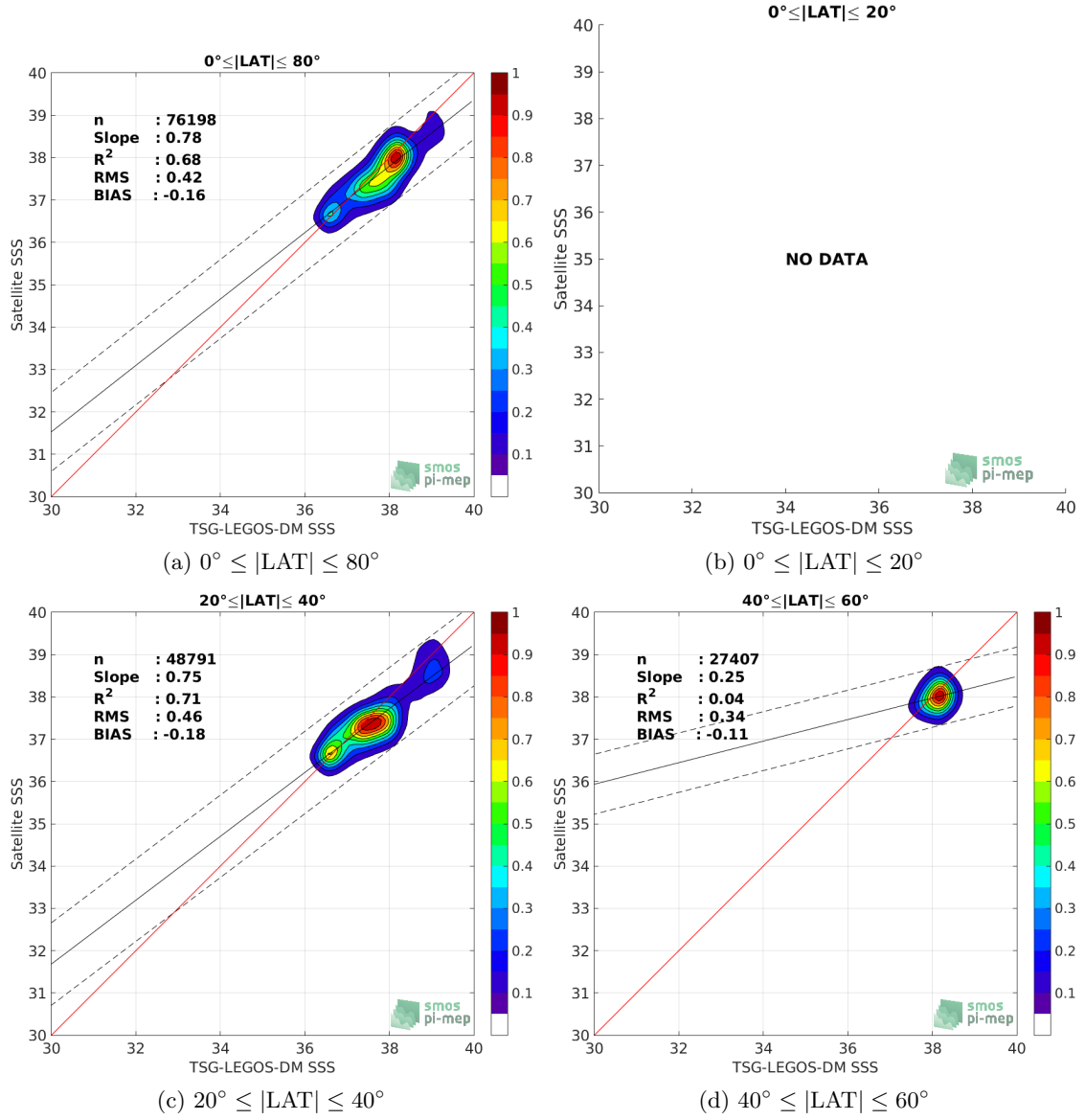
Figure 9: Contour maps of the concentration of SMOS L3 MED-ATL-OA v2 - 9 Days (BEC) SSS (y-axis) versus TSG-LEGOS-DM SSS (x-axis) at match-up pairs for different latitude bands. For each plot, the red line shows x=y . The black thin and dashed lines indicate a linear fit through the data cloud and the \pm 95\% confidence levels, respectively. The number match-up pairs n , the slope and R^2 coefficient of the linear fit, the root mean square (RMS) and the mean bias between satellite and in situ data are indicated for each latitude band in each plots.
