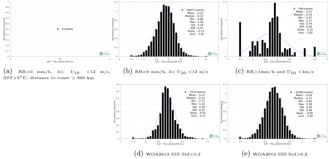
Figure 13: Normalized histogram of \Delta SSS (SMOS L3 MED-ATL-OA v2 - 9 Days (BEC) - TSG-LEGOS-DM) for 5 different subdatasets corresponding to: RR=0 mm/h, 3 < U_{10} < 12 m/s, SST>5°C, distance to coast > 800 km (a), RR=0 mm/h, 3 < U_{10} < 12 m/s (b), RR>1mm/h and U_{10} < 4 m/s (c), WOA2013 SSS Std<0.2 (d), WOA2013 SSS Std>0.2 (e).
