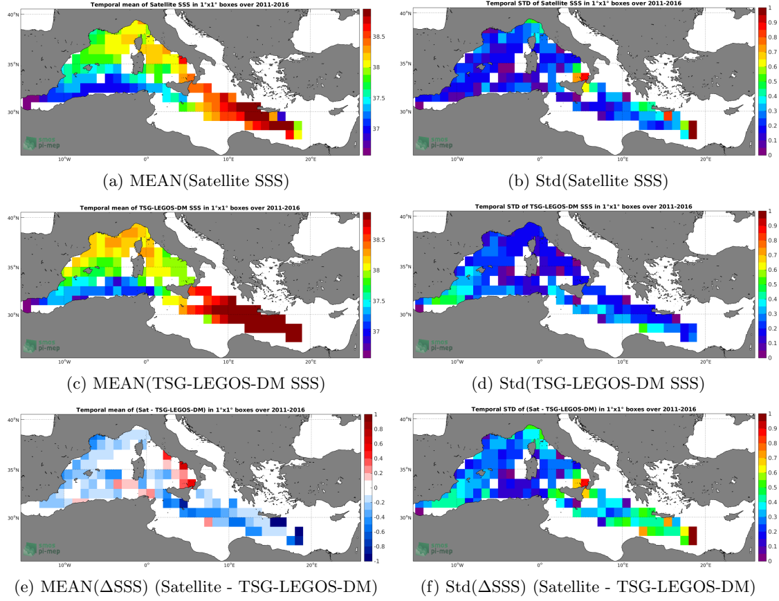
Figure 6: Temporal mean (left) and Std (right) of SSS from SMOS L3 MED-ATL-OA v2 - 9 Days (BEC) (top), TSG-LEGOS-DM (middle), and of \Delta SSS (Satellite - TSG-LEGOS-DM). Only match-up pairs are used to generate these maps.
