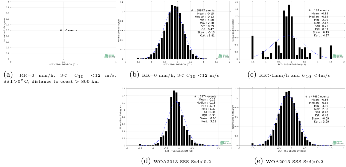
Figure 13: Normalized histogram of \Delta\text{SSS} (SMOS-L3-BEC-MED-ATL-OA-V2-9DAYS-0.25DEG - TSG-LEGOS-DM) for 5 different subdatasets corresponding to: RR=0 mm/h, 3 < U_{10} < 12 m/s, SST > 5^\circ\text{C} , distance to coast > 800 km (a), RR=0 mm/h, 3 < U_{10} < 12 m/s (b), RR > 1 mm/h and U_{10} < 4 m/s (c), WOA2013 SSS Std < 0.2 (d), WOA2013 SSS Std > 0.2 (e).
