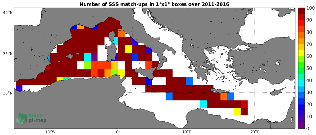
Figure 4: Number of SSS match-ups between TSG-LEGOS-DM SSS and the SMOS-L3-BEC-MED-ATL-OA-V2-9DAYS-0.25DEG SSS product for the Mediterranean Sea Pi-MEP region over 1^\circ \times 1^\circ boxes and for the full satellite product period.
