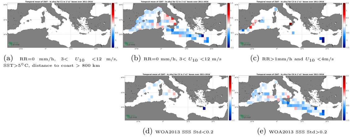
Figure 12: Temporal mean gridded over spatial boxes of size 1^\circ \times 1^\circ of \Delta SSS (SMOS-L3-BEC-MED-ATL-OA-V2-9DAYS-0.25DEG - TSG-LEGOS-DM) for 5 different subdatasets corresponding to: RR=0 mm/h, 3 < U_{10} < 12 m/s, SST > 5^\circ C , distance to coast > 800 km (a), RR=0 mm/h, 3 < U_{10} < 12 m/s (b), RR > 1 mm/h and U_{10} < 4 m/s (c), WOA2013 SSS Std < 0.2 (d), WOA2013 SSS Std > 0.2 (e).
