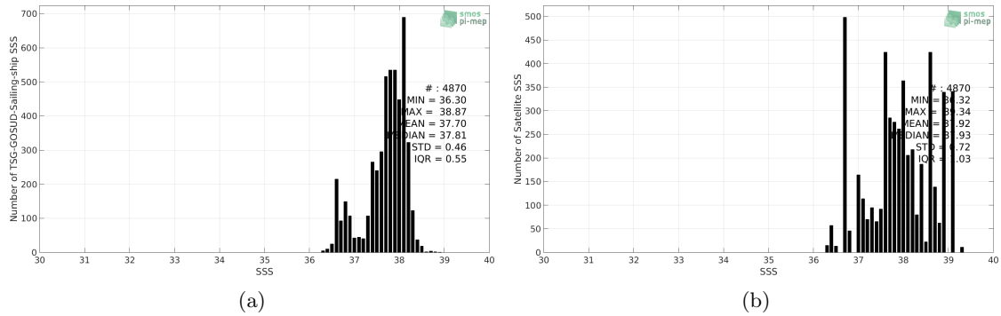
Figure 2: Histograms of SSS from TSG-GOSUD-Sailing-ship (a) and SMOS L3 MED-ATL-OA v2 - 9 Days (BEC) (b) considering all match-up pairs per bins of 0.1 over the Mediterranean Sea Pi-MEP region and for the full satellite product period.
