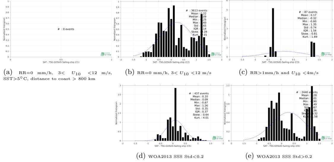
Figure 13: Normalized histogram of \Delta SSS (SMOS L3 MED-ATL-OA v2 - 9 Days (BEC) - TSG-GOSUD-Sailing-ship) for 5 different subdatasets corresponding to: RR=0 mm/h, 3 < U_{10} < 12 m/s, SST>5°C, distance to coast > 800 km (a), RR=0 mm/h, 3 < U_{10} < 12 m/s (b), RR>1 mm/h and U_{10} < 4 m/s (c), WOA2013 SSS Std<0.2 (d), WOA2013 SSS Std>0.2 (e).
