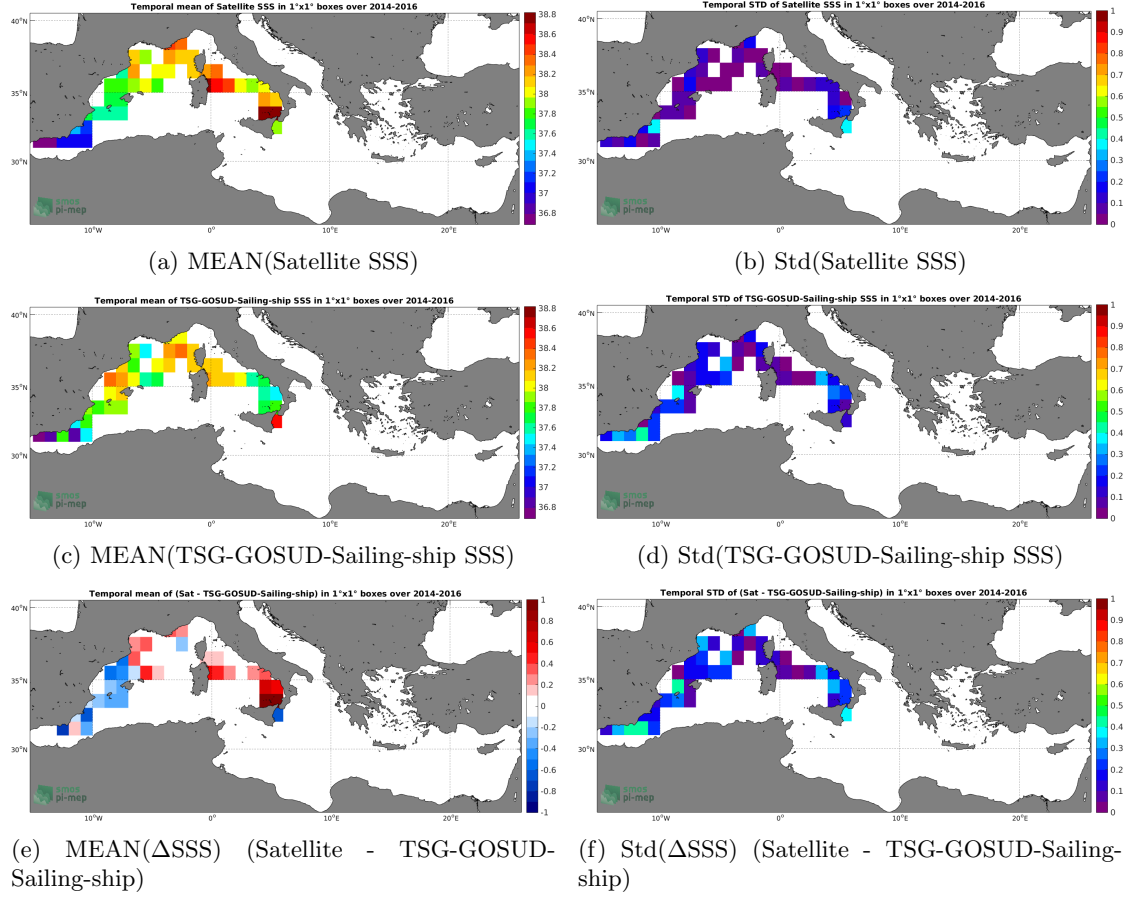
Figure 6: Temporal mean (left) and Std (right) of SSS from SMOS L3 MED-ATL-OA v2 - 9 Days (BEC) (top), TSG-GOSUD-Sailing-ship (middle), and of \Delta SSS (Satellite - TSG-GOSUD-Sailing-ship). Only match-up pairs are used to generate these maps.
