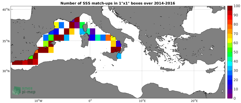
Figure 4: Number of SSS match-ups between TSG-GOSUD-Sailing-ship SSS and the SMOS L3 MED-ATL-OA v2 - 9 Days (BEC) SSS product for the Mediterranean Sea Pi-MEP region over 1°x1° boxes and for the full satellite product period.
