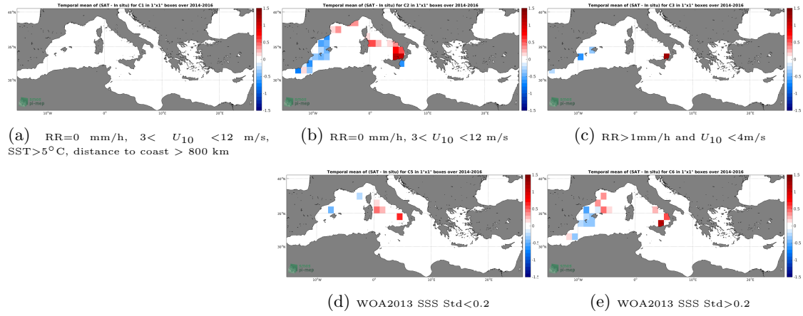
Figure 12: Temporal mean gridded over spatial boxes of size 1^\circ \times 1^\circ of \Delta SSS (SMOS L3 MED-ATL-OA v2 - 9 Days (BEC) - TSG-GOSUD-Sailing-ship) for 5 different subdatasets corresponding to: RR=0 mm/h, 3 < U_{10} < 12 m/s, SST >5^\circ\text{C} , distance to coast > 800 km (a), RR=0 mm/h, 3 < U_{10} < 12 m/s (b), RR >1 mm/h and U_{10} < 4 m/s (c), WOA2013 SSS Std <0.2 (d), WOA2013 SSS Std >0.2 (e).
