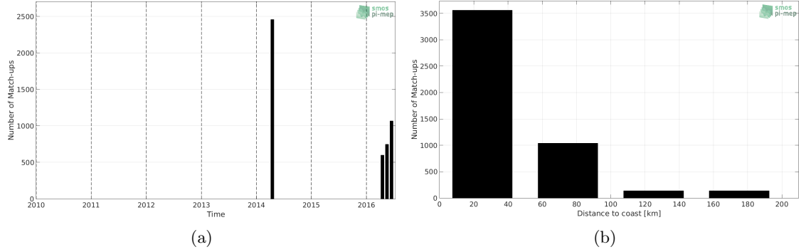
Figure 1: Number of match-ups between TSG-GOSUD-Sailing-ship and SMOS L3 MED-ATL-OA v2 - 9 Days (BEC) SSS as a function of time (a) and as function of the distance to coast (b) over the Mediterranean Sea Pi-MEP region and for the full satellite product period.
