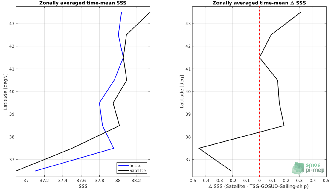
Figure 8: Left panel: Zonal mean SSS from SMOS L3 MED-ATL-OA v2 - 9 Days (BEC) satellite product (black) and from TSG-GOSUD-Sailing-ship (blue). Right panel: Zonal mean of \Delta SSS (Satellite - TSG-GOSUD-Sailing-ship) for all the collected Pi-MEP match-up pairs estimated over the full satellite product period.
