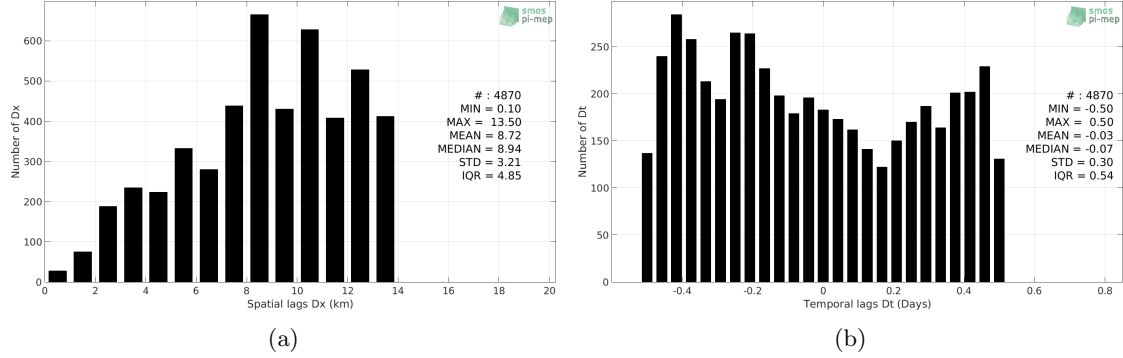
Figure 5: Histograms of the spatial (a) and temporal (b) lags between the time of the TSG-GOSUD-Sailing-ship measurements and the date of the corresponding SMOS L3 MED-ATL-OA v2 - 9 Days (BEC) SSS product.
