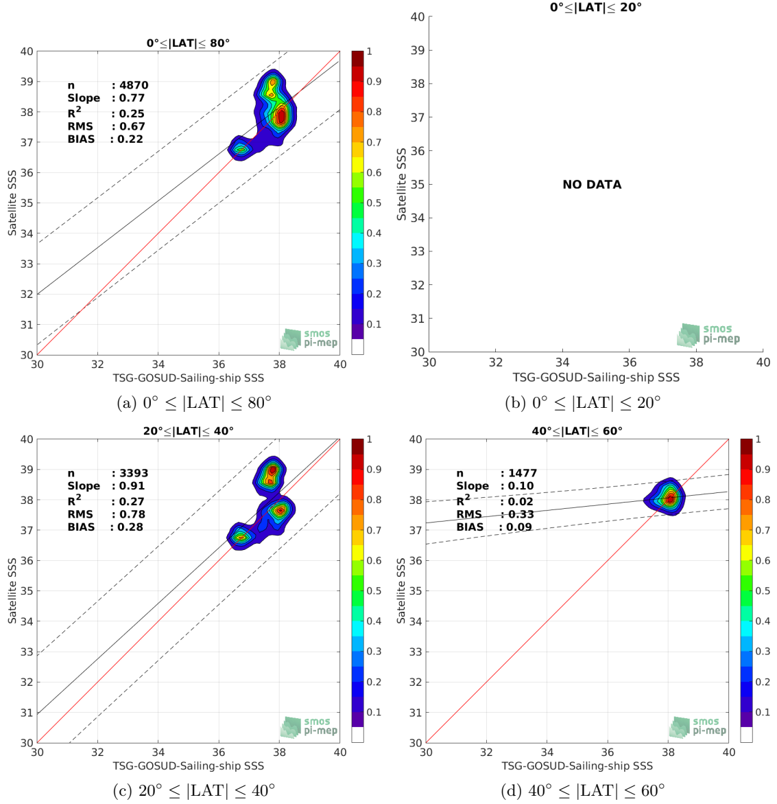
Figure 9: Contour maps of the concentration of SMOS L3 MED-ATL-OA v2 - 9 Days (BEC) SSS (y-axis) versus TSG-GOSUD-Sailing-ship SSS (x-axis) at match-up pairs for different latitude bands. For each plot, the red line shows x=y . The black thin and dashed lines indicate a linear fit through the data cloud and the \pm 95\% confidence levels, respectively. The number match-up pairs n , the slope and R^2 coefficient of the linear fit, the root mean square (RMS) and the mean bias between satellite and in situ data are indicated for each latitude band in each plots.
