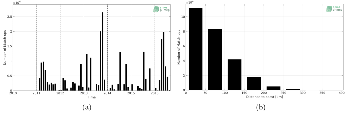
Figure 1: Number of match-ups between TSG-GOSUD-Research-vessel and SMOS-L3-BEC-MED-ATL-OA-V2-9DAYS-0.25DEG SSS as a function of time (a) and as function of the distance to coast (b) over the Mediterranean Sea Pi-MEP region and for the full satellite product period.
