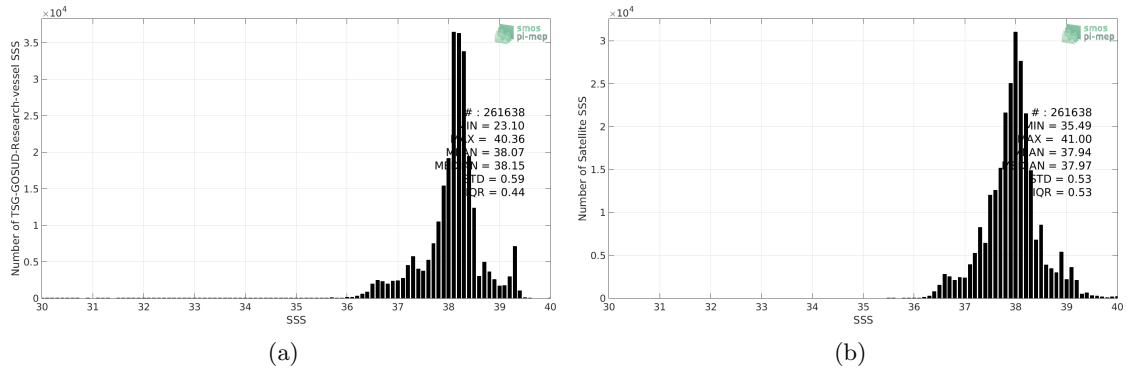
Figure 2: Histograms of SSS from TSG-GOSUD-Research-vessel (a) and SMOS-L3-BEC-MED-ATL-OA-V2-9DAYS-0.25DEG (b) considering all match-up pairs per bins of 0.1 over the Mediterranean Sea Pi-MEP region and for the full satellite product period.
