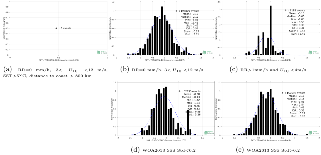
Figure 13: Normalized histogram of \Delta\text{SSS} (SMOS-L3-BEC-MED-ATL-OA-V2-9DAYS-0.25DEG - TSG-GOSUD-Research-vessel) for 5 different subdatasets corresponding to: RR=0 mm/h, 3 < U_{10} < 12 m/s, SST > 5^\circ\text{C} , distance to coast > 800 km (a), RR=0 mm/h, 3 < U_{10} < 12 m/s (b), RR > 1\text{mm/h} and U_{10} < 4\text{m/s} (c), WOA2013 SSS Std < 0.2 (d), WOA2013 SSS Std > 0.2 (e).
