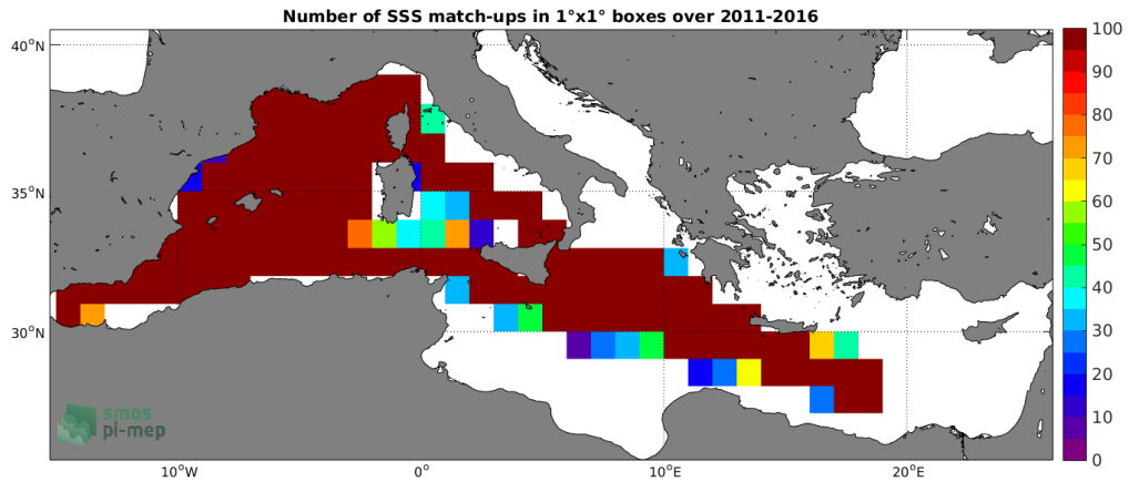
Figure 4: Number of SSS match-ups between TSG-GOSUD-Research-vessel SSS and the SMOS-L3-BEC-MED-ATL-OA-V2-9DAYS-0.25DEG SSS product for the Mediterranean Sea Pi-MEP region over 1^\circ \times 1^\circ boxes and for the full satellite product period.
