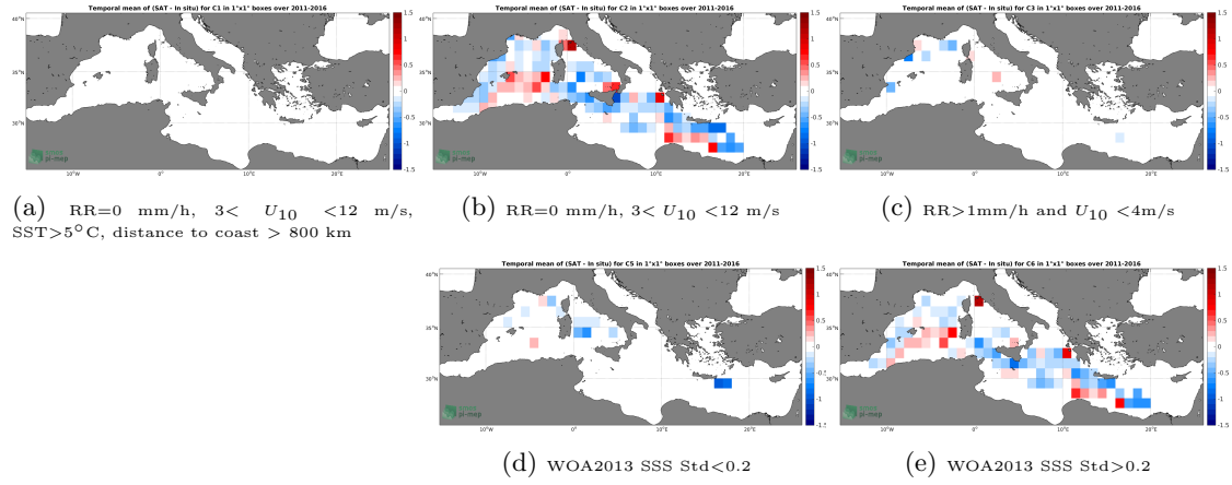
Figure 12: Temporal mean gridded over spatial boxes of size 1^\circ \times 1^\circ of \Delta SSS (SMOS-L3-BEC-MED-ATL-OA-V2-9DAYS-0.25DEG - TSG-GOSUD-Research-vessel) for 5 different subdatasets corresponding to: RR=0 mm/h, 3 < U_{10} < 12 m/s, SST >5^\circ\text{C} , distance to coast > 800 km (a), RR=0 mm/h, 3 < U_{10} < 12 m/s (b), RR >1 mm/h and U_{10} < 4 m/s (c), WOA2013 SSS Std <0.2 (d), WOA2013 SSS Std >0.2 (e).
