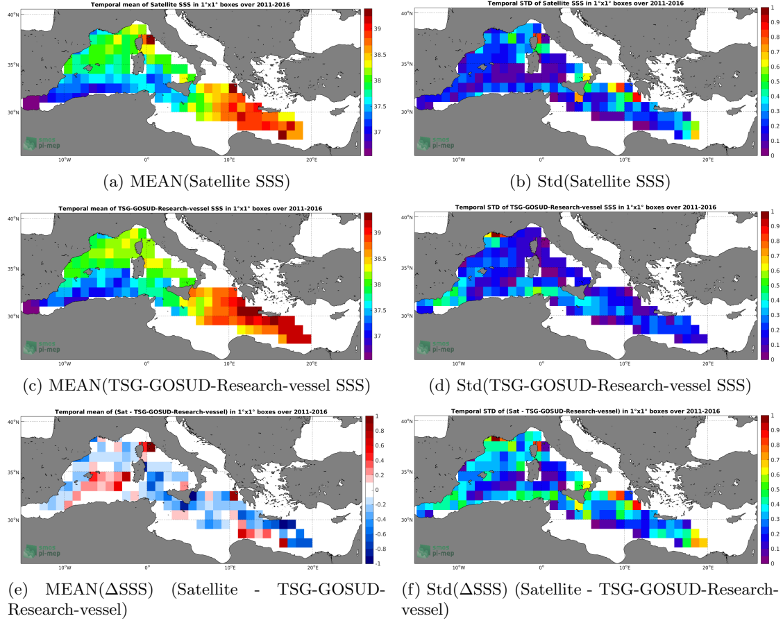
Figure 6: Temporal mean (left) and Std (right) of SSS from SMOS-L3-BEC-MED-ATL-OA-V2-9DAYS-0.25DEG (top), TSG-GOSUD-Research-vessel (middle), and of \Delta SSS (Satellite - TSG-GOSUD-Research-vessel). Only match-up pairs are used to generate these maps.
