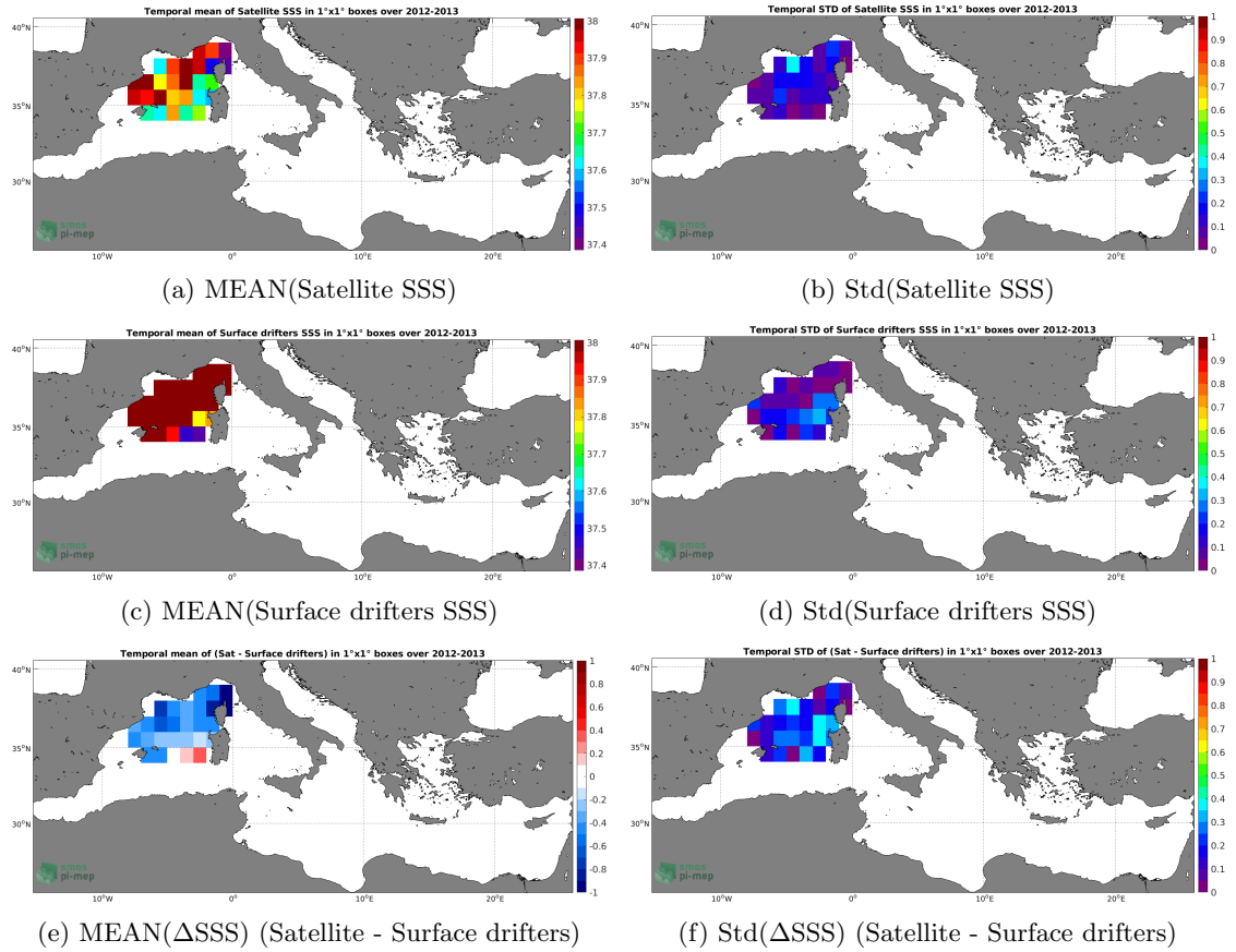
Figure 5: Temporal mean (left) and Std (right) of SSS from SMOS SSS L3 MED-ATL-OA v2 - 9 Days (BEC) (top), Surface drifters (middle), and of \Delta SSS (Satellite - Surface drifters). Only match-up pairs are used to generate these maps.
