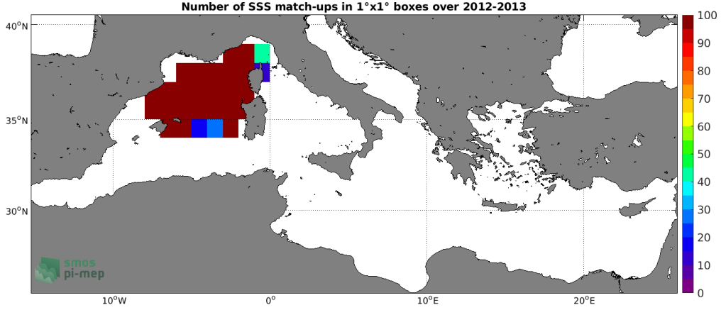
Figure 3: Number of SSS match-ups between Surface drifters SSS and the SMOS SSS L3 MED-ATL-OA v2 - 9 Days (BEC) SSS product for the Mediterranean Sea Pi-MEP region over 1^\circ \times 1^\circ boxes and for the full satellite product period.
