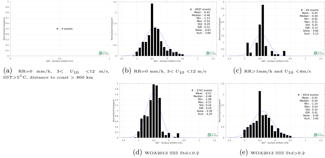
Figure 12: Normalized histogram of \Delta SSS (SMOS SSS L3 MED-ATL-OA v2 - 9 Days (BEC) - Surface drifters) for 5 different subdatasets corresponding to: RR=0 mm/h, 3 < U_{10} < 12 m/s, SST>5°C, distance to coast > 800 km (a), RR=0 mm/h, 3 < U_{10} < 12 m/s (b), RR>1mm/h and U_{10} < 4 m/s (c), WOA2013 SSS Std<0.2 (d), WOA2013 SSS Std>0.2 (e).
