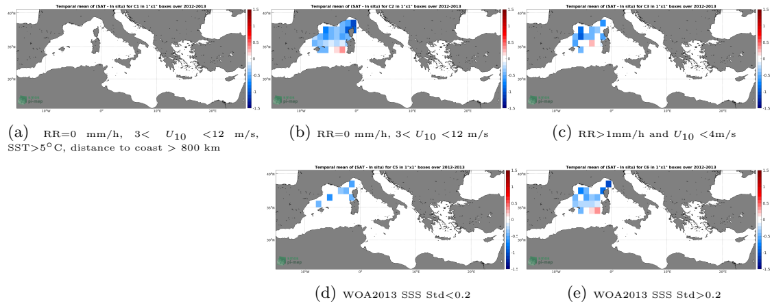
Figure 11: Temporal mean gridded over spatial boxes of size 1^\circ \times 1^\circ of \Delta SSS (SMOS SSS L3 MED-ATL-OA v2 - 9 Days (BEC) - Surface drifters) for 5 different subdatasets corresponding to: RR=0 mm/h, 3 < U_{10} < 12 m/s, SST > 5^\circ C , distance to coast > 800 km (a), RR=0 mm/h, 3 < U_{10} < 12 m/s (b), RR > 1 mm/h and U_{10} < 4 m/s (c), WOA2013 SSS Std < 0.2 (d), WOA2013 SSS Std > 0.2 (e).
