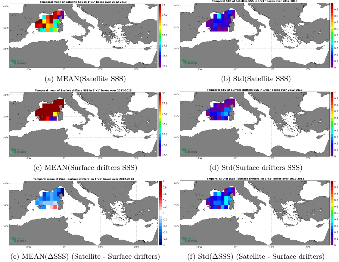
Figure 5: Temporal mean (left) and Std (right) of SSS from SMOS SSS L3 MED-ATL-OA v2 - 9 Days (BEC) (top), Surface drifters (middle), and of \Delta\text{SSS} (Satellite - Surface drifters). Only match-up pairs are used to generate these maps.
