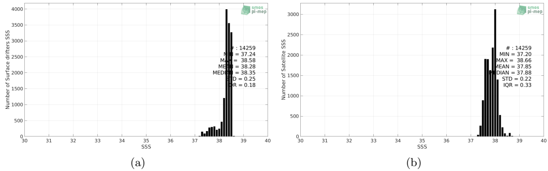
Figure 2: Histograms of SSS from Surface drifters (a) and SMOS SSS L3 MED-ATL-OA v2 - 9 Days (BEC) (b) considering all match-up pairs per bins of 0.1 over the Mediterranean Sea Pi-MEP region and for the full satellite product period.
