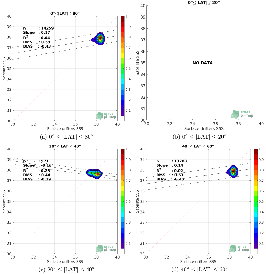
Figure 8: Contour maps of the concentration of SMOS SSS L3 MED-ATL-OA v2 - 9 Days (BEC) SSS (y-axis) versus Surface drifters SSS (x-axis) at match-up pairs for different latitude bands. For each plot, the red line shows x=y . The black thin and dashed lines indicate a linear fit through the data cloud and the \pm 95\% confidence levels, respectively. The number match-up pairs n , the slope and R^2 coefficient of the linear fit, the root mean square (RMS) and the mean bias between satellite and in situ data are indicated for each latitude band in each plots.
