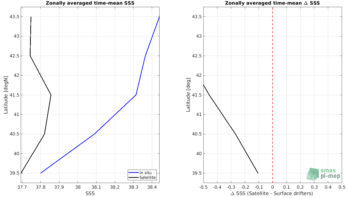
Figure 7: Left panel: Zonal mean SSS from SMOS SSS L3 MED-ATL-OA v2 - 9 Days (BEC) satellite product (black) and from Surface drifters (blue). Right panel: Zonal mean of \Delta SSS (Satellite - Surface drifters) for all the collected Pi-MEP match-up pairs estimated over the full satellite product period.
