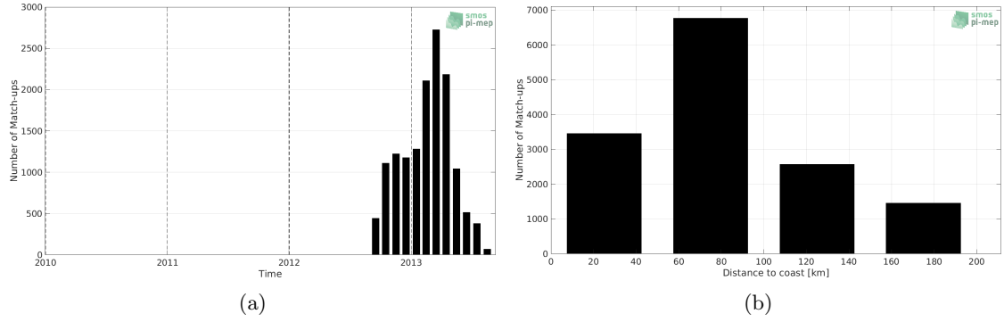
Figure 1: Number of match-ups between Surface drifters and SMOS SSS L3 MED-ATL-OA v2 - 9 Days (BEC) SSS as a function of time (a) and as function of the distance to coast (b) over the Mediterranean Sea Pi-MEP region and for the full satellite product period.
