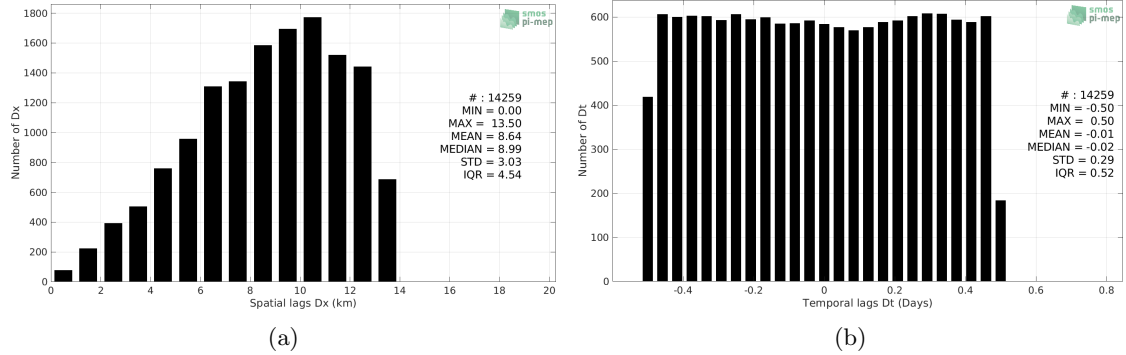
Figure 4: Histograms of the spatial (a) and temporal (b) lags between the location/time of the Surface drifters measurement and the date of the corresponding SMOS SSS L3 MED-ATL-OA v2 - 9 Days (BEC) SSS pixel.
