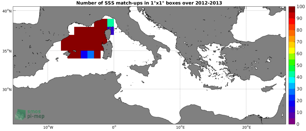
Figure 3: Number of SSS match-ups between Surface drifters SSS and the SMOS L3 MED-ATL-OA v2 - 9 Days (BEC) SSS product for the Mediterranean Sea Pi-MEP region over 1^\circ \times 1^\circ boxes and for the full satellite product period.
