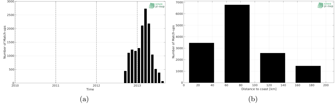
Figure 1: Number of match-ups between Surface drifters and SMOS L3 MED-ATL-OA v2 - 9 Days (BEC) SSS as a function of time (a) and as function of the distance to coast (b) over the Mediterranean Sea Pi-MEP region and for the full satellite product period.
