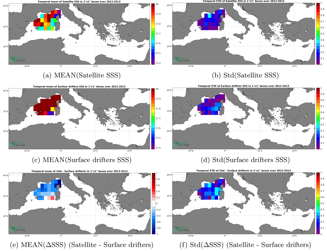
Figure 5: Temporal mean (left) and Std (right) of SSS from SMOS L3 MED-ATL-OA v2 - 9 Days (BEC) (top), Surface drifters (middle), and of \Delta SSS (Satellite - Surface drifters). Only match-up pairs are used to generate these maps.
