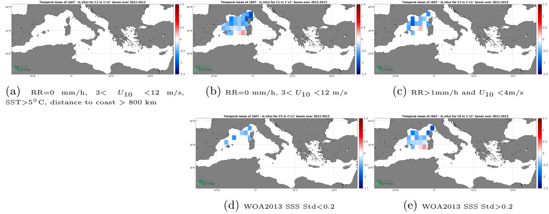
Figure 11: Temporal mean gridded over spatial boxes of size 1^\circ \times 1^\circ of \Delta SSS (SMOS L3 MED-ATL-OA v2 - 9 Days (BEC) - Surface drifters) for 5 different subdatasets corresponding to:RR=0 mm/h, 3 < U_{10} < 12 m/s, SST >5^\circ\text{C} , distance to coast > 800 km (a), RR=0 mm/h, 3 < U_{10} < 12 m/s (b), RR >1 mm/h and U_{10} < 4 m/s (c), WOA2013 SSS Std <0.2 (d), WOA2013 SSS Std >0.2 (e).
