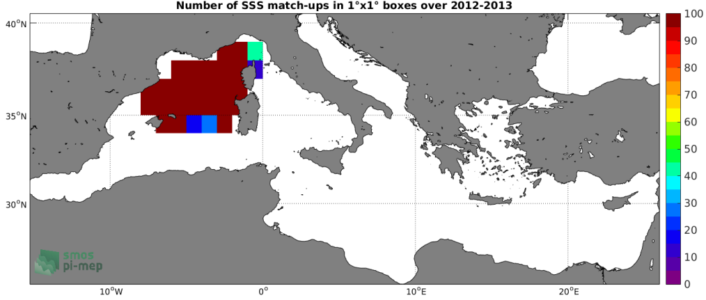
Figure 3: Number of SSS match-ups between Surface drifters SSS and the SMOS-L3-BEC-MED-ATL-OA-V2-9DAYS-0.25DEG SSS product for the Mediterranean Sea Pi-MEP region over 1°x1° boxes and for the full satellite product period.
