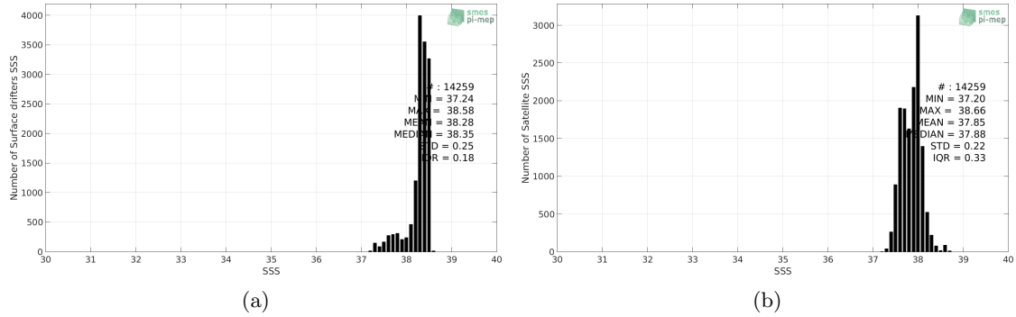
Figure 2: Histograms of SSS from Surface drifters (a) and SMOS-L3-BEC-MED-ATL-OA-V2-9DAYS-0.25DEG (b) considering all match-up pairs per bins of 0.1 over the Mediterranean Sea Pi-MEP region and for the full satellite product period.
