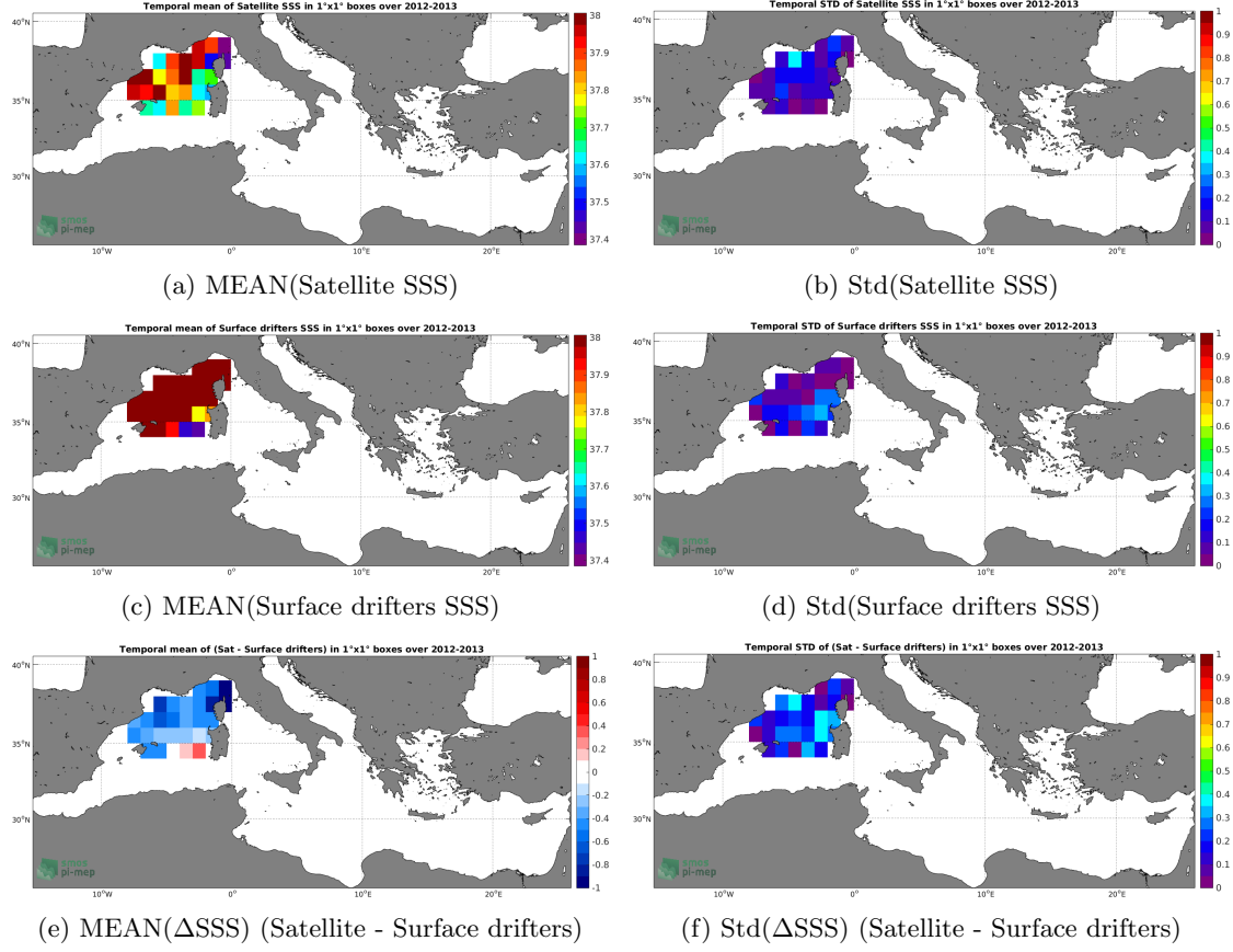
Figure 5: Temporal mean (left) and Std (right) of SSS from SMOS-L3-BEC-MED-ATL-OA-V2-9DAYS-0.25DEG (top), Surface drifters (middle), and of \Delta SSS (Satellite - Surface drifters). Only match-up pairs are used to generate these maps.
