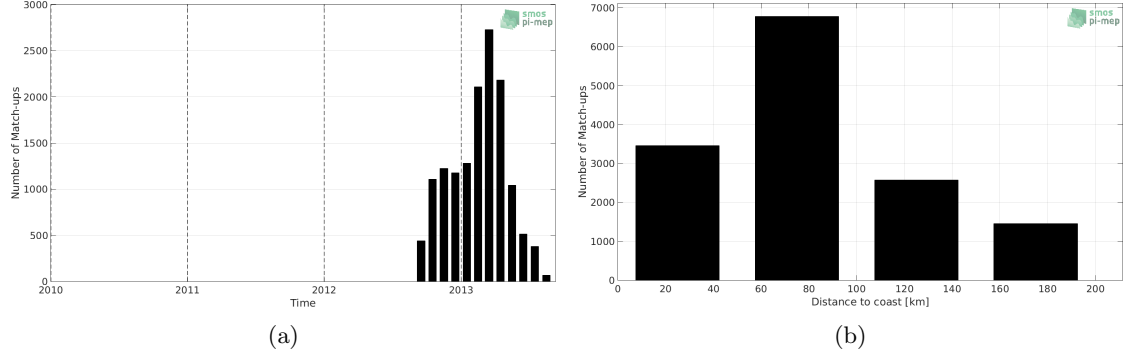
Figure 1: Number of match-ups between Surface drifters and SMOS-L3-BEC-MED-ATL-OA-V2-9DAYS-0.25DEG SSS as a function of time (a) and as function of the distance to coast (b) over the Mediterranean Sea Pi-MEP region and for the full satellite product period.
