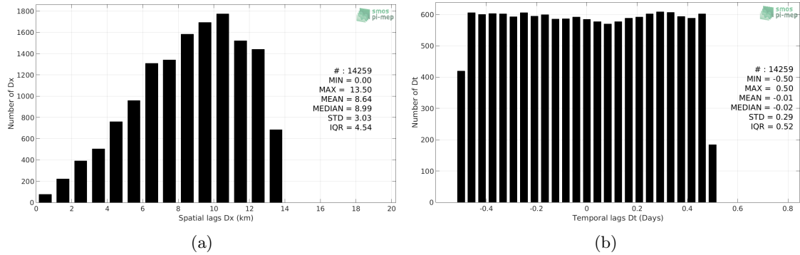
Figure 4: Histograms of the spatial (a) and temporal (b) lags between the time of the Surface drifters measurements and the date of the corresponding SMOS-L3-BEC-MED-ATL-OA-V2-9DAYS-0.25DEG SSS product.
