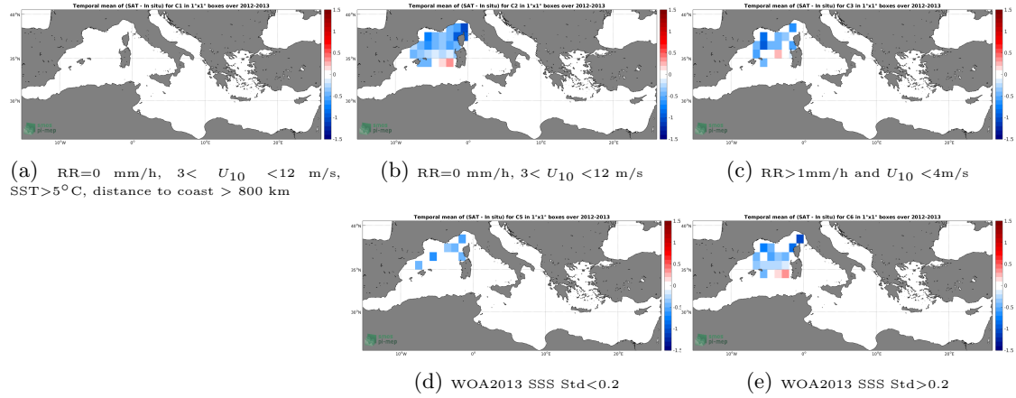
Figure 11: Temporal mean gridded over spatial boxes of size 1^\circ \times 1^\circ of \Delta SSS (SMOS-L3-BEC-MED-ATL-OA-V2-9DAYS-0.25DEG - Surface drifters) for 5 different subdatasets corresponding to: RR=0 mm/h, 3 < U_{10} < 12 m/s, SST >5^\circ\text{C} , distance to coast > 800 km (a), RR=0 mm/h, 3 < U_{10} < 12 m/s (b), RR >1 mm/h and U_{10} < 4 m/s (c), WOA2013 SSS Std <0.2 (d), WOA2013 SSS Std >0.2 (e).
