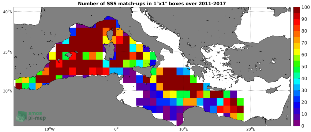
Figure 4: Number of SSS match-ups between Argo SSS and the SMOS SSS L3 MED-ATL-OA v2 - 9 Days (BEC) SSS product for the Mediterranean Sea Pi-MEP region over 1^\circ \times 1^\circ boxes and for the full satellite product period.
