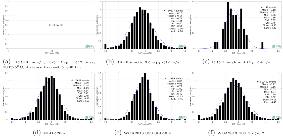
Figure 13: Normalized histogram of \Delta\text{SSS} (SMOS SSS L3 MED-ATL-OA v2 - 9 Days (BEC) - Argo) for 6 different subdatasets corresponding to: RR=0 mm/h, 3 < U_{10} < 12 m/s, SST>5°C, distance to coast > 800 km (a), RR=0 mm/h, 3 < U_{10} < 12 m/s (b), RR>1mm/h and U_{10} < 4 m/s (c), MLD<20m (d), WOA2013 SSS Std<0.2 (e), WOA2013 SSS Std>0.2 (f).
