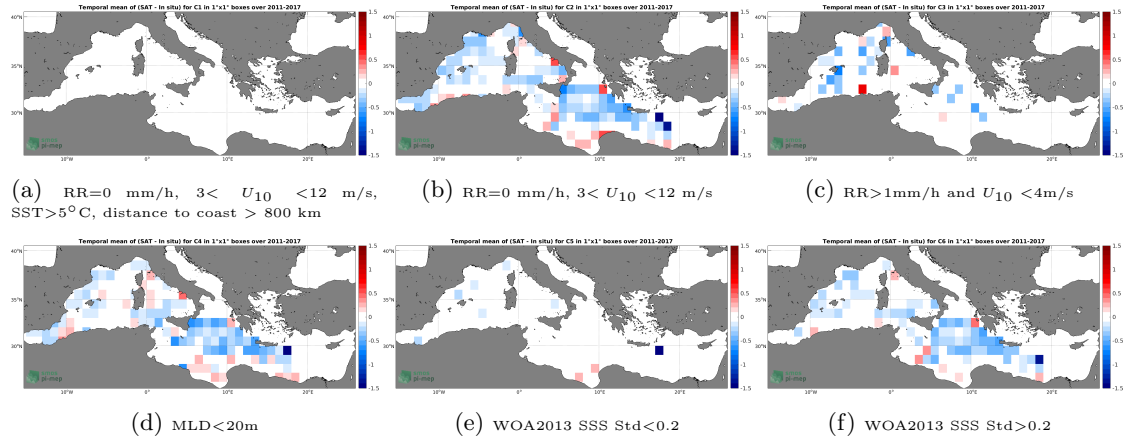
Figure 12: Temporal mean gridded over spatial boxes of size 1^\circ \times 1^\circ of \Delta SSS (SMOS SSS L3 MED-ATL-OA v2 - 9 Days (BEC) - Argo) for 6 different subdatasets corresponding to: RR=0 mm/h, 3 < U_{10} < 12 m/s, SST > 5^\circ C , distance to coast > 800 km (a), RR=0 mm/h, 3 < U_{10} < 12 m/s (b), RR > 1 mm/h and U_{10} < 4 m/s (c), MLD < 20 m (d), WOA2013 SSS Std < 0.2 (e), WOA2013 SSS Std > 0.2 (f).
