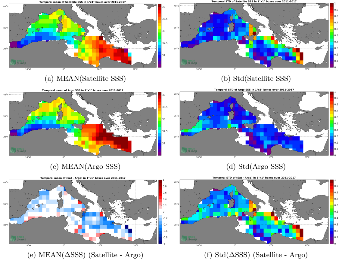
Figure 6: Temporal mean (left) and Std (right) of SSS from SMOS L3 MED-ATL-OA v2 - 9 Days (BEC) (top), Argo (middle), and of \Delta SSS (Satellite - Argo). Only match-up pairs are used to generate these maps.
