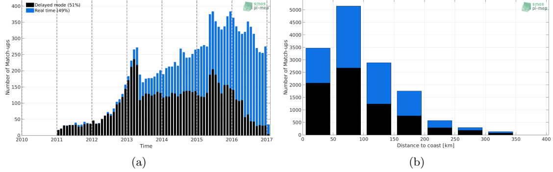
Figure 1: Number of match-ups between Argo and SMOS L3 MED-ATL-OA v2 - 9 Days (BEC) SSS as a function of time (a) and as function of the distance to coast (b) over the Mediterranean Sea Pi-MEP region and for the full satellite product period.
