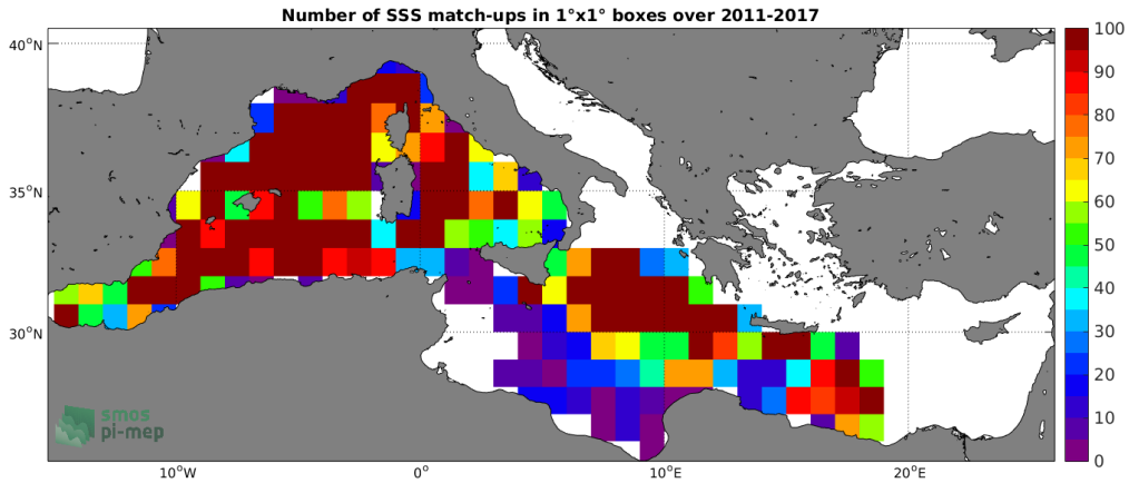
Figure 4: Number of SSS match-ups between Argo SSS and the SMOS L3 MED-ATL-OA v2 - 9 Days (BEC) SSS product for the Mediterranean Sea Pi-MEP region over 1°x1° boxes and for the full satellite product period.
