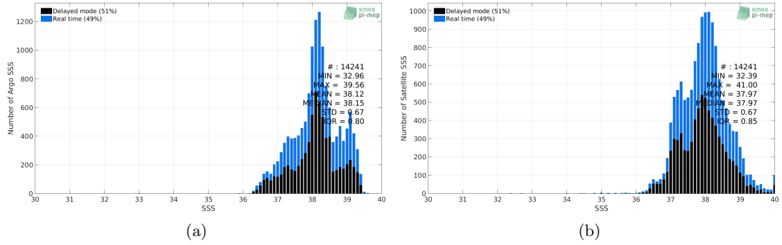
Figure 2: Histograms of SSS from Argo (a) and SMOS L3 MED-ATL-OA v2 - 9 Days (BEC) (b) considering all match-up pairs per bins of 0.1 over the Mediterranean Sea Pi-MEP region and for the full satellite product period.
