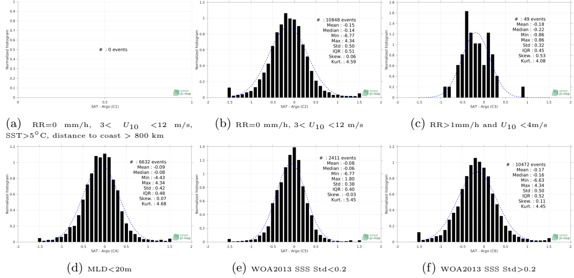
Figure 13: Normalized histogram of \Delta SSS (SMOS L3 MED-ATL-OA v2 - 9 Days (BEC) - Argo) for 6 different subdatasets corresponding to: RR=0 mm/h, 3 < U_{10} < 12 m/s, SST>5°C, distance to coast > 800 km (a), RR=0 mm/h, 3 < U_{10} < 12 m/s (b), RR>1mm/h and U_{10} < 4 m/s (c), MLD<20m (d), WOA2013 SSS Std<0.2 (e), WOA2013 SSS Std>0.2 (f).
