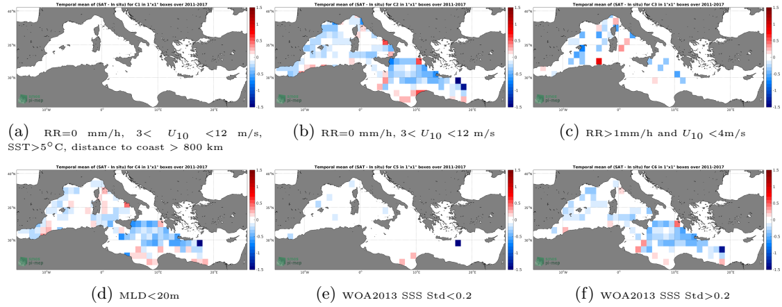
Figure 12: Temporal mean gridded over spatial boxes of size 1^\circ \times 1^\circ of \Delta SSS (SMOS L3 MED-ATL-OA v2 - 9 Days (BEC) - Argo) for 6 different subdatasets corresponding to: RR=0 mm/h, 3 < U_{10} < 12 m/s, SST > 5^\circ C , distance to coast > 800 km (a), RR=0 mm/h, 3 < U_{10} < 12 m/s (b), RR > 1 mm/h and U_{10} < 4 m/s (c), MLD < 20 m (d), WOA2013 SSS Std < 0.2 (e), WOA2013 SSS Std > 0.2 (f).
