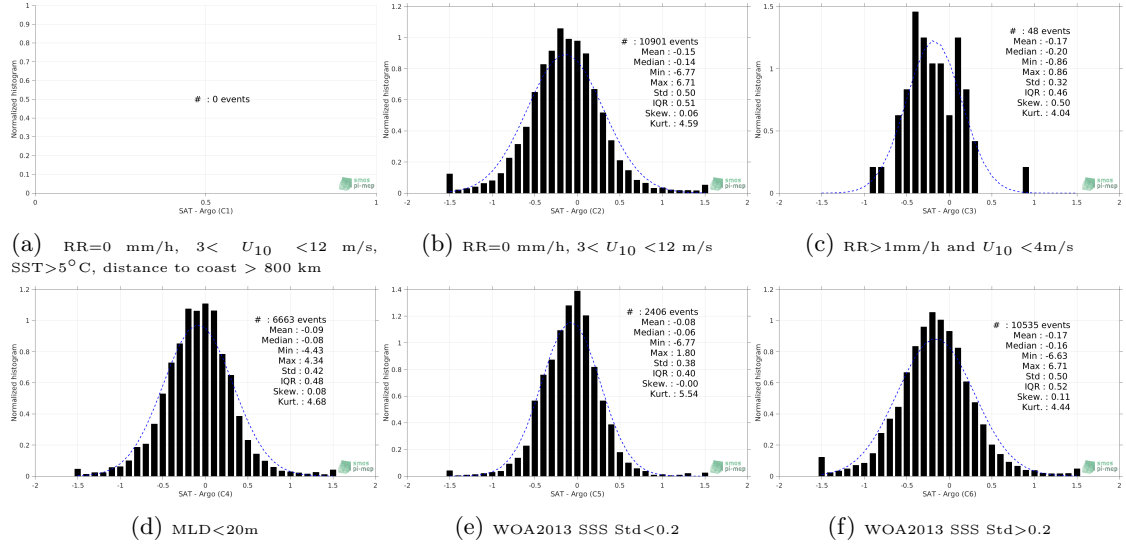
Figure 13: Normalized histogram of \Delta SSS (SMOS-L3-BEC-MED-ATL-OA-V2-9DAYS-0.25DEG - Argo) for 6 different subdatasets corresponding to: RR=0 mm/h, 3 < U_{10} < 12 m/s, SST>5°C, distance to coast > 800 km (a), RR=0 mm/h, 3 < U_{10} < 12 m/s (b), RR>1mm/h and U_{10} < 4 m/s (c), MLD<20m (d), WOA2013 SSS Std<0.2 (e), WOA2013 SSS Std>0.2 (f).
