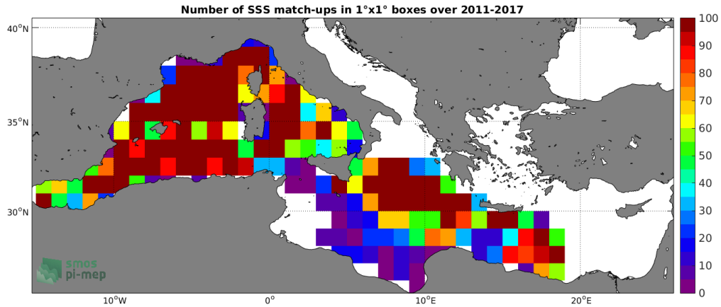
Figure 4: Number of SSS match-ups between Argo SSS and the SMOS-L3-BEC-MED-ATL-OA-V2-9DAYS-0.25DEG SSS product for the Mediterranean Sea Pi-MEP region over 1°x1° boxes and for the full satellite product period.
