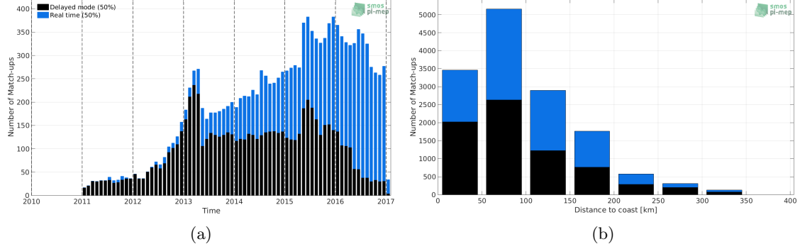
Figure 1: Number of match-ups between Argo and SMOS-L3-BEC-MED-ATL-OA-V2-9DAYS-0.25DEG SSS as a function of time (a) and as function of the distance to coast (b) over the Mediterranean Sea Pi-MEP region and for the full satellite product period.
