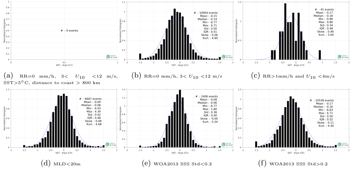
Figure 13: Normalized histogram of \Delta SSS (SMOS-L3-BEC-MED-ATL-OA-V2-9DAYS-0.25DEG - Argo) for 6 different subdatasets corresponding to: RR=0 mm/h, 3 < U_{10} < 12 m/s, SST>5°C, distance to coast > 800 km (a), RR=0 mm/h, 3 < U_{10} < 12 m/s (b), RR>1mm/h and U_{10} < 4 m/s (c), MLD<20m (d), WOA2013 SSS Std<0.2 (e), WOA2013 SSS Std>0.2 (f).
