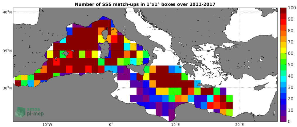
Figure 4: Number of SSS match-ups between Argo SSS and the SMOS-L3-BEC-MED-ATL-OA-V2-9DAYS-0.25DEG SSS product for the Mediterranean Sea Pi-MEP region over 1^\circ \times 1^\circ boxes and for the full satellite product period.
