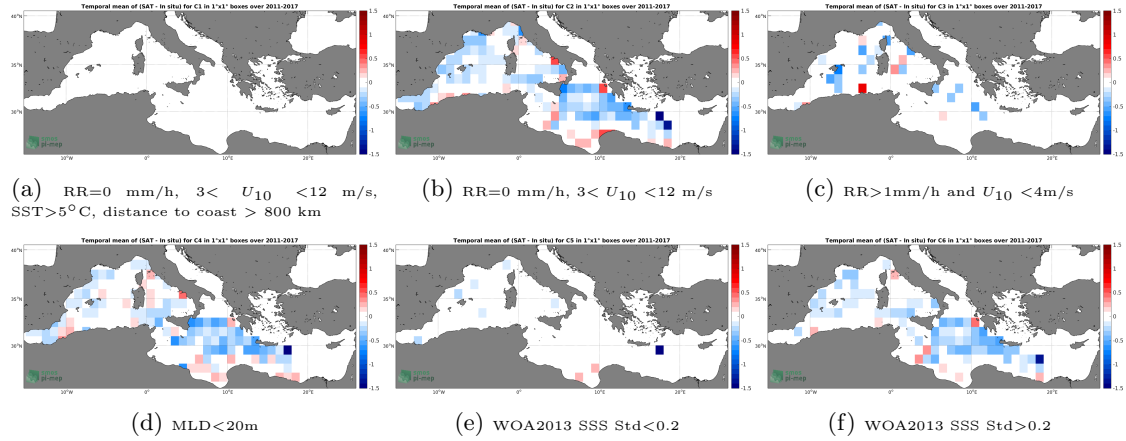
Figure 12: Temporal mean gridded over spatial boxes of size 1^\circ \times 1^\circ of \Delta SSS (SMOS-L3-BEC-MED-ATL-OA-V2-9DAYS-0.25DEG - Argo) for 6 different subdatasets corresponding to: RR=0 mm/h, 3 < U_{10} < 12 m/s, SST > 5^\circ C , distance to coast > 800 km (a), RR=0 mm/h, 3 < U_{10} < 12 m/s (b), RR > 1 mm/h and U_{10} < 4 m/s (c), MLD < 20 m (d), WOA2013 SSS Std < 0.2 (e), WOA2013 SSS Std > 0.2 (f).
