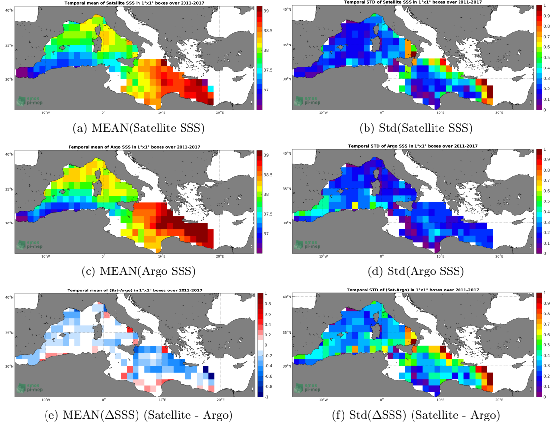
Figure 6: Temporal mean (left) and Std (right) of SSS from SMOS-L3-BEC-MED-ATL-OA-V2-9DAYS-0.25DEG (top), Argo (middle), and of \Delta SSS (Satellite - Argo). Only match-up pairs are used to generate these maps.
