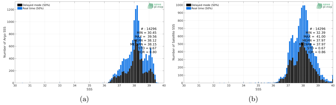
Figure 2: Histograms of SSS from Argo (a) and SMOS-L3-BEC-MED-ATL-OA-V2-9DAYS-0.25DEG (b) considering all match-up pairs per bins of 0.1 over the Mediterranean Sea Pi-MEP region and for the full satellite product period.
