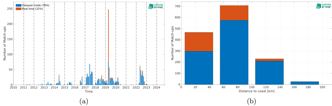
Figure 2: Number of match-ups between Argo and SMOS SSS L2-AVERAGED v700 (ESA) SSS as a function of time (a) and as function of the distance to coast (b) over the Mediterranean Sea Pi-MEP region and for the full satellite product period.
