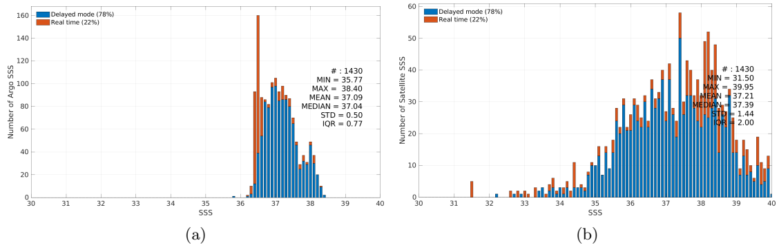
Figure 3: Histograms of SSS from Argo (a) and SMOS SSS L2-AVERAGED v700 (ESA) (b) considering all match-up pairs per bins of 0.1 over the Mediterranean Sea Pi-MEP region and for the full satellite product period.
