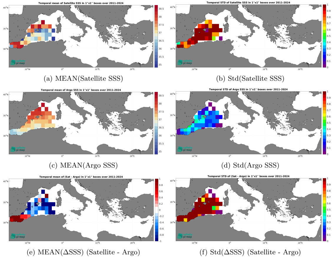
Figure 7: Temporal mean (left) and Std (right) of SSS from SMOS SSS L2-AVERAGED v700 (ESA) (top), Argo (middle), and of \Delta SSS (Satellite - Argo). Only match-up pairs are used to generate these maps.
