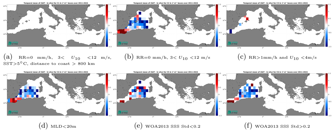
Figure 14: Temporal mean gridded over spatial boxes of size 1^\circ \times 1^\circ of \Delta SSS (SMOS SSS L2-AVERAGED v700 (ESA) - Argo) for 6 different subdatasets corresponding to:RR=0 mm/h, 3 < U_{10} < 12 m/s, SST>5°C, distance to coast > 800 km (a), RR=0 mm/h, 3 < U_{10} < 12 m/s (b), RR>1mm/h and U_{10} < 4 m/s (c),MLD<20m (d),WOA2013 SSS Std<0.2 (e),WOA2013 SSS Std>0.2 (f).
