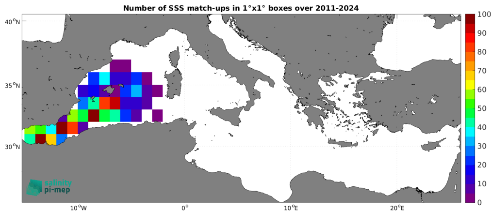
Figure 5: Number of SSS match-ups between Argo SSS and the SMOS SSS L2-AVERAGED v700 (ESA) SSS product for the Mediterranean Sea Pi-MEP region over 1^\circ \times 1^\circ boxes and for the full satellite product period.
