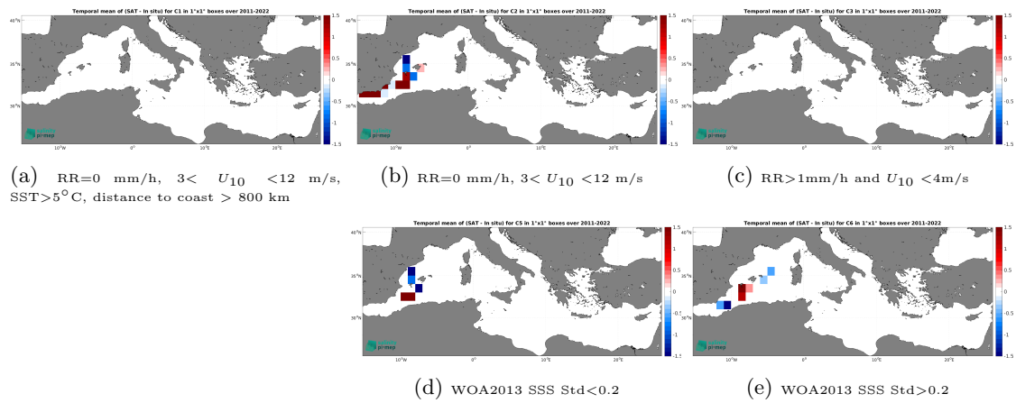
Figure 14: Temporal mean gridded over spatial boxes of size 1^\circ \times 1^\circ of \Delta SSS (SMOS SSS L2 v700 (ESA) - TSG (LEGOS-DM)) for 5 different subdatasets corresponding to:RR=0 mm/h, 3 < U_{10} < 12 m/s, SST>5°C, distance to coast > 800 km (a), RR=0 mm/h, 3 < U_{10} < 12 m/s (b), RR>1mm/h and U_{10} < 4 m/s (c), WOA2013 SSS Std<0.2 (d), WOA2013 SSS Std>0.2 (e).
