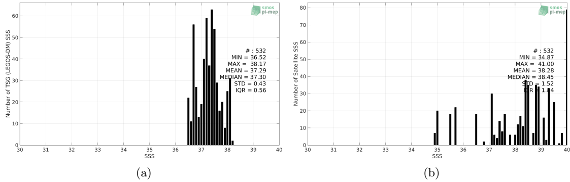
Figure 2: Histograms of SSS from TSG (LEGOS-DM) (a) and SMOS SSS L2 v700 (ESA) (b) considering all match-up pairs per bins of 0.1 over the Mediterranean Sea Pi-MEP region and for the full satellite product period.
