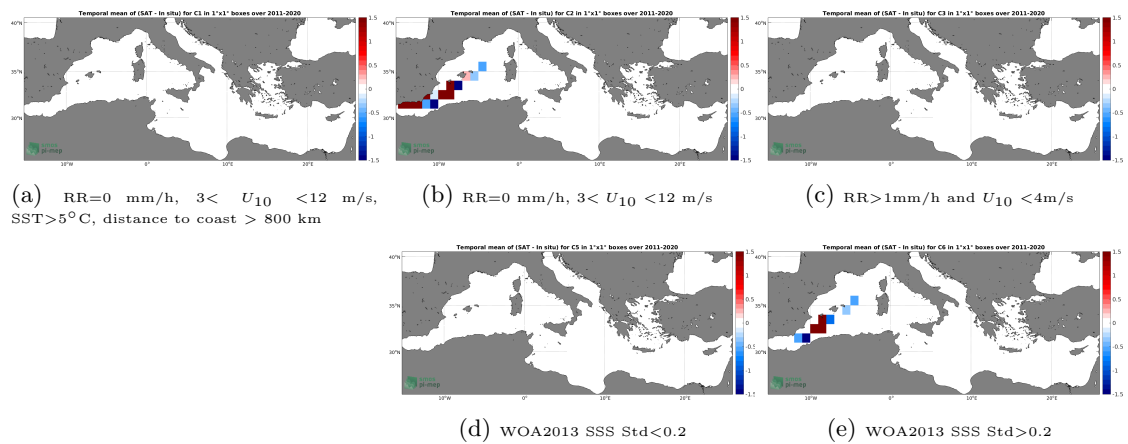
Figure 12: Temporal mean gridded over spatial boxes of size 1^\circ \times 1^\circ of \Delta SSS (SMOS SSS L2 v700 (ESA) - TSG (LEGOS-DM)) for 5 different subdatasets corresponding to:RR=0 mm/h, 3 < U_{10} < 12 m/s, SST >5^\circ\text{C} , distance to coast > 800 km (a), RR=0 mm/h, 3 < U_{10} < 12 m/s (b), RR >1 mm/h and U_{10} < 4 m/s (c), WOA2013 SSS Std <0.2 (d), WOA2013 SSS Std >0.2 (e).
