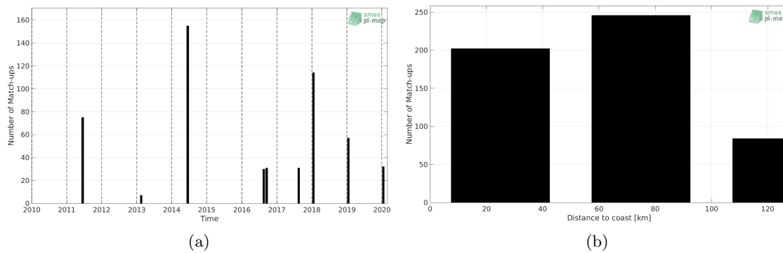
Figure 1: Number of match-ups between TSG (LEGOS-DM) and SMOS SSS L2 v700 (ESA) SSS as a function of time (a) and as function of the distance to coast (b) over the Mediterranean Sea Pi-MEP region and for the full satellite product period.
