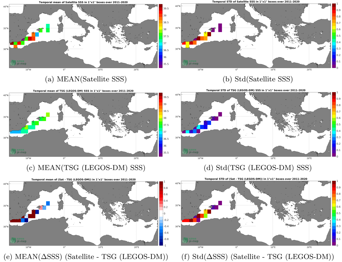
Figure 6: Temporal mean (left) and Std (right) of SSS from SMOS SSS L2 v700 (ESA) (top), TSG (LEGOS-DM) (middle), and of \Delta\text{SSS} (Satellite - TSG (LEGOS-DM)). Only match-up pairs are used to generate these maps.
