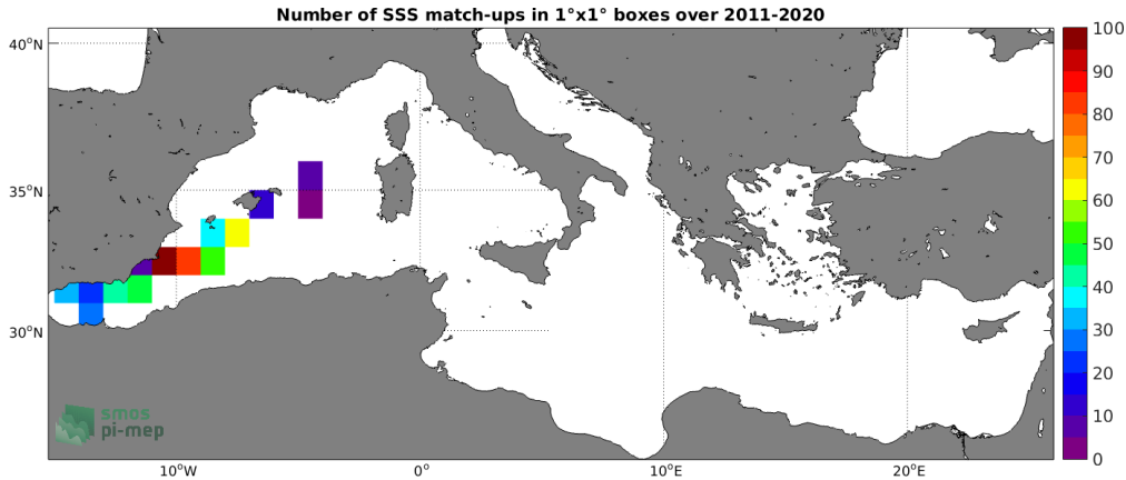
Figure 4: Number of SSS match-ups between TSG (LEGOS-DM) SSS and the SMOS SSS L2 v700 (ESA) SSS product for the Mediterranean Sea Pi-MEP region over 1^\circ \times 1^\circ boxes and for the full satellite product period.
