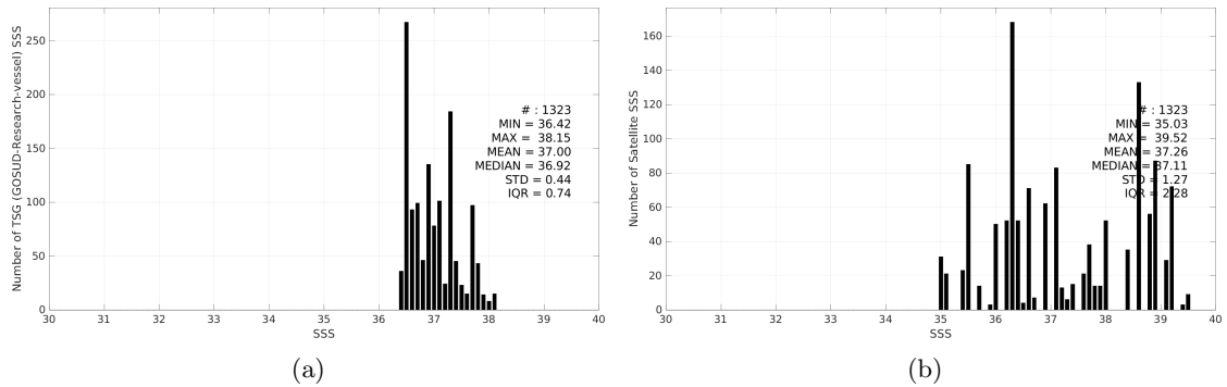
Figure 3: Histograms of SSS from TSG (GOSUD-Research-vessel) (a) and SMOS SSS L2 v700 (ESA) (b) considering all match-up pairs per bins of 0.1 over the Mediterranean Sea Pi-MEP region and for the full satellite product period.
