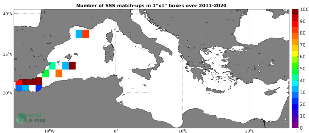
Figure 4: Number of SSS match-ups between TSG (GOSUD-Research-vessel) SSS and the SMOS SSS L2 v700 (ESA) SSS product for the Mediterranean Sea Pi-MEP region over 1^\circ \times 1^\circ boxes and for the full satellite product period.
